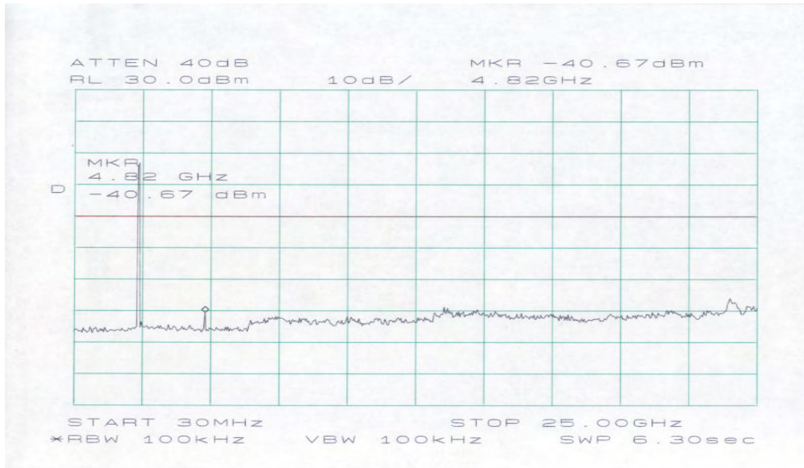
Conducted Spurious Emission for 2410 MHz (Low channel)
