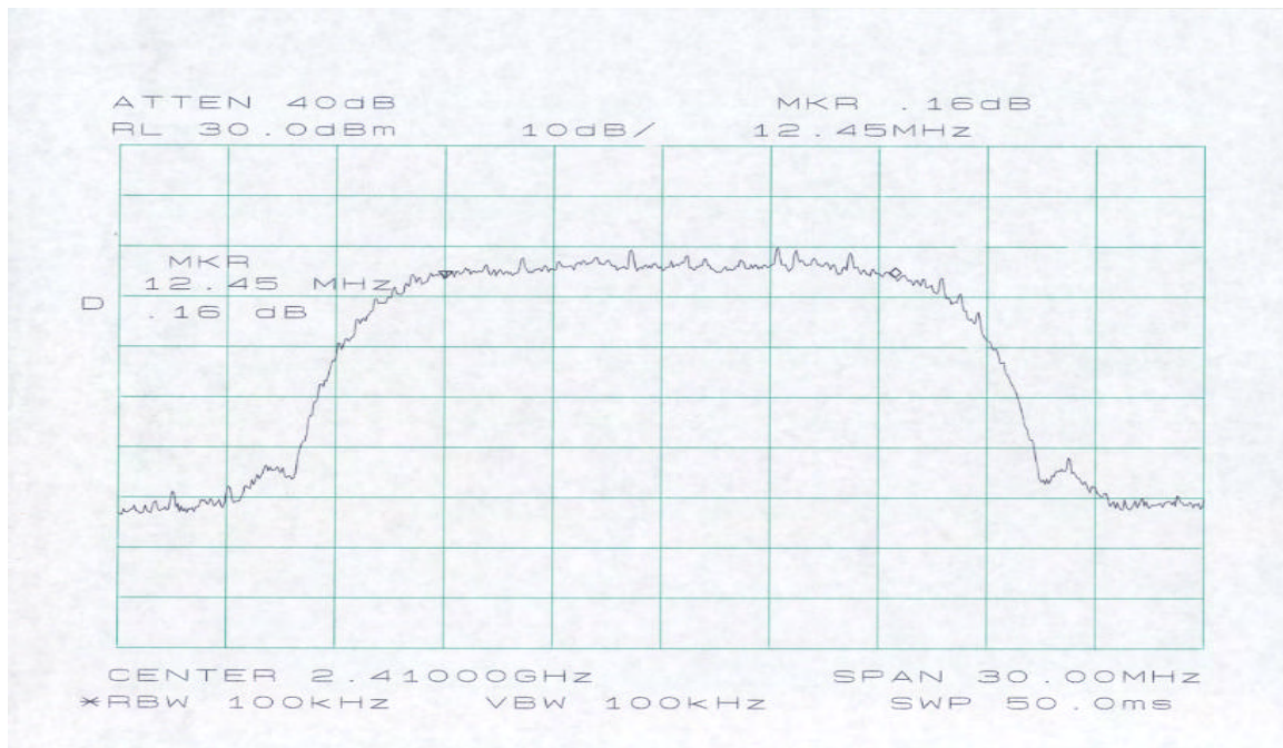
6 dB Bandwidth @ 2410 MHz (Low channel)
