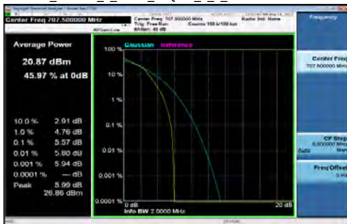
LTE_Band12_1_4MHz_16QAM_6_0_Channel Mid
