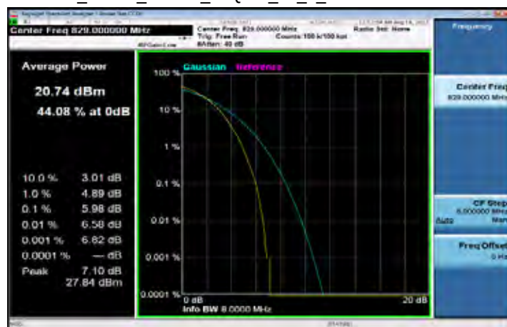
LTE_Band5_10MHz_16QAM_50_0_Channel Low
