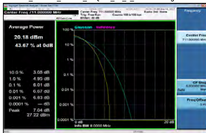
LTE_Band12_10MHz_16QAM_50_0_Channel High
