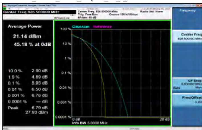
LTE_Band5_5MHz_16QAM_25_0_Channel Low
