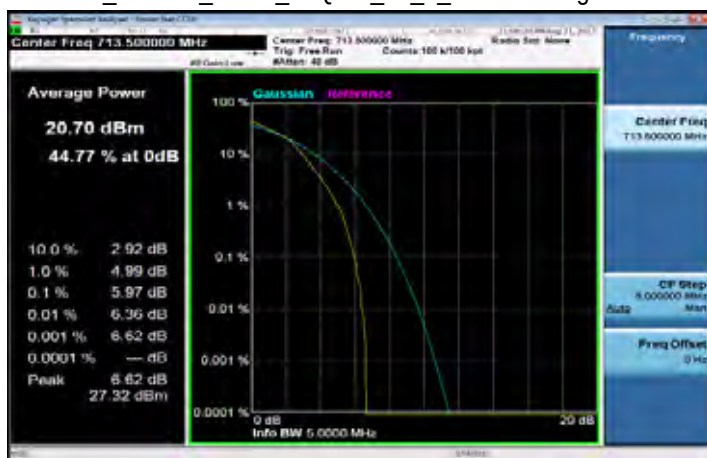
LTE_Band12_5MHz_16QAM_25_0_Channel High
