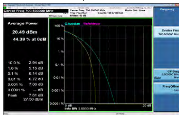
LTE_Band12_3MHz_16QAM_15_0_Channel Low
