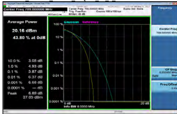
LTE_Band17_10MHz_16QAM_50_0_Channel Low
