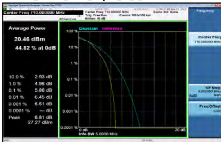
LTE_Band17_5MHz_16QAM_25_0_Channel Mid
