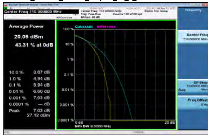
LTE_Band17_10MHz_16QAM_50_0_Channel Mid
