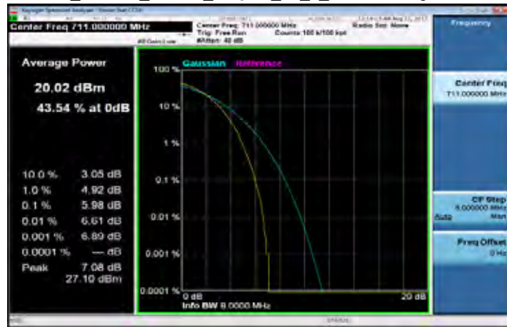
LTE_Band17_10MHz_16QAM_50_0_Channel High
