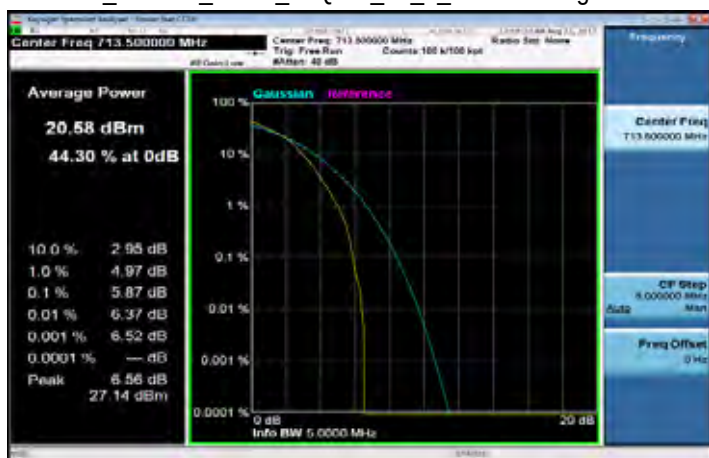
LTE_Band17_5MHz_16QAM_25_0_Channel High
