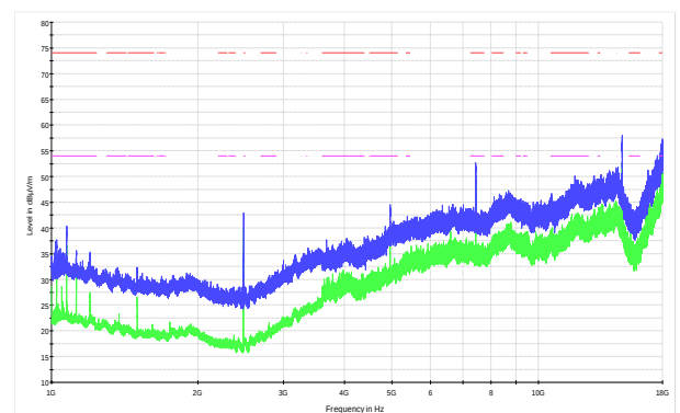
Figure 8.7-25: Radiated spurious emissions within 1–18 GHz for EDR2 modulation Mid channel
