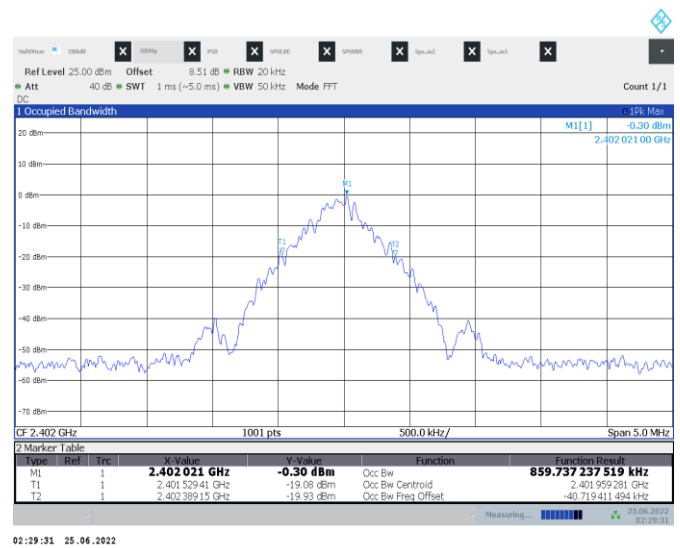
Figure 8.5-2: 99% occupied bandwidth sample plot
