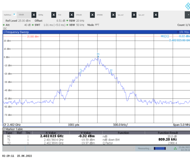
Figure 8.5-1: 20 dB bandwidth sample plot
