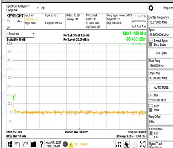
Band5_10MHz_QPSK_20525_50RB#0_0.15~30_0.15~30
