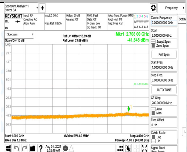
Band5_5MHz_16QAM_20625_1RB#24_1000~3000_1000~3000
