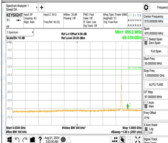
Band5_5MHz_16QAM_20625_1RB#24_3000~10000_3000~1000
