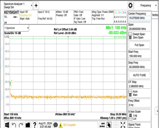
Band5_10MHz_QPSK_20450_50RB#0_1000~3000_1000~3000
