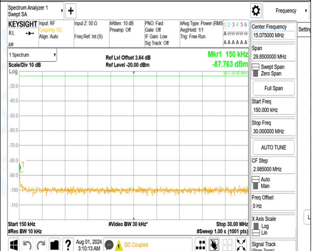
Band5_10MHz_QPSK_20600_50RB#0_1000~3000_1000~3000
