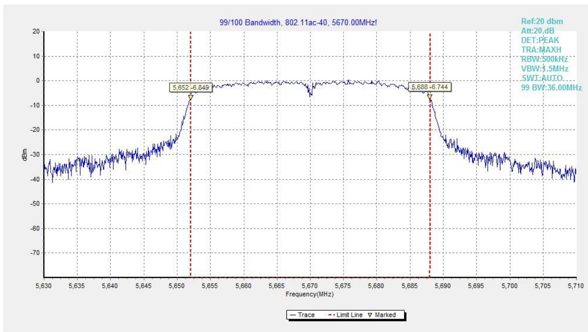
Fig. 42 99% Occupied Bandwidth (802.11ac-VHT40, 5670MHz)
