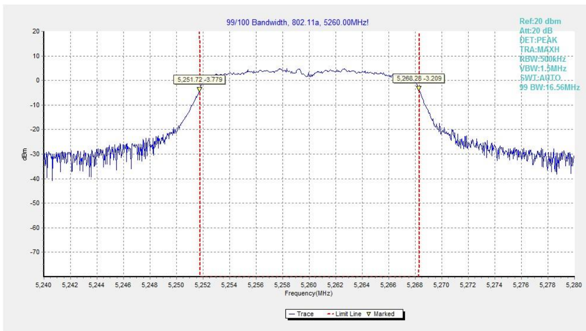
Fig. 28 99% Occupied Bandwidth (802.11a, 5260MHz)
