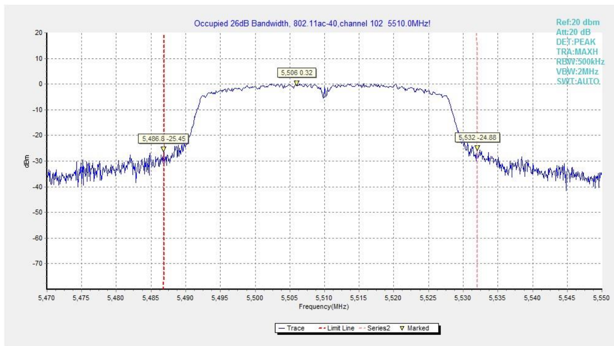
Fig. 14 Occupied 26dB Bandwidth (802.11ac-VHT40, 5510MHz)
