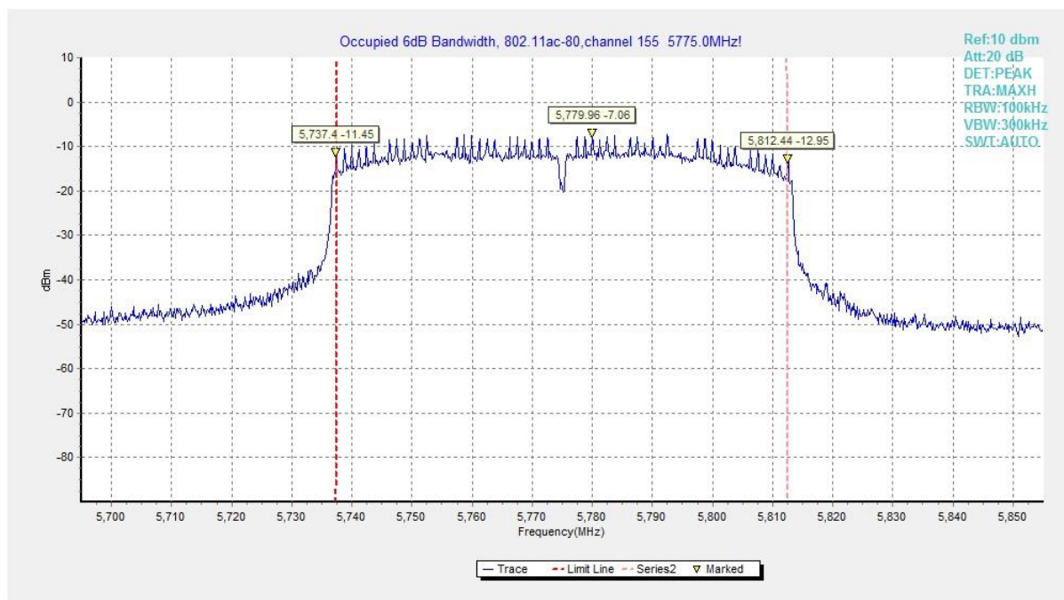
Fig. 24 Occupied 6dB Bandwidth (802.11ac-VHT80, 5775MHz)
