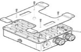
Figure 3 Attaching the "H" Bracket to the AP
