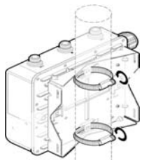
Figure 6 AP with Mounting Bracket—Vertical Pole
