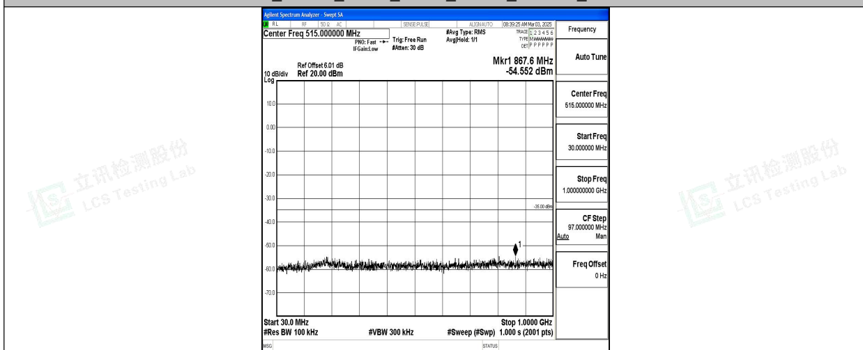
Band7_15MHz_QPSK_20825_1RB#0_30~1000_30~1000
