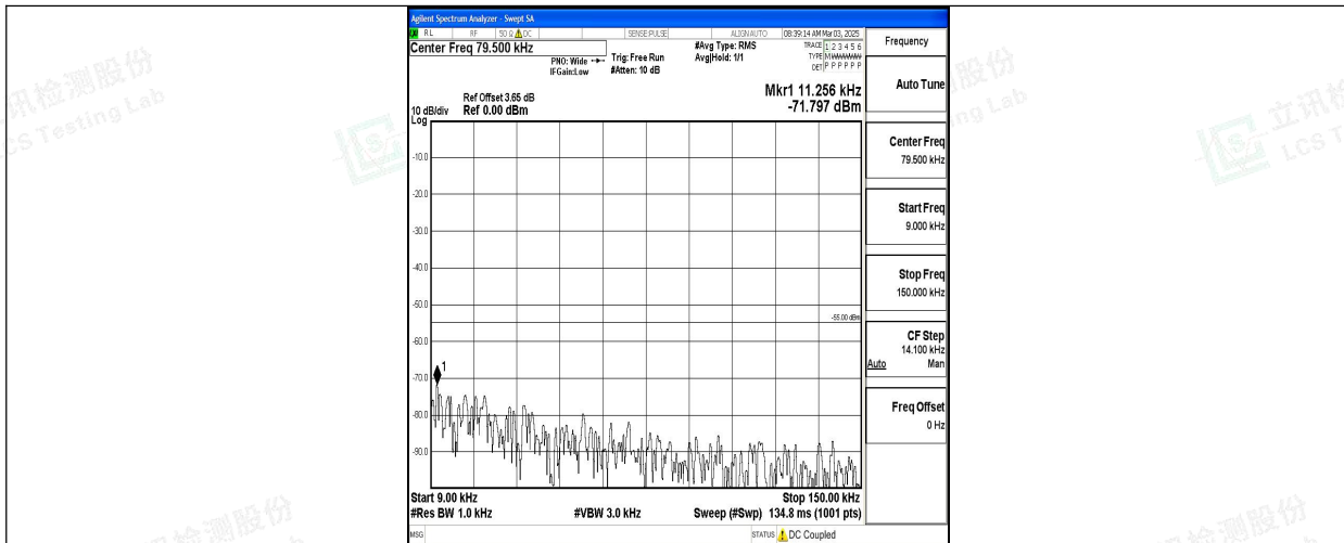
Band7_15MHz_QPSK_20825_1RB#0_0.009~0.15_0.009~0.15
