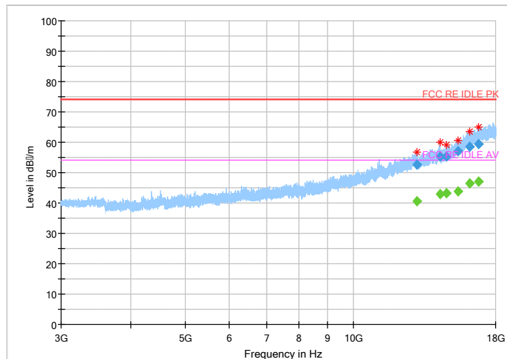
Fig.26 Radiated emission: Ch39, 3GHz~18GHz
