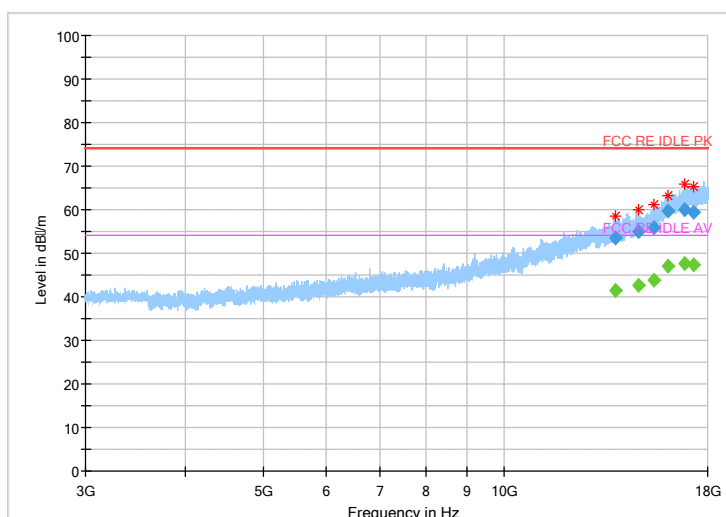
Fig.20 Radiated emission: Ch0, 3GHz~18GHz
