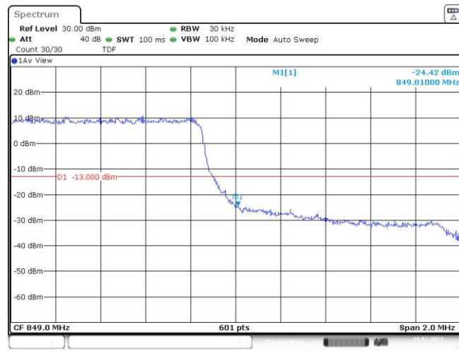
Band26-1.4MHz-QPSK-27033-6RB#0
