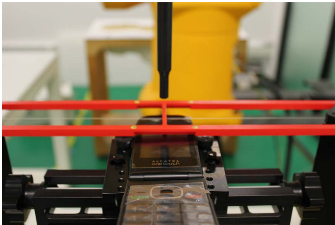
Picture 3: EUT Positioning for RF
