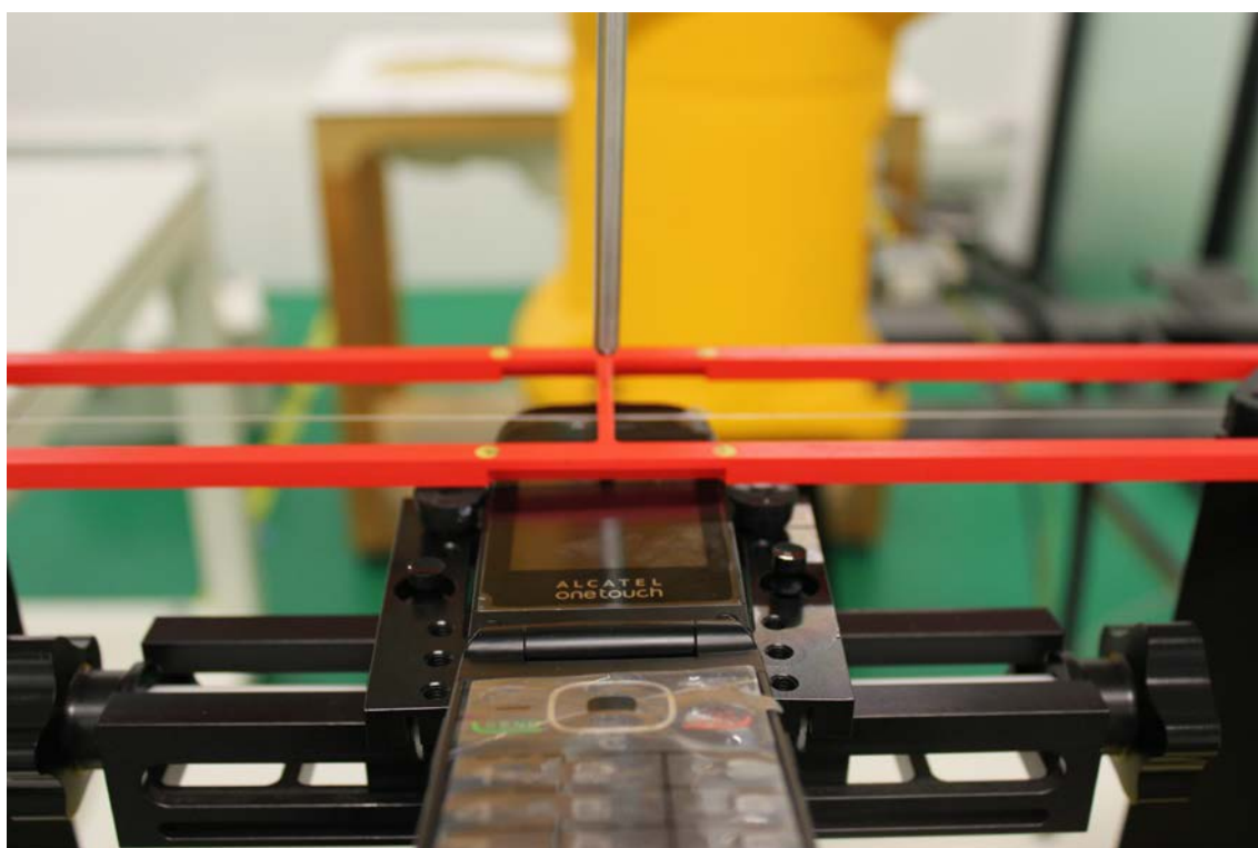
Picture 4: EUT Positioning for T-coil
