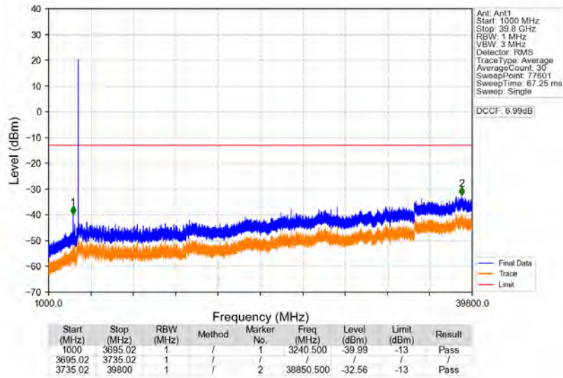
n77a_30kHz_SISO_NTNV_30MHz_DFT-s-OFDM_PI/2_BPSK_3715.02MHz_Edge_1RB_Left
