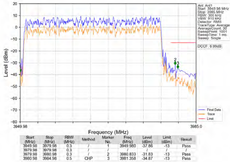
n77a_30kHz_SISO_NTNV_30MHz_DFT-s-OFDM_PI/2_BPSK_3964.98MHz_Outer_Full
