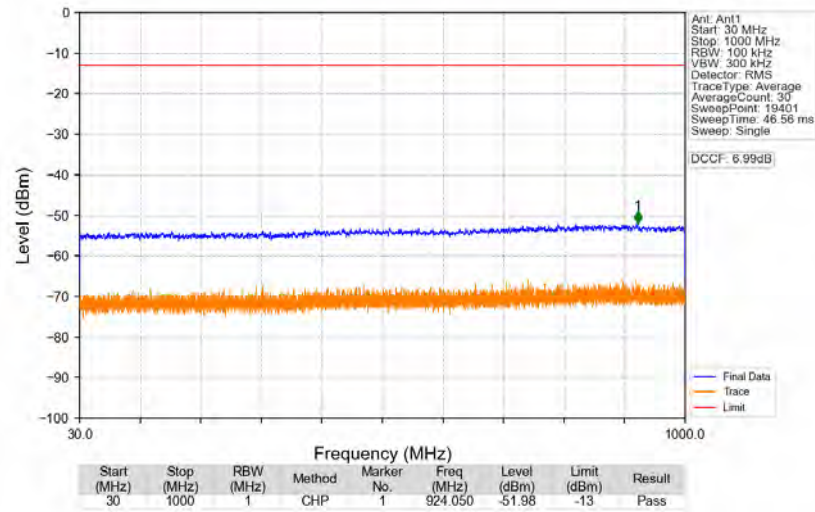
n77a_30kHz_SISO_NTNV_40MHz_DFT-s-OFDM_PI/2_BPSK_3840MHz_Edge_1RB_Left
