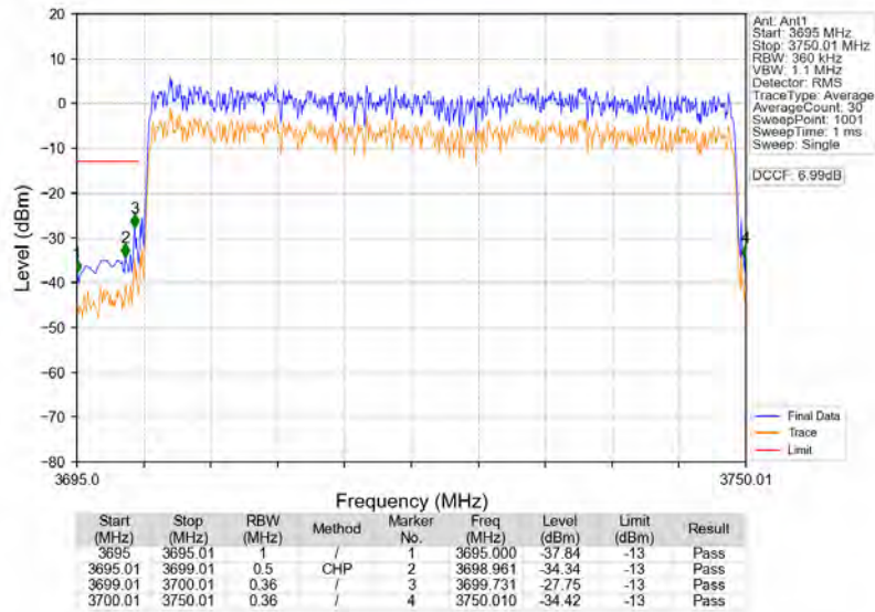
n77a_30kHz_SISO_NTNV_50MHz_CP-OFDM_QPSK_3725.01MHz_Outer_Full
