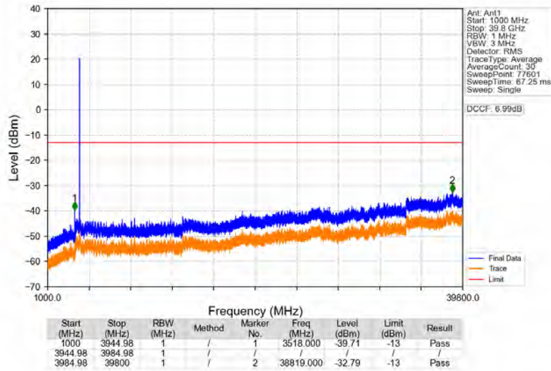
n77a_30kHz_SISO_NTNV_30MHz_DFT-s-OFDM_PI/2_BPSK_3964.98MHz_Edge_1RB_Right
