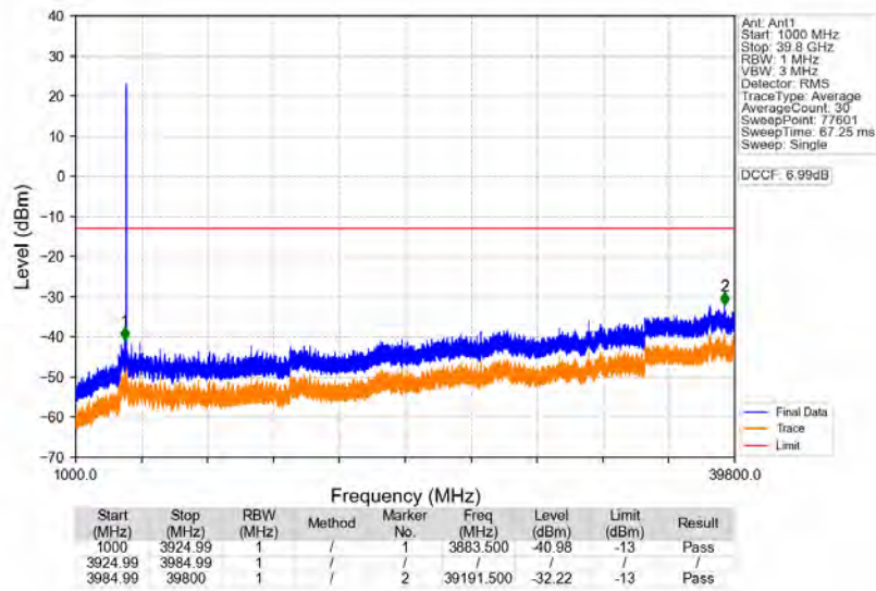
n77a_30kHz_SISO_NTNV_50MHz_DFT-s-OFDM_QPSK_3954.99MHz_Edge_1RB_Right
