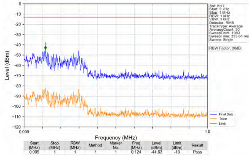
n77a_30kHz_SISO_NTNV_50MHz_DFT-s-OFDM_PI/2_BPSK_3840MHz_Edge_1RB_Left
