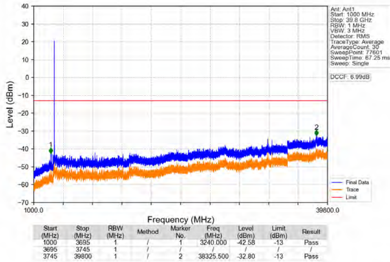
n77a_30kHz_SISO_NTNV_40MHz_DFT-s-OFDM_QPSK_3720MHz_Edge_1RB_Left
