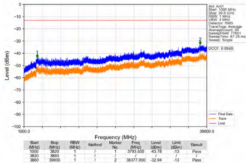
n77a_30kHz_SISO_NTNV_30MHz_DFT-s-OFDM_PI/2_BPSK_3840MHz_Edge_1RB_Left
