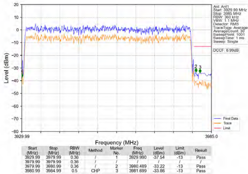
n77a 30kHz SISO NTN 50MHz CP-OFDM QPSK 3954.99MHz Outer_Full
