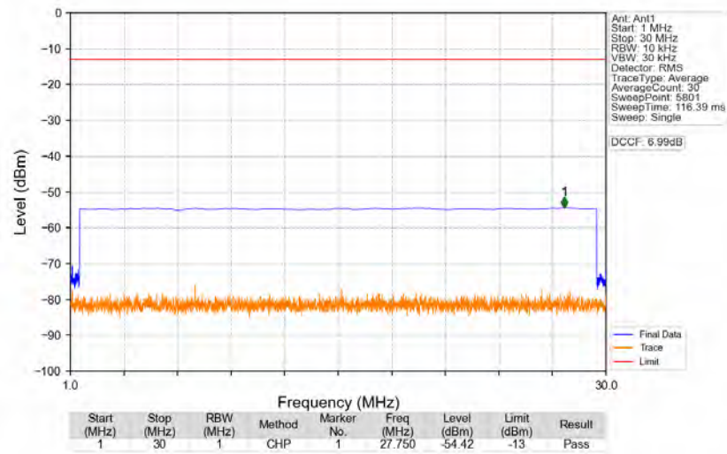
n77a_30kHz_SISO_NTNV_40MHz_CP-OFDM_QPSK_3720MHz_Edge_1RB_Left
