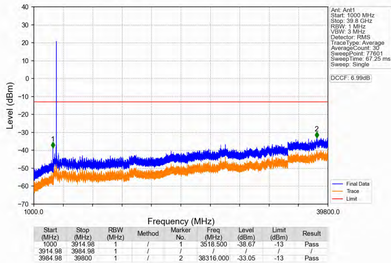
n77a_30kHz_SISO_NTNV_60MHz_DFT-s-OFDM_PI/2_BPSK_3949.98MHz_Edge_1RB_Right
