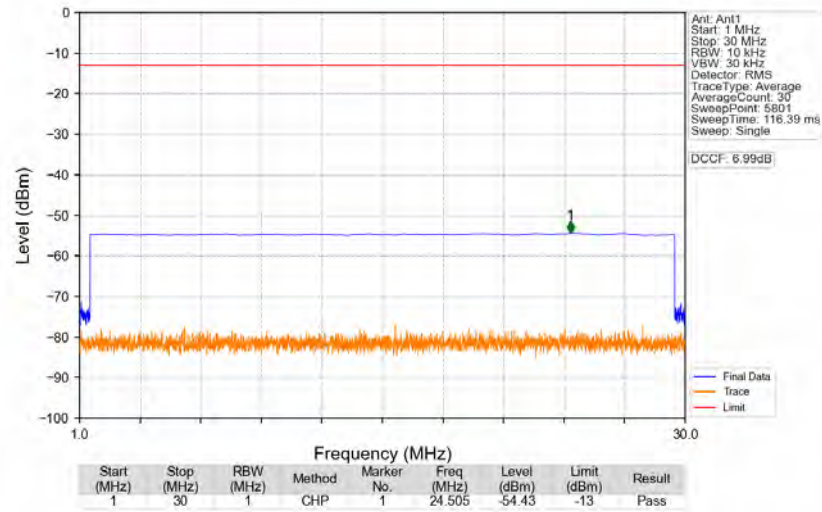
n77a_30kHz_SISO_NTNV_70MHz_DFT-s-OFDM_PI/2_BPSK_3840MHz_Edge_1RB_Left
