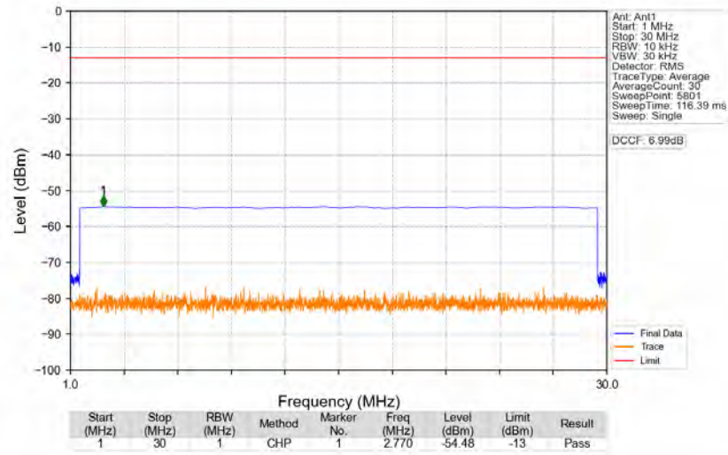
n77a_30kHz_SISO_NTNV_40MHz_DFT-s-OFDM_QPSK_3720MHz_Edge_1RB_Left
