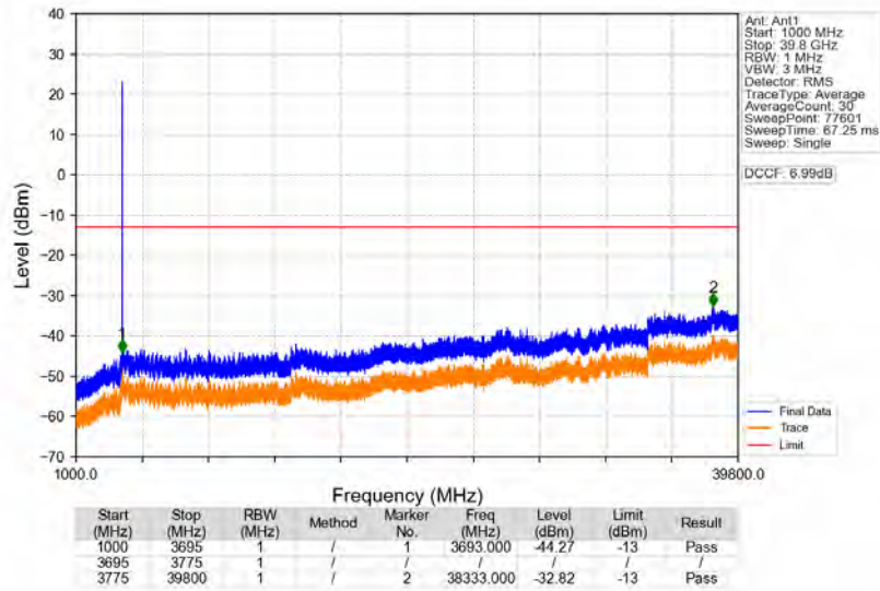
n77a_30kHz_SISO_NTNV_70MHz_DFT-s-OFDM_QPSK_3735MHz_Edge_1RB_Left
