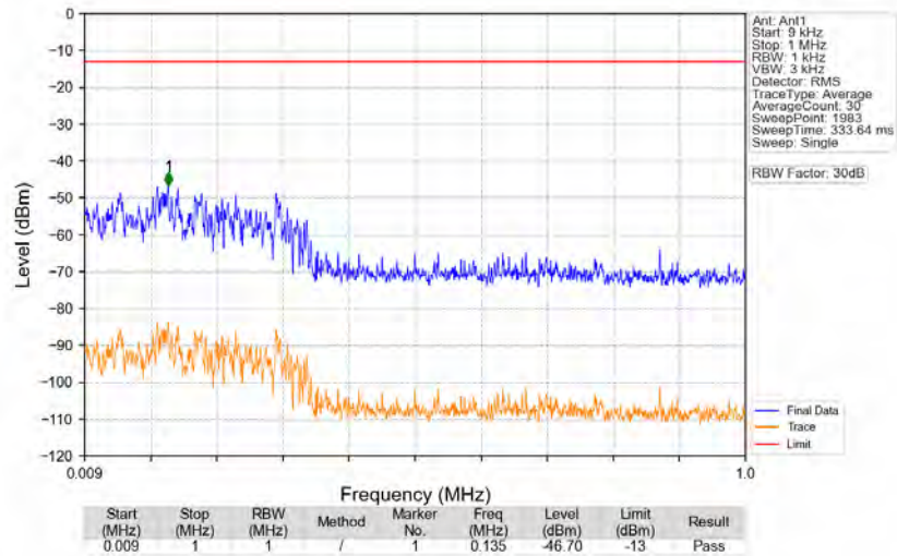
n77a_30kHz_SISO_NTNV_60MHz_DFT-s-OFDM_QPSK_3949.98MHz_Edge_1RB_Right
