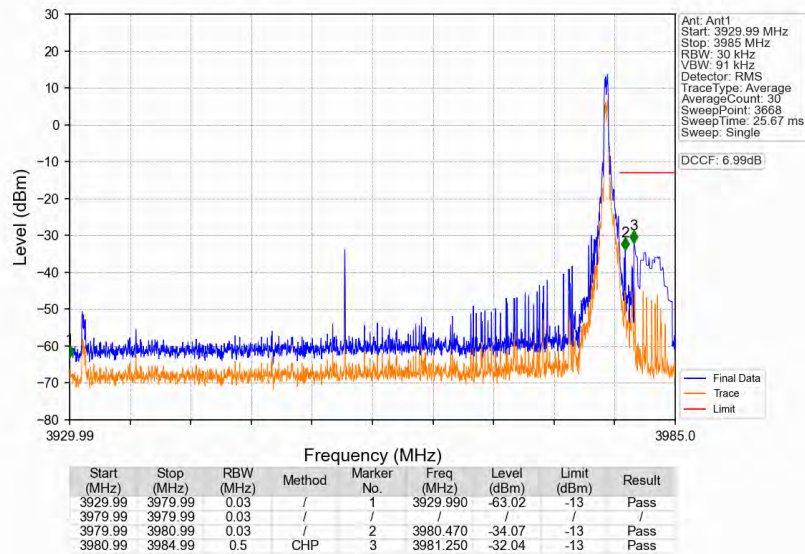
n77a_30kHz_SISO_NTNV_50MHz_DFT-s-OFDM_QPSK_3954.99MHz_Edge_1RB_Right
