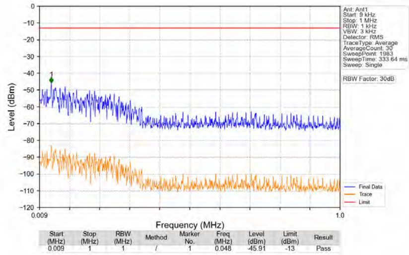
n77a_30kHz_SISO_NTNV_50MHz_CP-OFDM_QPSK_3840MHz_Edge_1RB_Left
