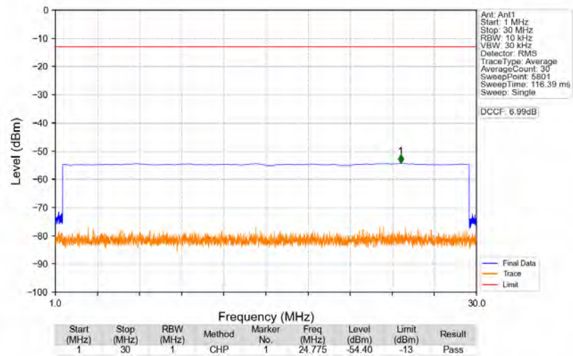
n77a_30kHz_SISO_NTNV_30MHz_CP-OFDM_QPSK_3840MHz_Edge_1RB_Left
