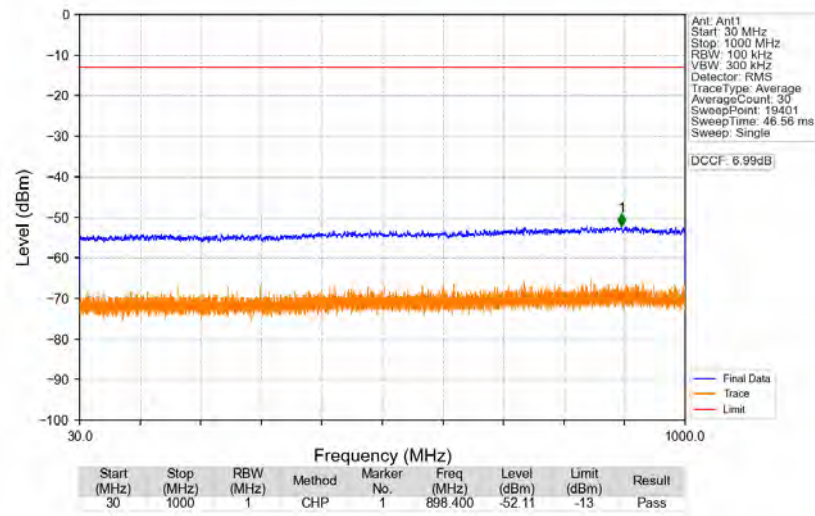
n77a_30kHz_SISO_NTNV_50MHz_CP-OFDM_QPSK_3840MHz_Edge_1RB_Left
