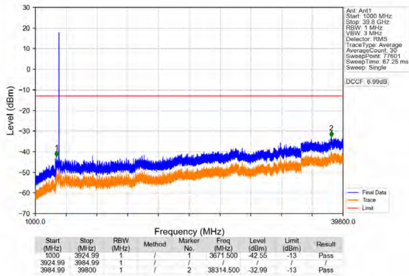
n77a_30kHz_SISO_NTNV_50MHz_DFT-s-OFDM_PI/2_BPSK_3954.99MHz_Edge_1RB_Right
