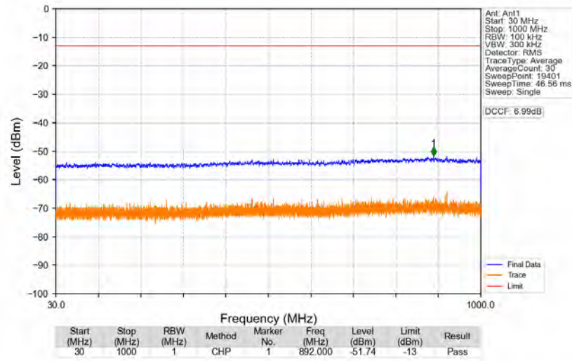
n77a_30kHz_SISO_NTNV_40MHz_CP-OFDM_QPSK_3840MHz_Edge_1RB_Left
