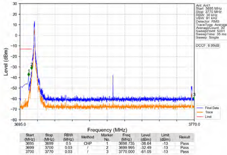
n77a_30kHz_SISO_NTNV_70MHz_DFT-s-OFDM_QPSK_3735MHz_Edge_1RB_Left
