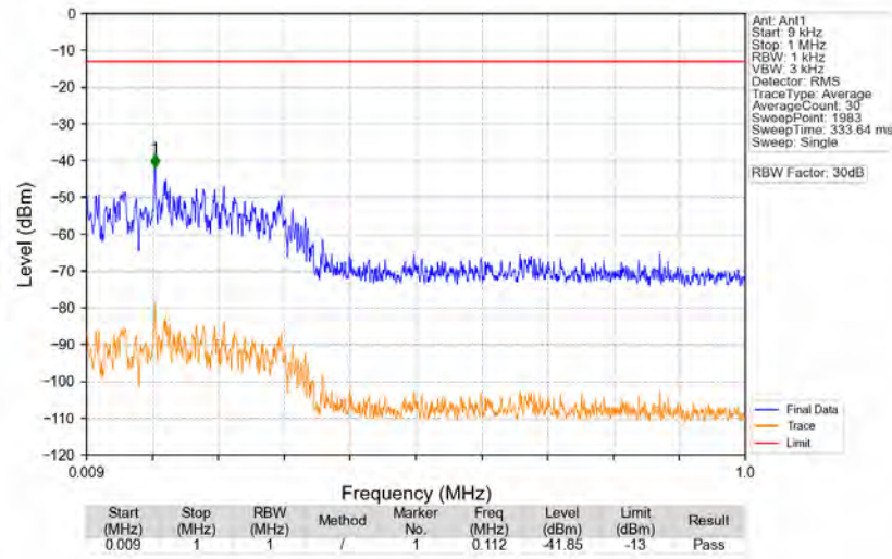
n77a_30kHz_SISO_NTNV_70MHz_DFT-s-OFDM_QPSK_3840MHz_Edge_1RB_Left
