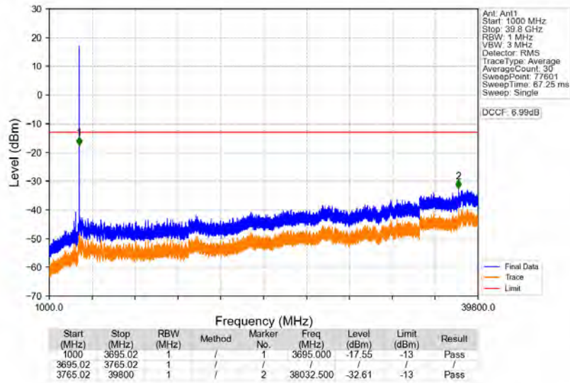
n77a_30kHz_SISO_NTNV_60MHz_CP-OFDM_QPSK_3730.02MHz_Edge_1RB_Left
