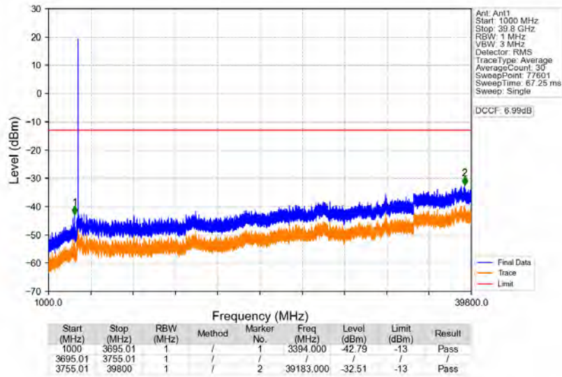
n77a_30kHz_SISO_NTNV_50MHz_CP-OFDM_QPSK_3725.01MHz_Edge_1RB_Left
