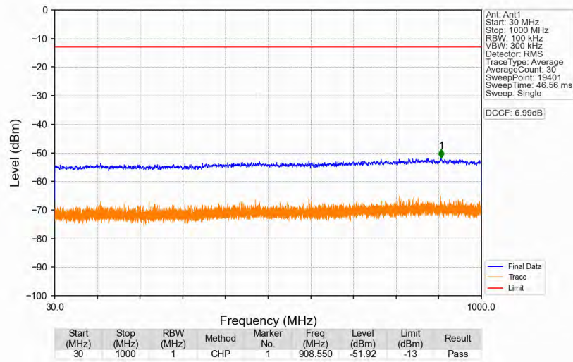
n77a_30kHz_SISO_NTNV_30MHz_DFT-s-OFDM_QPSK_3840MHz_Edge_1RB_Left
