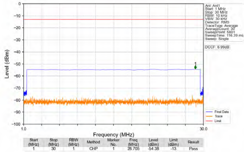
n77a_30kHz_SISO_NTNV_30MHz_DFT-s-OFDM_PI/2_BPSK_3840MHz_Edge_1RB_Left
