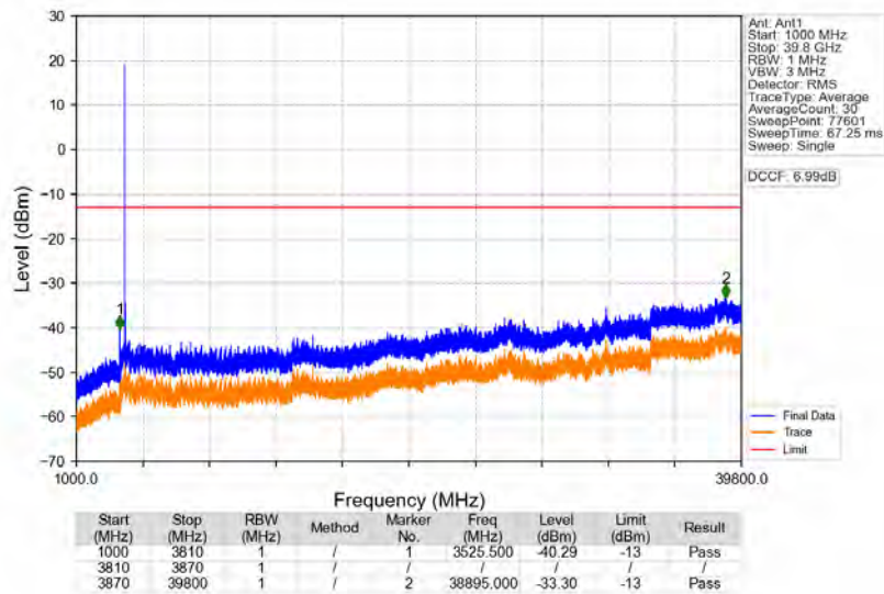
n77a_30kHz_SISO_NTNV_50MHz_DFT-s-OFDM_QPSK_3840MHz_Edge_1RB_Left
