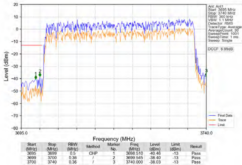
n77a 30kHz SISO NTN 40MHz DFT-s-OFDM PI/2 BPSK 3720MHz Outer Full
