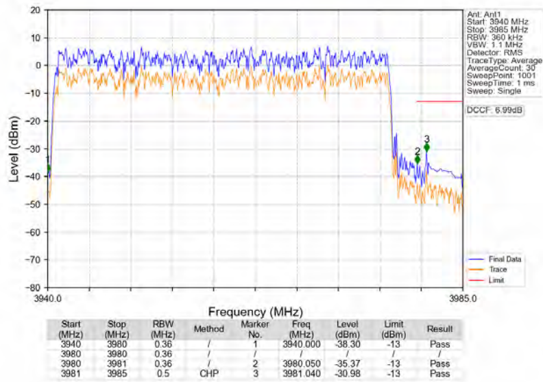
n77a 30kHz SISO NTN 40MHz DFT-s-OFDM QPSK 3960MHz Outer Full
