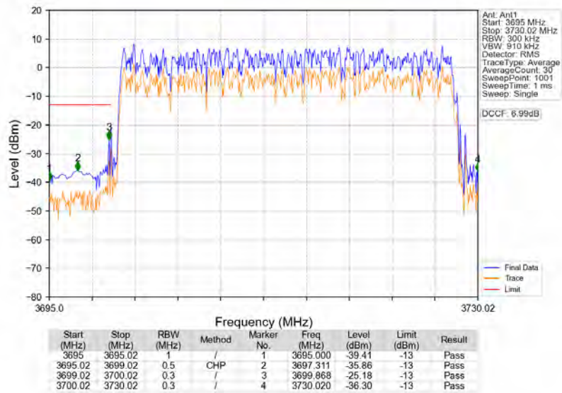
n77a_30kHz_SISO_NTNV_30MHz_DFT-s-OFDM_QPSK_3715.02MHz_Outer_Full
