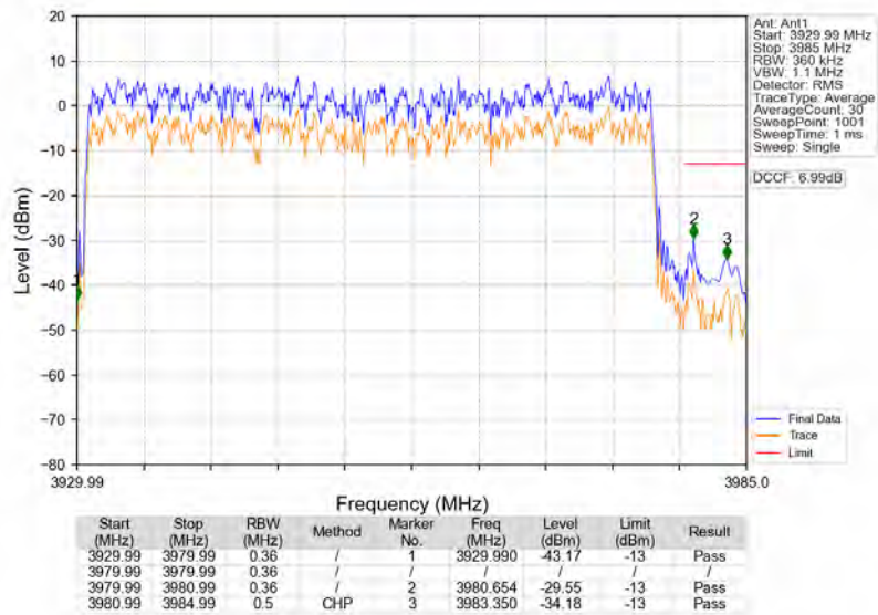
n77a_30kHz_SISO_NTNV_50MHz_DFT-s-OFDM_PI/2_BPSK_3954.99MHz_Outer_Full
