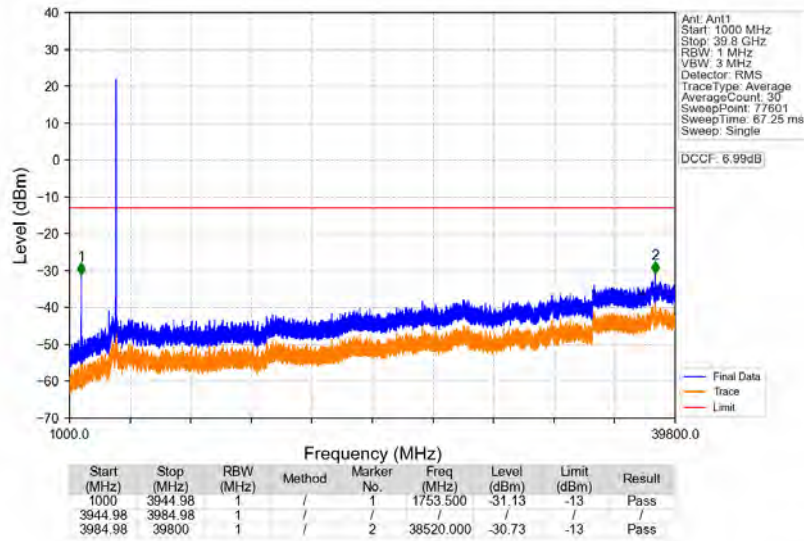
n77a 30kHz SISO NTN 30MHz CP-OFDM QPSK 3964.98MHz Edge_1RB_Right
