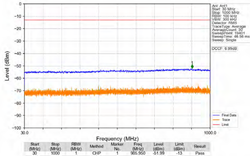
n77a_30kHz_SISO_NTNV_50MHz_CP-OFDM_QPSK_3725.01MHz_Edge_1RB_Left
