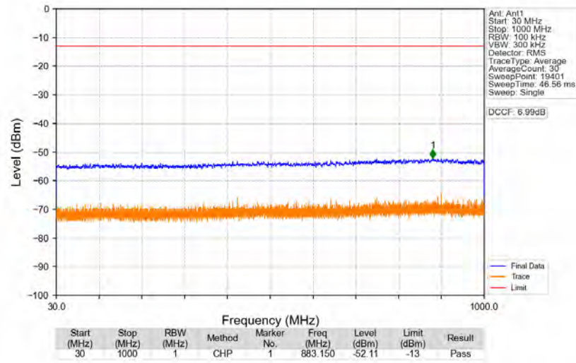
n77a_30kHz_SISO_NTNV_30MHz_CP-OFDM_QPSK_3840MHz_Edge_1RB_Left
