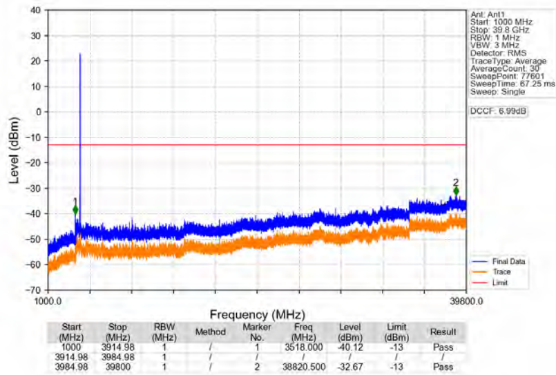
n77a_30kHz_SISO_NTNV_60MHz_DFT-s-OFDM_QPSK_3949.98MHz_Edge_1RB_Right
