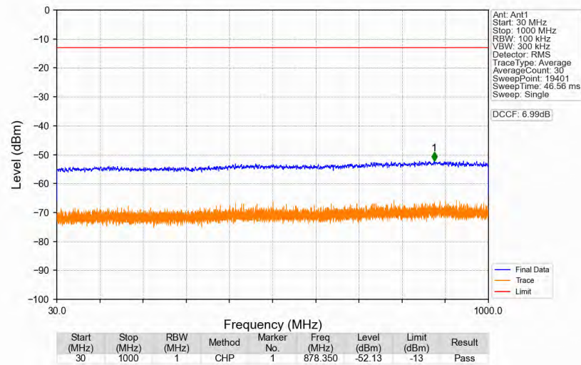
n77a_30kHz_SISO_NTNV_70MHz_DFT-s-OFDM_PI/2_BPSK_3945MHz_Edge_1RB_Right
