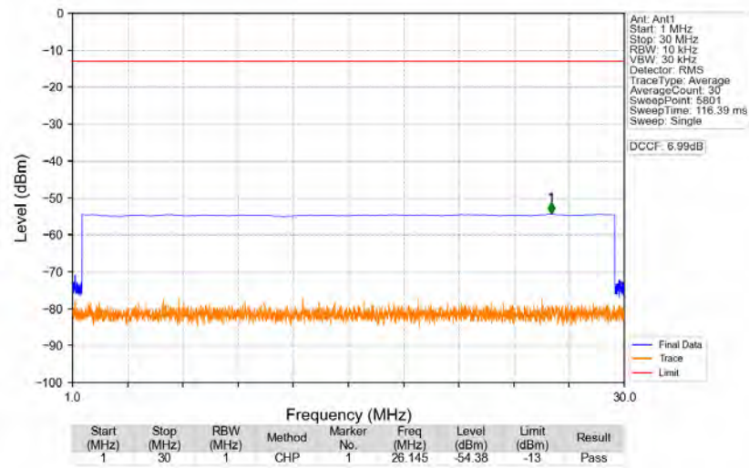
n77a_30kHz_SISO_NTNV_40MHz_DFT-s-OFDM_PI/2_BPSK_3720MHz_Edge_1RB_Left
