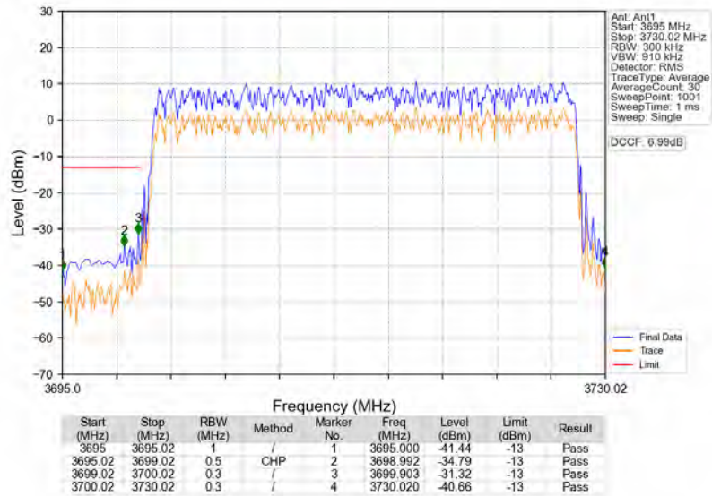
n77a_30kHz_SISO_NTNV_30MHz_DFT-s-OFDM_PI/2_BPSK_3715.02MHz_Outer_Full
