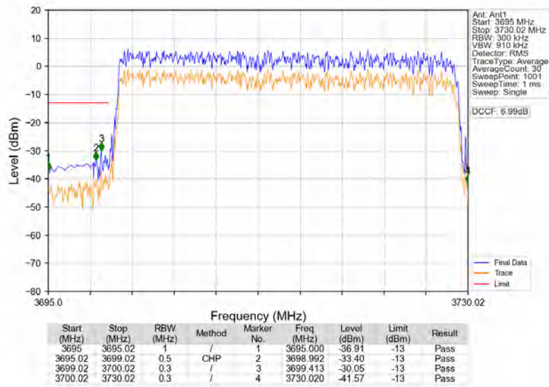
n77a_30kHz_SISO_NTNV_30MHz_CP-OFDM_QPSK_3715.02MHz_Outer_Full
