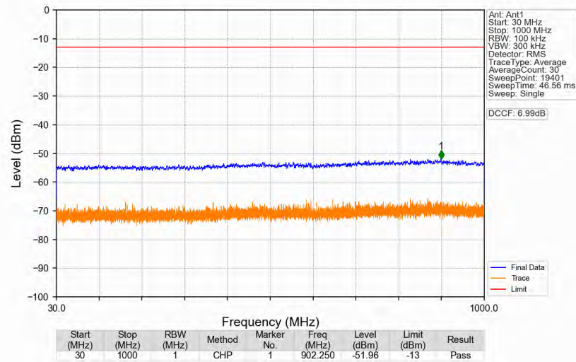
n77a_30kHz_SISO_NTNV_40MHz_DFT-s-OFDM_PI/2_BPSK_3960MHz_Edge_1RB_Right
