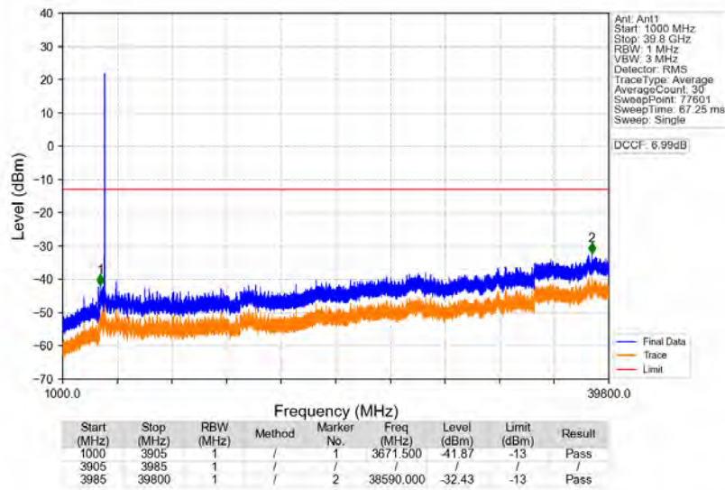
n77a_30kHz_SISO_NTNV_70MHz_DFT-s-OFDM_PI/2_BPSK_3945MHz_Edge_1RB_Right
