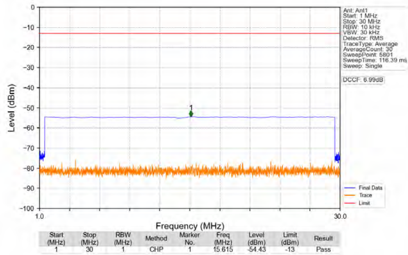
n77a_30kHz_SISO_NTNV_40MHz_DFT-s-OFDM_PI/2_BPSK_3960MHz_Edge_1RB_Right
