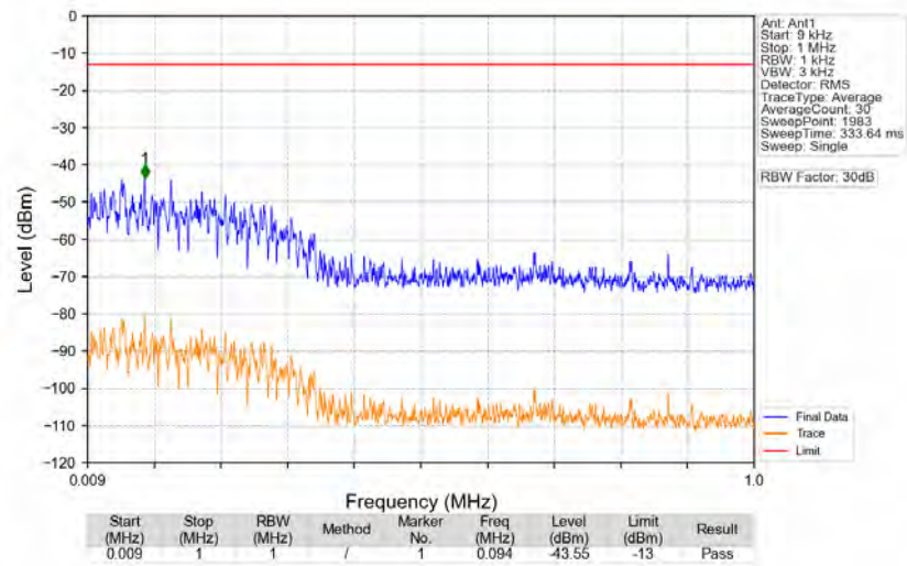
n77a_30kHz_SISO_NTNV_30MHz_CP-OFDM_QPSK_3840MHz_Edge_1RB_Left
