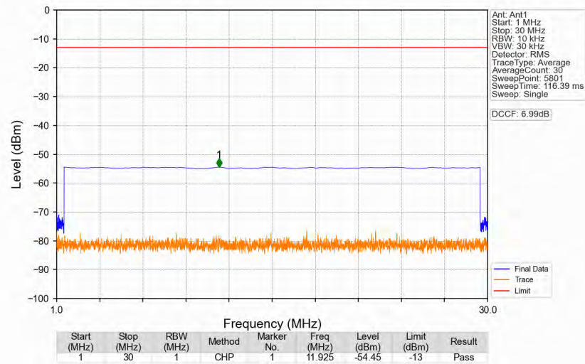
n77a_30kHz_SISO_NTNV_70MHz_DFT-s-OFDM_PI/2_BPSK_3945MHz_Edge_1RB_Right
