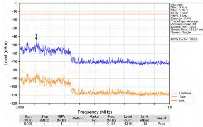
n77a_30kHz_SISO_NTNV_60MHz_DFT-s-OFDM_PI/2_BPSK_3840MHz_Edge_1RB_Left
