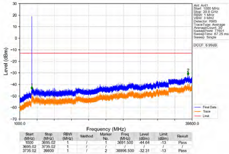
n77a_30kHz_SISO_NTNV_30MHz_DFT-s-OFDM_QPSK_3715.02MHz_Edge_1RB_Left
