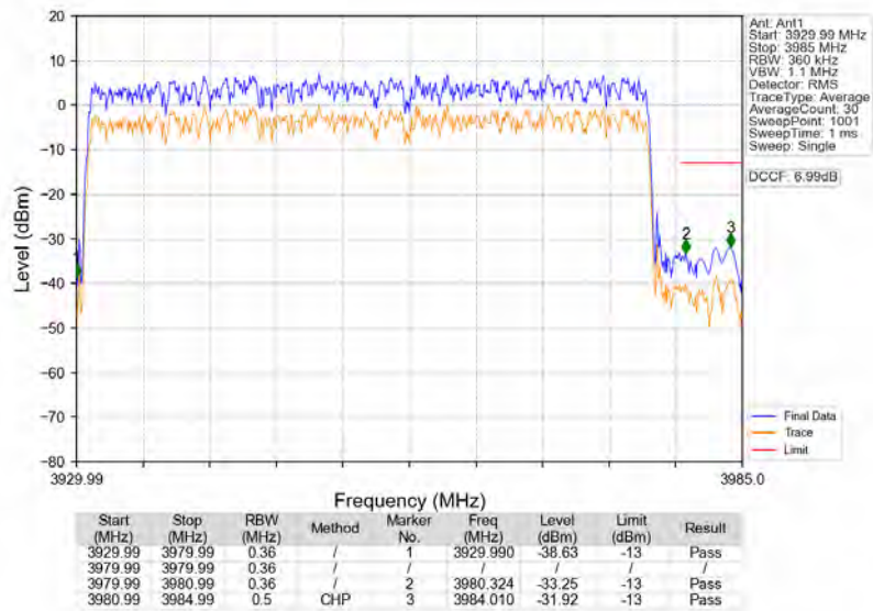
n77a_30kHz_SISO_NTNV_50MHz_DFT-s-OFDM_QPSK_3954.99MHz_Outer_Full
