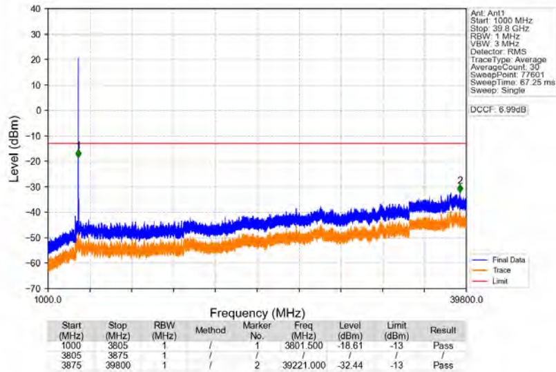
n77a_30kHz_SISO_NTNV_60MHz_DFT-s-OFDM_PI/2_BPSK_3840MHz_Edge_1RB_Left
