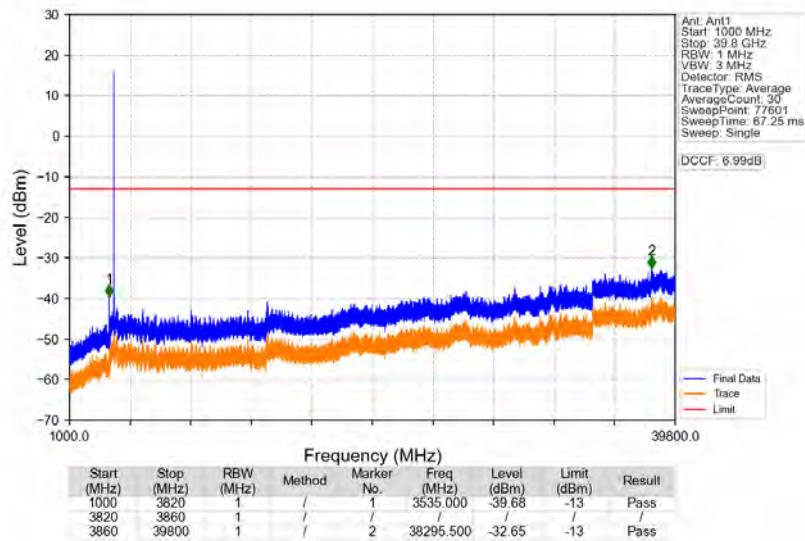
n77a_30kHz_SISO_NTNV_30MHz_DFT-s-OFDM_QPSK_3840MHz_Edge_1RB_Left
