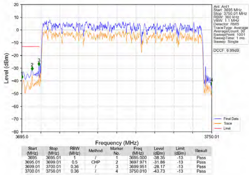
n77a_30kHz_SISO_NTNV_50MHz_DFT-s-OFDM_QPSK_3725.01MHz_Outer_Full
