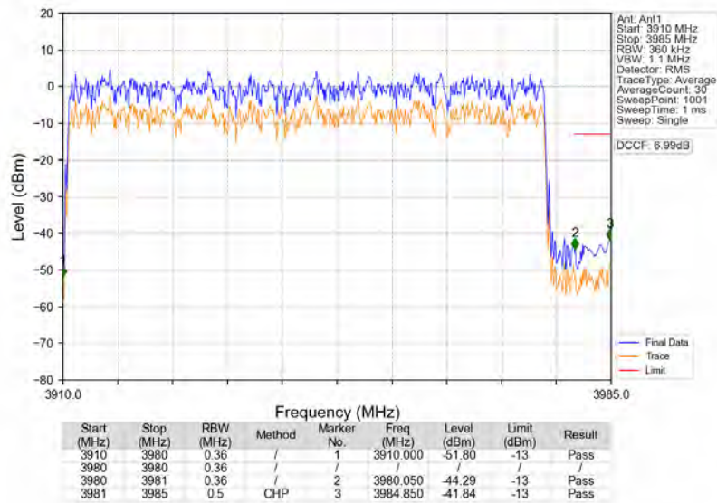
n77a_30kHz_SISO_NTNV_70MHz_DFT-s-OFDM_PI/2_BPSK_3945MHz_Outer_Full
