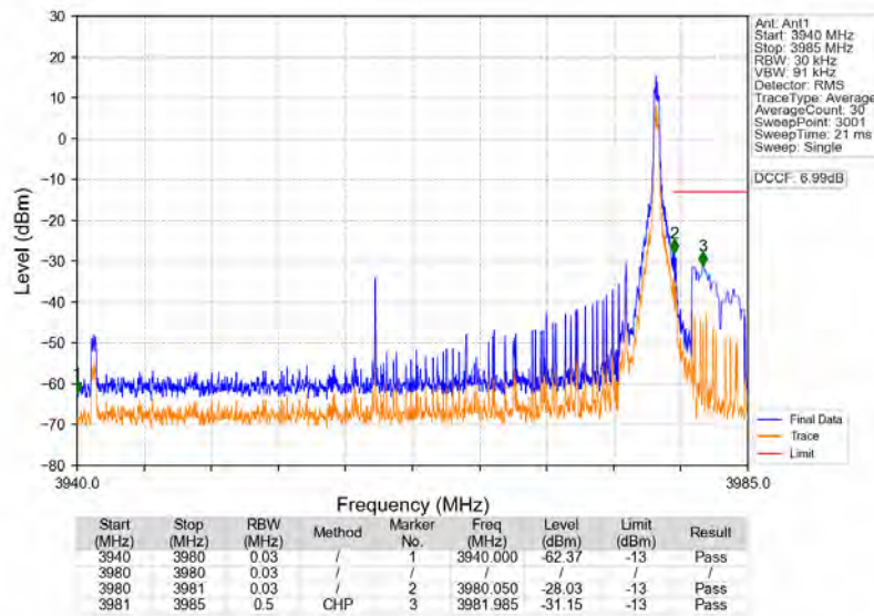
n77a_30kHz_SISO_NTNV_40MHz_DFT-s-OFDM_PI/2_BPSK_3960MHz_Edge_1RB_Right
