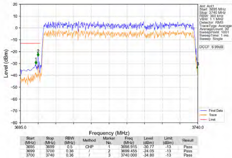
n77a_30kHz_SISO_NTNV_40MHz_CP-OFDM_QPSK_3720MHz_Outer_Full
