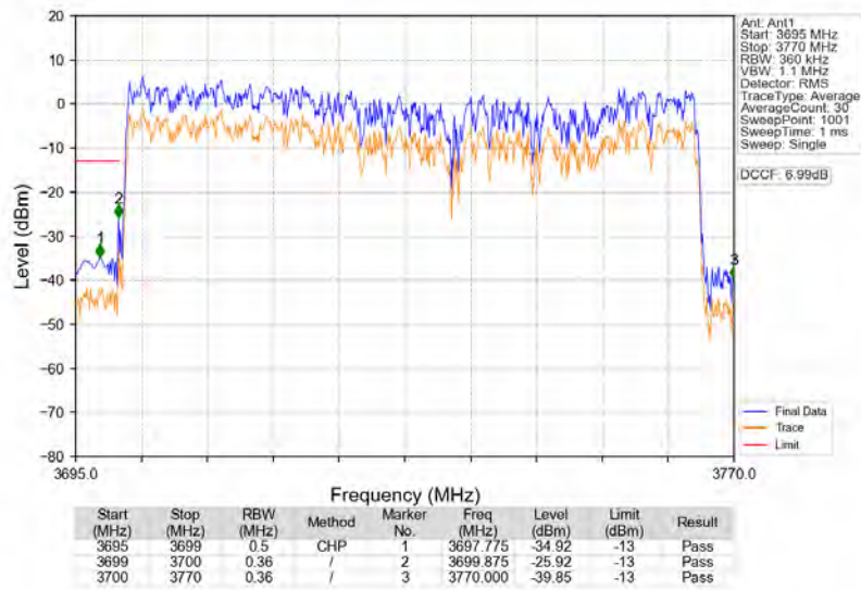
n77a_30kHz_SISO_NTNV_70MHz_DFT-s-OFDM_QPSK_3735MHz_Outer_Full
