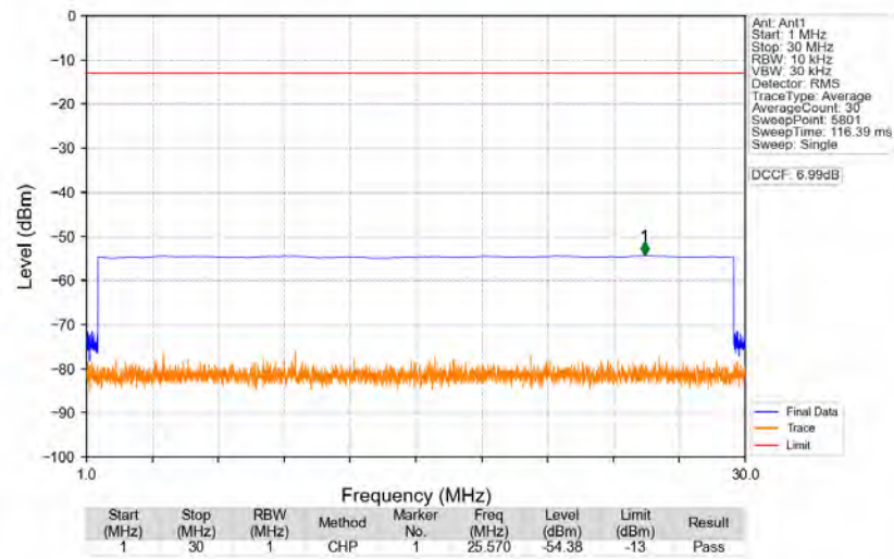
n77a_30kHz_SISO_NTNV_50MHz_DFT-s-OFDM_QPSK_3725.01MHz_Edge_1RB_Left
