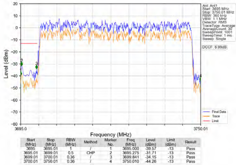
n77a_30kHz_SISO_NTNV_50MHz_DFT-s-OFDM_PI/2_BPSK_3725.01MHz_Outer_Full
