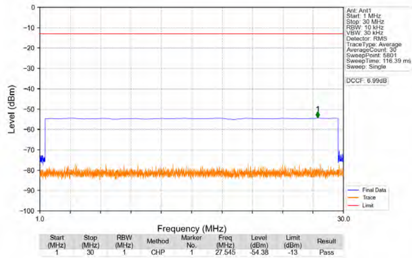
n77a_30kHz_SISO_NTNV_70MHz_DFT-s-OFDM_QPSK_3735MHz_Edge_1RB_Left
