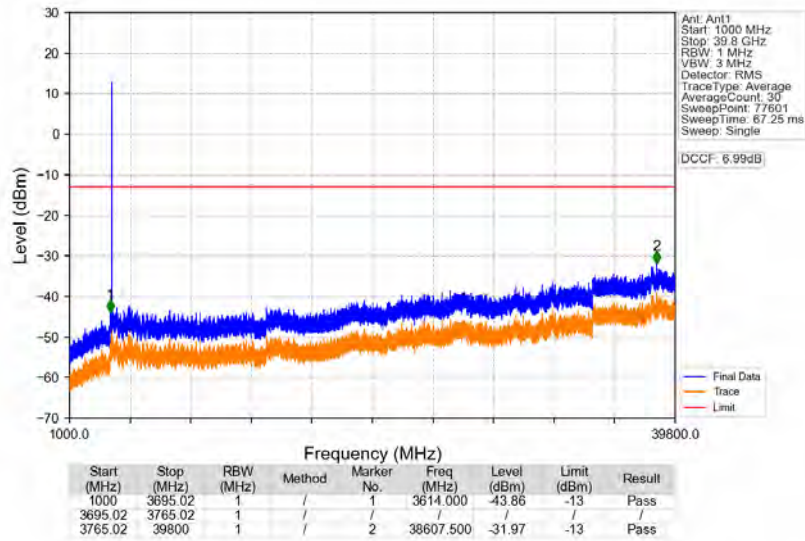
n77a_30kHz_SISO_NTNV_60MHz_DFT-s-OFDM_QPSK_3730.02MHz_Edge_1RB_Left
