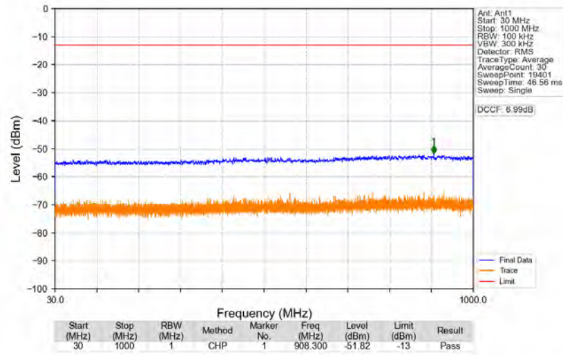
n77a_30kHz_SISO_NTNV_60MHz_DFT-s-OFDM_PI/2_BPSK_3840MHz_Edge_1RB_Left
