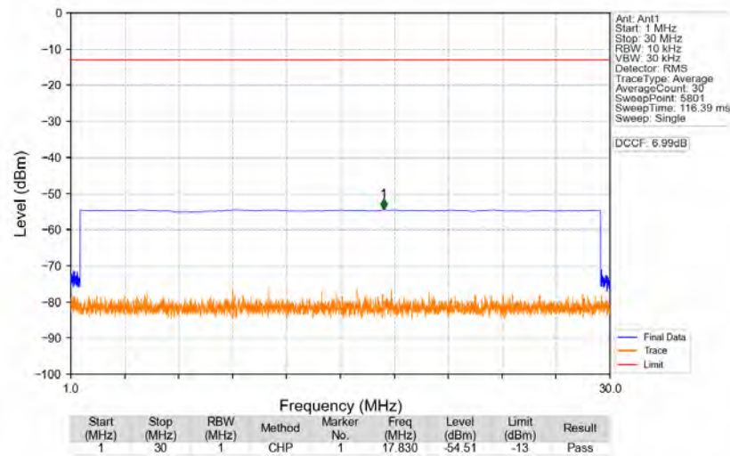
n77a_30kHz_SISO_NTNV_40MHz_CP-OFDM_QPSK_3840MHz_Edge_1RB_Left
