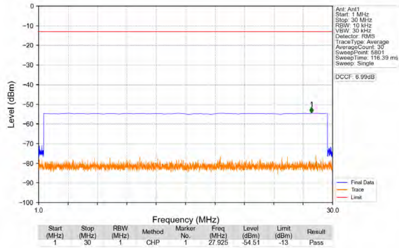
n77a_30kHz_SISO_NTNV_30MHz_DFT-s-OFDM_QPSK_3840MHz_Edge_1RB_Left
