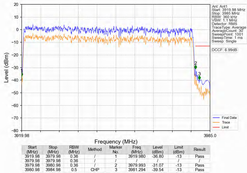
n77a 30kHz SISO NTN 60MHz CP-OFDM QPSK 3949.98MHz Outer Full
