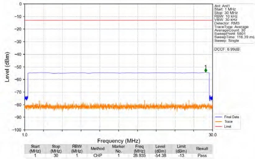
n77a_30kHz_SISO_NTNV_50MHz_DFT-s-OFDM_PI/2_BPSK_3840MHz_Edge_1RB_Left
