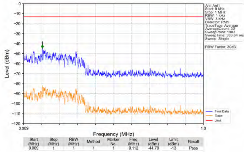
n77a_30kHz_SISO_NTNV_30MHz_DFT-s-OFDM_QPSK_3840MHz_Edge_1RB_Left
