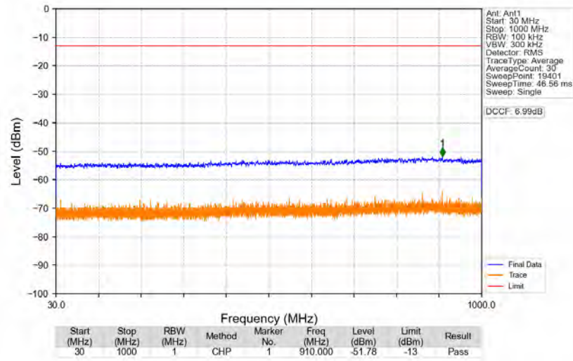
n77a_30kHz_SISO_NTNV_70MHz_DFT-s-OFDM_QPSK_3840MHz_Edge_1RB_Left
