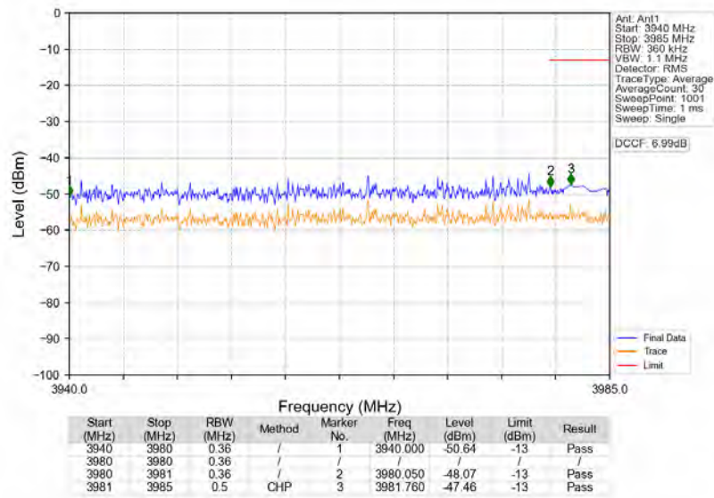
n77a_30kHz_SISO_NTNV_40MHz_DFT-s-OFDM_PI/2_BPSK_3960MHz_Outer_Full
