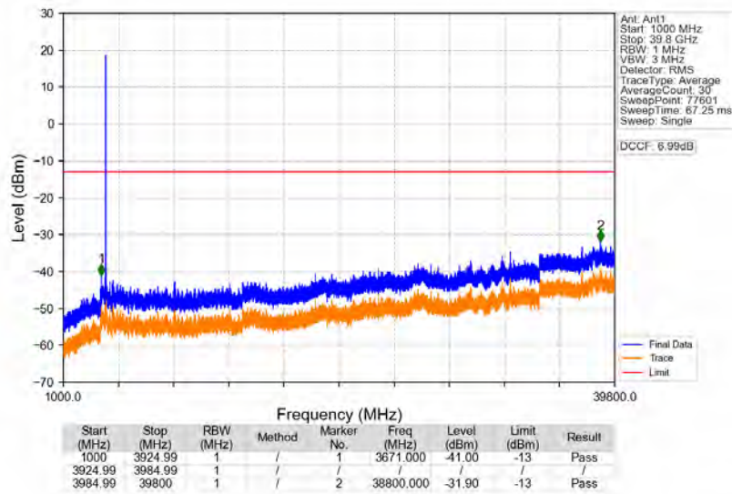
n77a 30kHz SISO NTN 50MHz CP-OFDM QPSK 3954.99MHz Edge_1RB_Right
