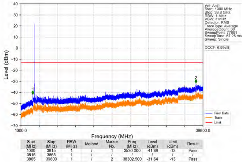
n77a_30kHz_SISO_NTNV_40MHz_DFT-s-OFDM_PI/2_BPSK_3840MHz_Edge_1RB_Left
