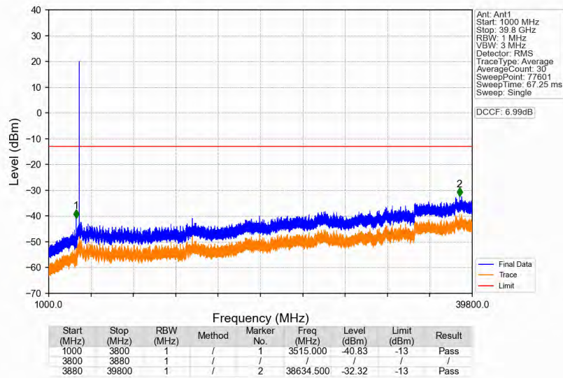
n77a_30kHz_SISO_NTNV_70MHz_DFT-s-OFDM_PI/2_BPSK_3840MHz_Edge_1RB_Left
