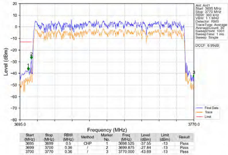
n77a 30kHz SISO NTN 70MHz DFT-s-OFDM PI/2 BPSK 3735MHz Outer Full
