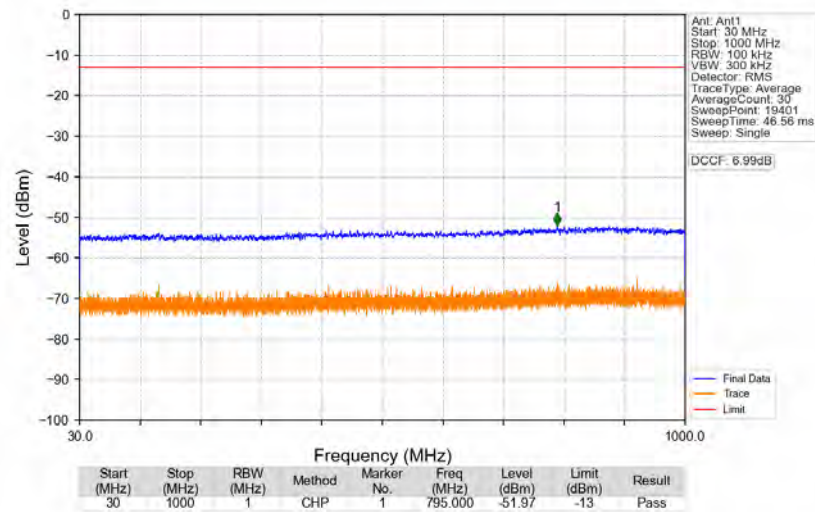
n77a_30kHz_SISO_NTNV_60MHz_DFT-s-OFDM_QPSK_3730.02MHz_Edge_1RB_Left
