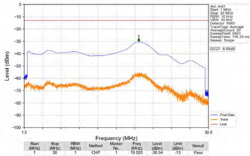
n77a_30kHz_SISO_NTNV_30MHz_CP-OFDM_QPSK_3715.02MHz_Edge_1RB_Left
