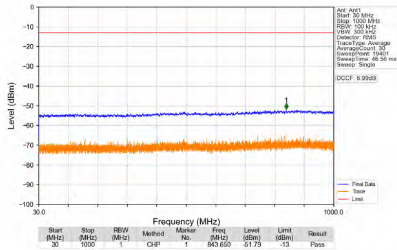
n77a_30kHz_SISO_NTNV_30MHz_DFT-s-OFDM_PI/2_BPSK_3840MHz_Edge_1RB_Left
