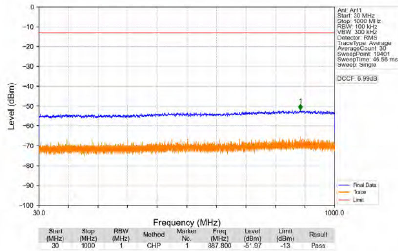
n77a_30kHz_SISO_NTNV_40MHz_DFT-s-OFDM_QPSK_3720MHz_Edge_1RB_Left
