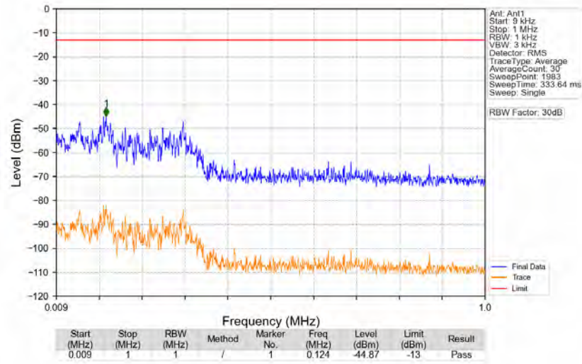
n77a_30kHz_SISO_NTNV_70MHz_DFT-s-OFDM_PI/2_BPSK_3840MHz_Edge_1RB_Left
