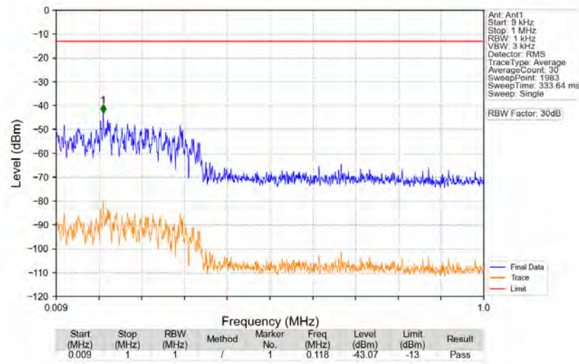
n77a_30kHz_SISO_NTNV_40MHz_DFT-s-OFDM_QPSK_3840MHz_Edge_1RB_Left
