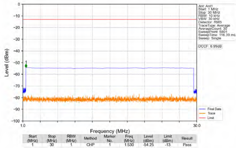
n77a_30kHz_SISO_NTNV_30MHz_DFT-s-OFDM_QPSK_3964.98MHz_Edge_1RB_Right
