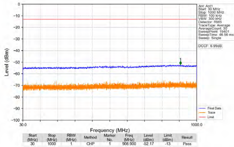
n77a_30kHz_SISO_NTNV_30MHz_DFT-s-OFDM_QPSK_3715.02MHz_Edge_1RB_Left
