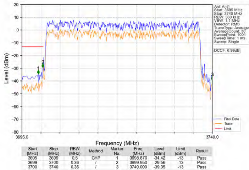
n77a_30kHz_SISO_NTNV_40MHz_DFT-s-OFDM_QPSK_3720MHz_Outer_Full
