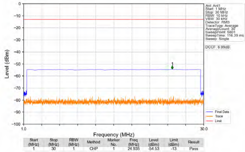
n77a_30kHz_SISO_NTNV_50MHz_CP-OFDM_QPSK_3840MHz_Edge_1RB_Left
