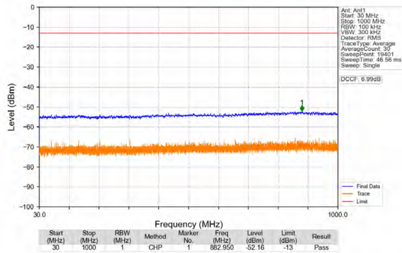
n77a_30kHz_SISO_NTNV_40MHz_CP-OFDM_QPSK_3720MHz_Edge_1RB_Left
