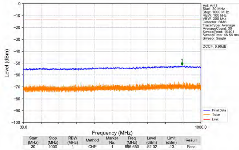
n77a_30kHz_SISO_NTNV_70MHz_DFT-s-OFDM_PI/2_BPSK_3840MHz_Edge_1RB_Left
