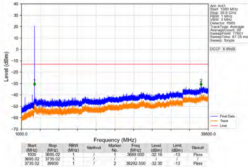
n77a_30kHz_SISO_NTNV_30MHz_CP-OFDM_QPSK_3715.02MHz_Edge_1RB_Left
