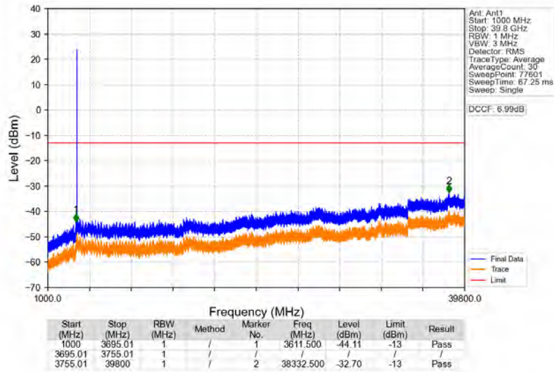
n77a_30kHz_SISO_NTNV_50MHz_DFT-s-OFDM_PI/2_BPSK_3725.01MHz_Edge_1RB_Left
