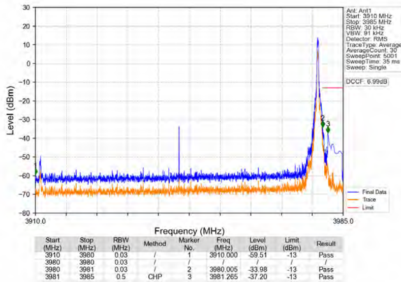
n77a_30kHz_SISO_NTNV_70MHz_DFT-s-OFDM_PI/2_BPSK_3945MHz_Edge_1RB_Right
