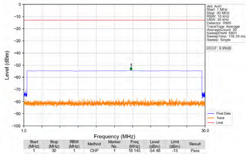
n77a_30kHz_SISO_NTNV_50MHz_DFT-s-OFDM_QPSK_3954.99MHz_Edge_1RB_Right
