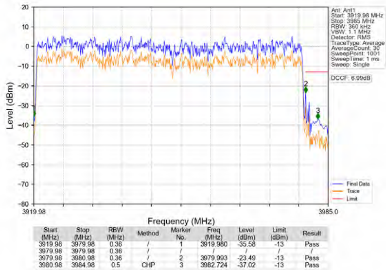
n77a_30kHz_SISO_NTNV_60MHz_DFT-s-OFDM_QPSK_3949.98MHz_Outer_Full
