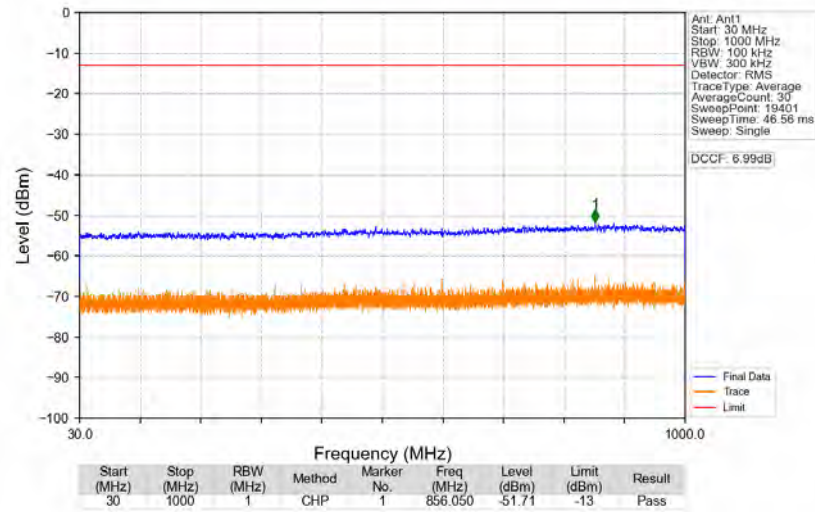
n77a_30kHz_SISO_NTNV_50MHz_DFT-s-OFDM_PI/2_BPSK_3840MHz_Edge_1RB_Left
