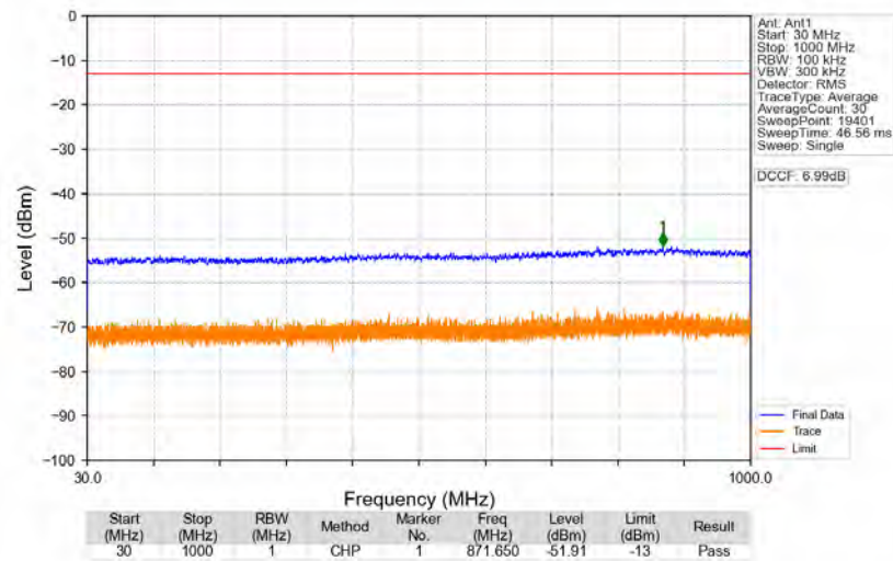
n77a_30kHz_SISO_NTNV_50MHz_DFT-s-OFDM_QPSK_3954.99MHz_Edge_1RB_Right
