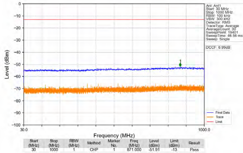
n77a_30kHz_SISO_NTNV_70MHz_DFT-s-OFDM_PI/2_BPSK_3735MHz_Edge_1RB_Left
