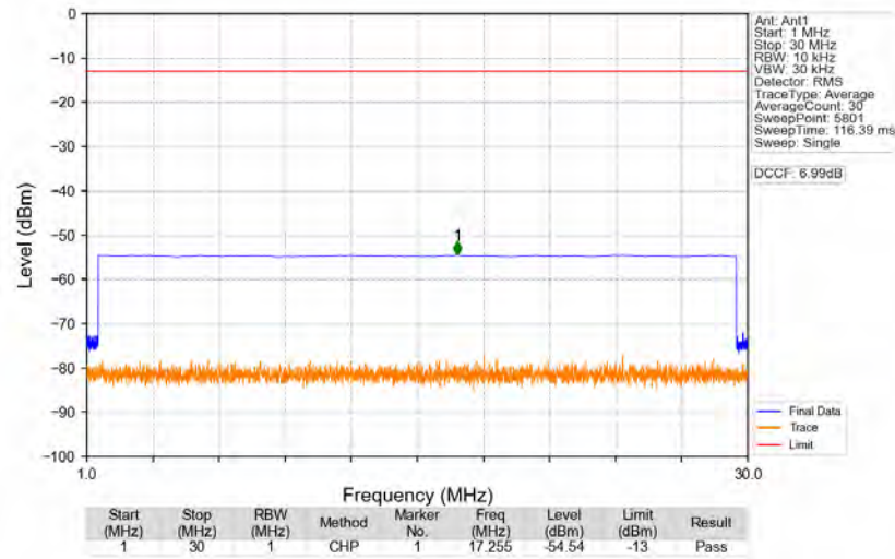
n77a_30kHz_SISO_NTNV_60MHz_DFT-s-OFDM_PI/2_BPSK_3840MHz_Edge_1RB_Left
