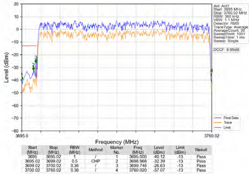
n77a_30kHz_SISO_NTNV_60MHz_DFT-s-OFDM_PI/2_BPSK_3730.02MHz_Outer_Full
