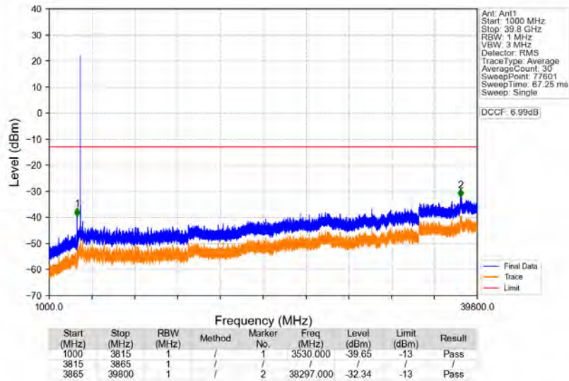
n77a_30kHz_SISO_NTNV_40MHz_DFT-s-OFDM_QPSK_3840MHz_Edge_1RB_Left
