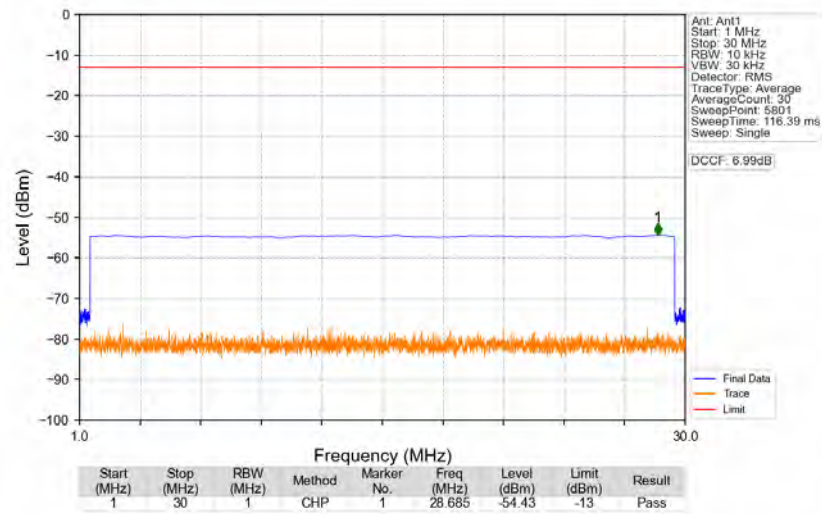
n77a_30kHz_SISO_NTNV_60MHz_DFT-s-OFDM_QPSK_3949.98MHz_Edge_1RB_Right
