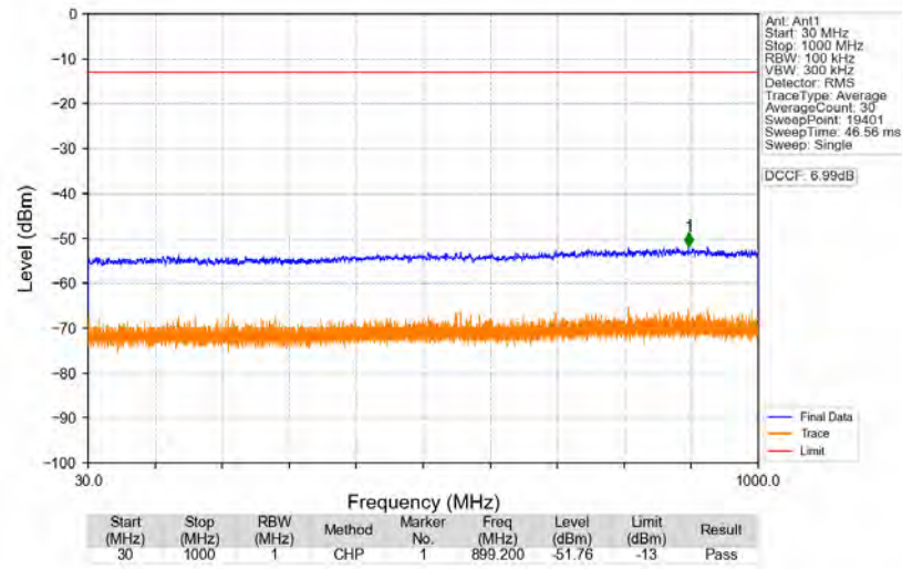
n77a_30kHz_SISO_NTNV_60MHz_CP-OFDM_QPSK_3840MHz_Edge_1RB_Left
