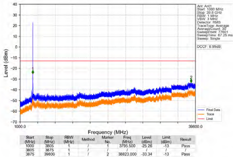
n77a_30kHz_SISO_NTNV_60MHz_DFT-s-OFDM_QPSK_3840MHz_Edge_1RB_Left
