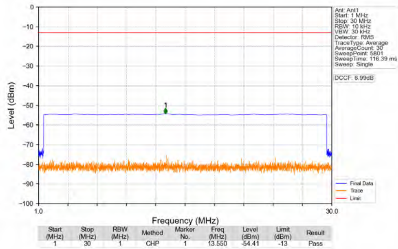
n77a_30kHz_SISO_NTNV_60MHz_DFT-s-OFDM_QPSK_3730.02MHz_Edge_1RB_Left
