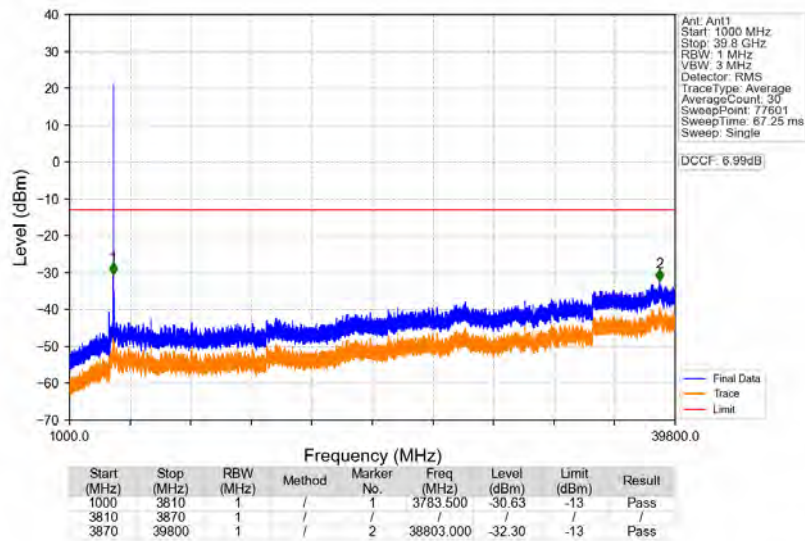
n77a_30kHz_SISO_NTNV_50MHz_DFT-s-OFDM_PI/2_BPSK_3840MHz_Edge_1RB_Left
