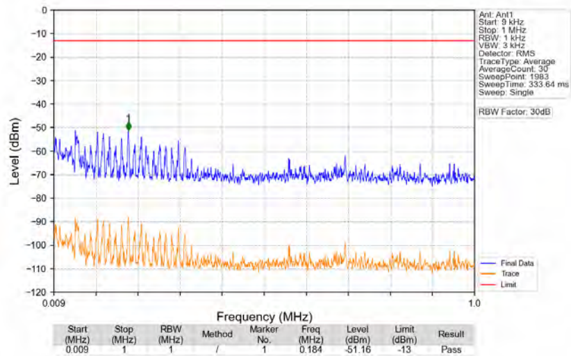
n77a_30kHz_SISO_NTNV_50MHz_DFT-s-OFDM_QPSK_3954.99MHz_Edge_1RB_Right
