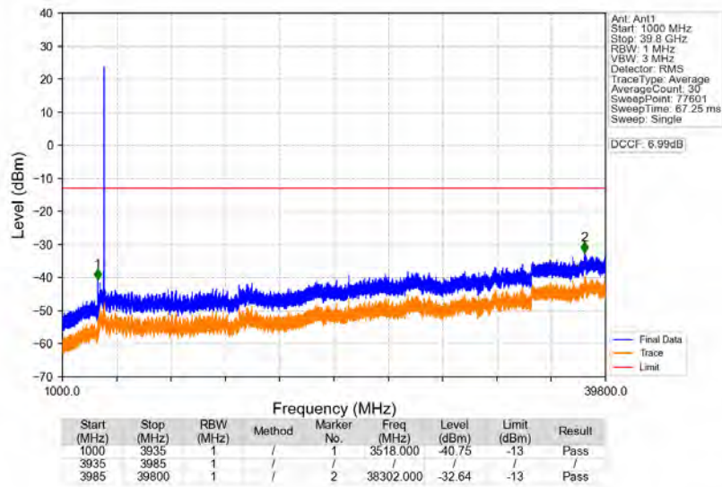
n77a_30kHz_SISO_NTNV_40MHz_DFT-s-OFDM_PI/2_BPSK_3960MHz_Edge_1RB_Right
