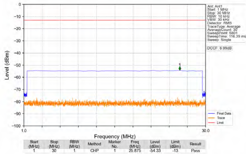
n77a_30kHz_SISO_NTNV_50MHz_DFT-s-OFDM_QPSK_3840MHz_Edge_1RB_Left
