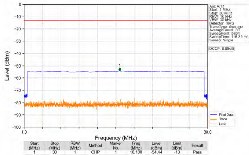
n77a_30kHz_SISO_NTNV_40MHz_DFT-s-OFDM_PI/2_BPSK_3840MHz_Edge_1RB_Left
