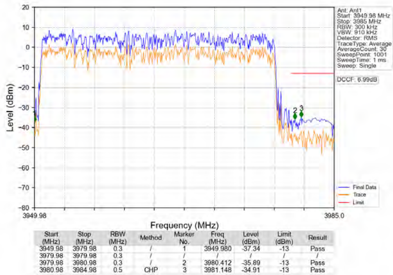
n77a_30kHz_SISO_NTNV_30MHz_DFT-s-OFDM_QPSK_3964.98MHz_Outer_Full
