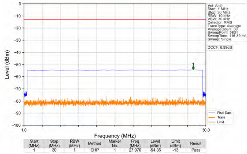
n77a_30kHz_SISO_NTNV_70MHz_DFT-s-OFDM_PI/2_BPSK_3735MHz_Edge_1RB_Left
