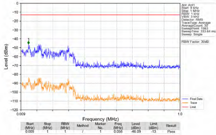
n77a_30kHz_SISO_NTNV_30MHz_DFT-s-OFDM_PI/2_BPSK_3840MHz_Edge_1RB_Left
