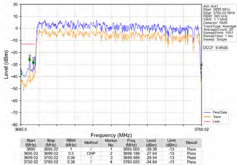
n77a_30kHz_SISO_NTNV_60MHz_DFT-s-OFDM_QPSK_3730.02MHz_Outer_Full
