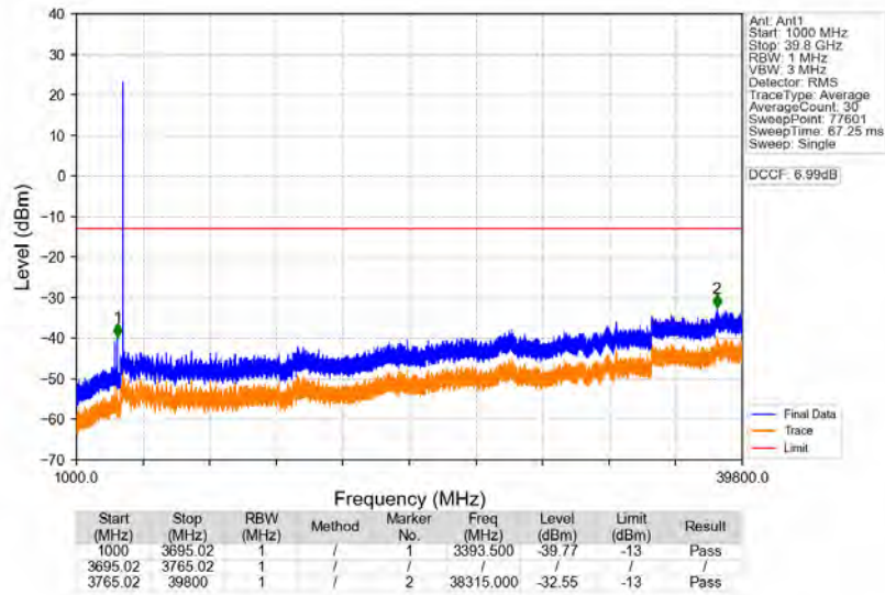
n77a_30kHz_SISO_NTNV_60MHz_DFT-s-OFDM_PI/2_BPSK_3730.02MHz_Edge_1RB_Left
