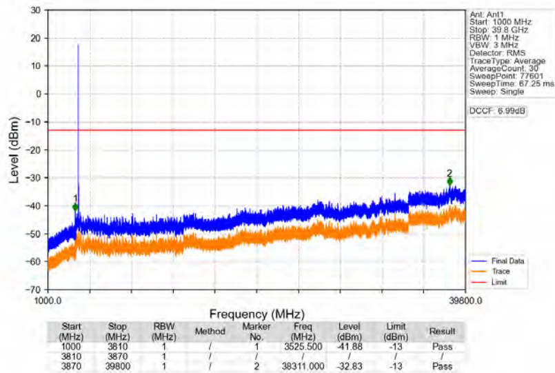
n77a_30kHz_SISO_NTNV_50MHz_CP-OFDM_QPSK_3840MHz_Edge_1RB_Left
