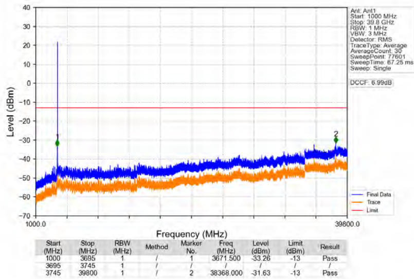
n77a_30kHz_SISO_NTNV_40MHz_CP-OFDM_QPSK_3720MHz_Edge_1RB_Left
