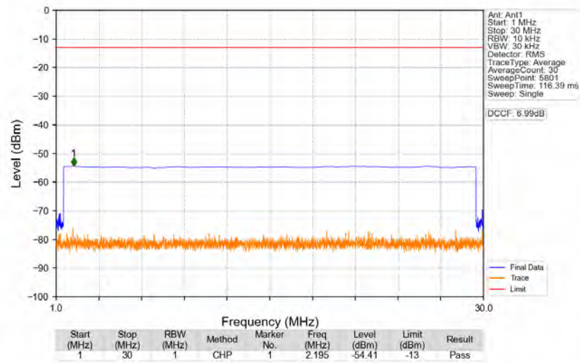
n77a_30kHz_SISO_NTNV_30MHz_DFT-s-OFDM_QPSK_3715.02MHz_Edge_1RB_Left
