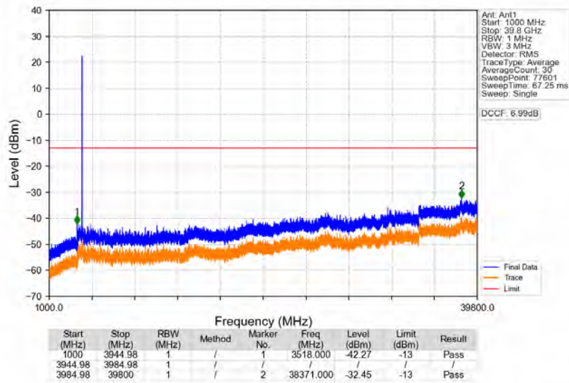
n77a_30kHz_SISO_NTNV_30MHz_DFT-s-OFDM_QPSK_3964.98MHz_Edge_1RB_Right
