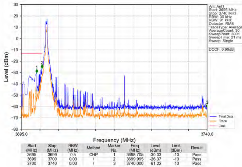
n77a_30kHz_SISO_NTNV_40MHz_DFT-s-OFDM_QPSK_3720MHz_Edge_1RB_Left
