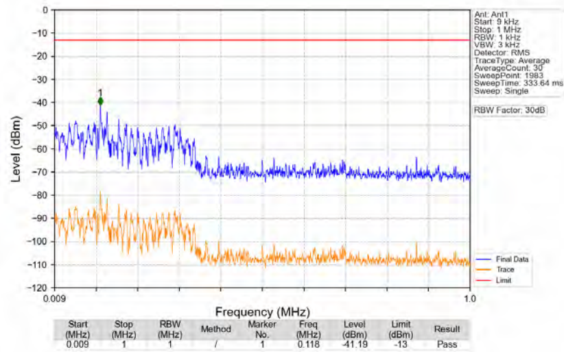
n77a_30kHz_SISO_NTNV_40MHz_DFT-s-OFDM_PI/2_BPSK_3840MHz_Edge_1RB_Left
