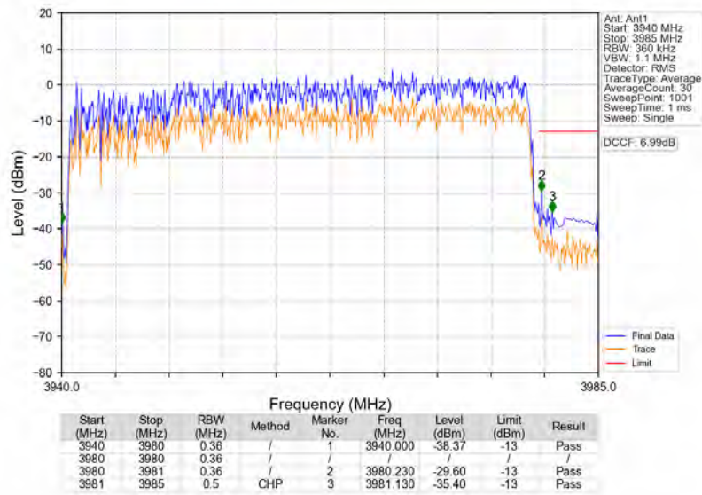
n77a 30kHz SISO NTN 40MHz CP-OFDM QPSK 3960MHz Outer Full
