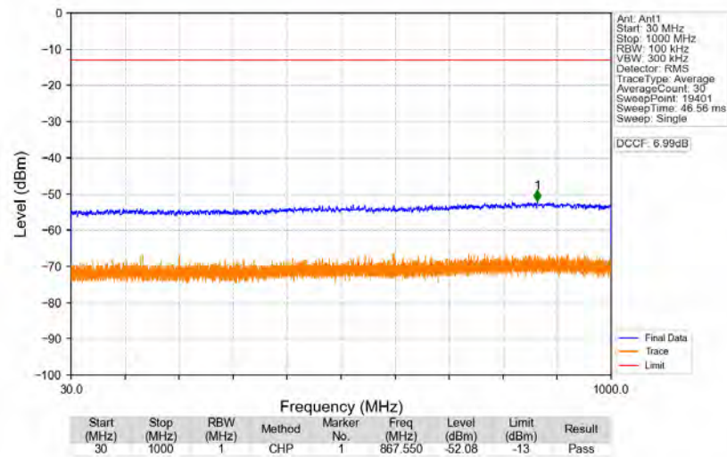
n77a_30kHz_SISO_NTNV_30MHz_DFT-s-OFDM_QPSK_3964.98MHz_Edge_1RB_Right
