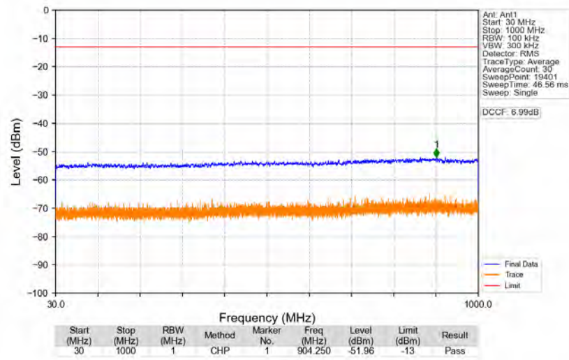
n77a_30kHz_SISO_NTNV_50MHz_DFT-s-OFDM_QPSK_3840MHz_Edge_1RB_Left
