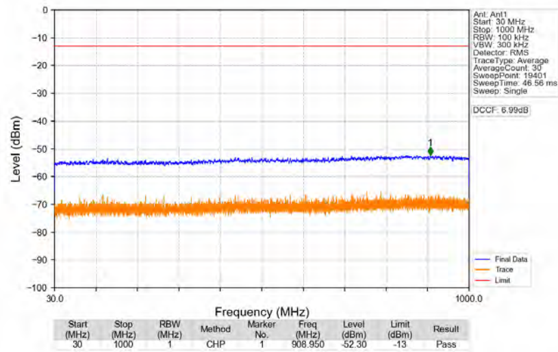
n77a_30kHz_SISO_NTNV_70MHz_DFT-s-OFDM_QPSK_3735MHz_Edge_1RB_Left
