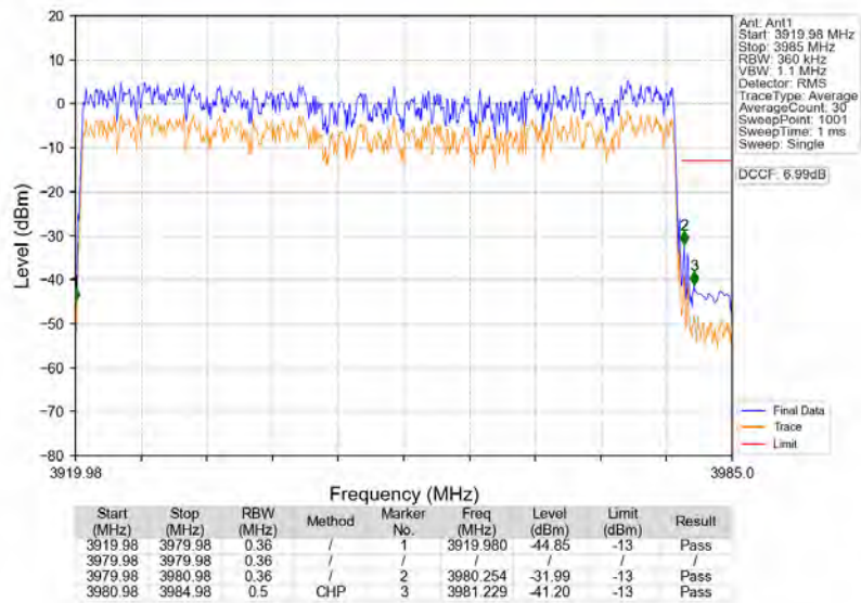
n77a_30kHz_SISO_NTNV_60MHz_DFT-s-OFDM_PI/2_BPSK_3949.98MHz_Outer_Full
