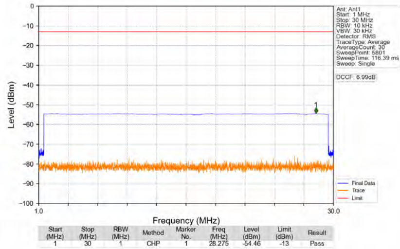
n77a_30kHz_SISO_NTNV_50MHz_CP-OFDM_QPSK_3725.01MHz_Edge_1RB_Left
