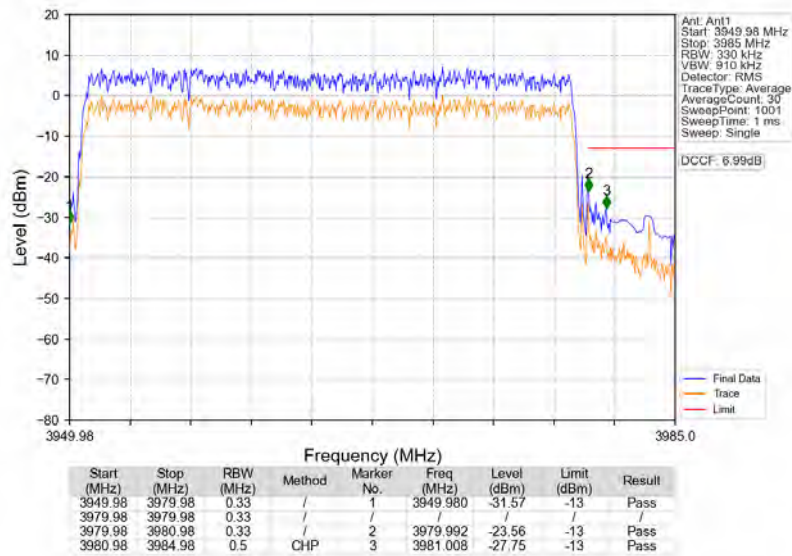
n77a 30kHz SISO NTN 30MHz CP-OFDM QPSK 3964.98MHz Outer_Full
