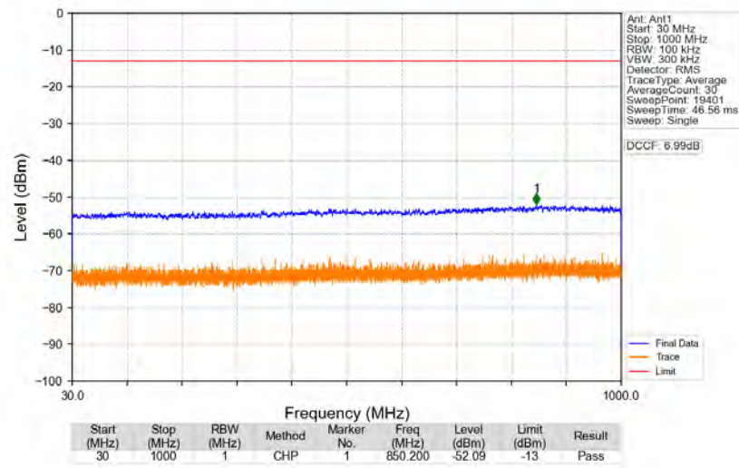
n77a_30kHz_SISO_NTNV_60MHz_DFT-s-OFDM_QPSK_3840MHz_Edge_1RB_Left
