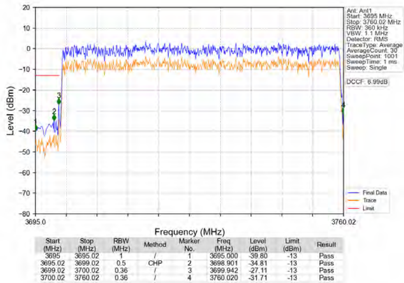
n77a_30kHz_SISO_NTNV_60MHz_CP-OFDM_QPSK_3730.02MHz_Outer_Full
