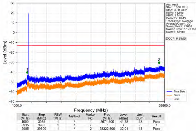
n77a 30kHz SISO NTN 40MHz CP-OFDM QPSK 3960MHz Edge_1RB_Right
