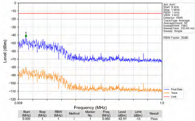
n77a_30kHz_SISO_NTNV_60MHz_CP-OFDM_QPSK_3730.02MHz_Edge_1RB_Left
