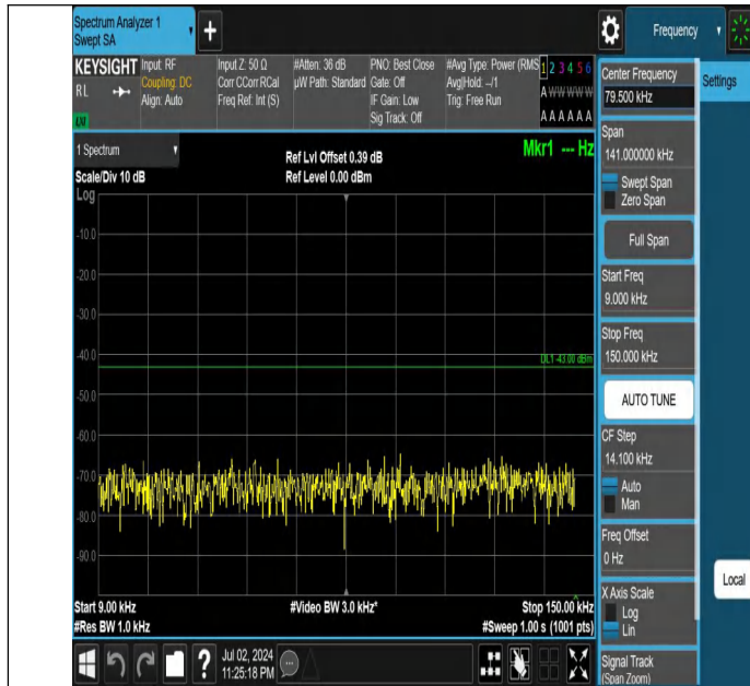
Band66-20MHz-QPSK-132322-1RB#0-0.009~0.15-PASS
