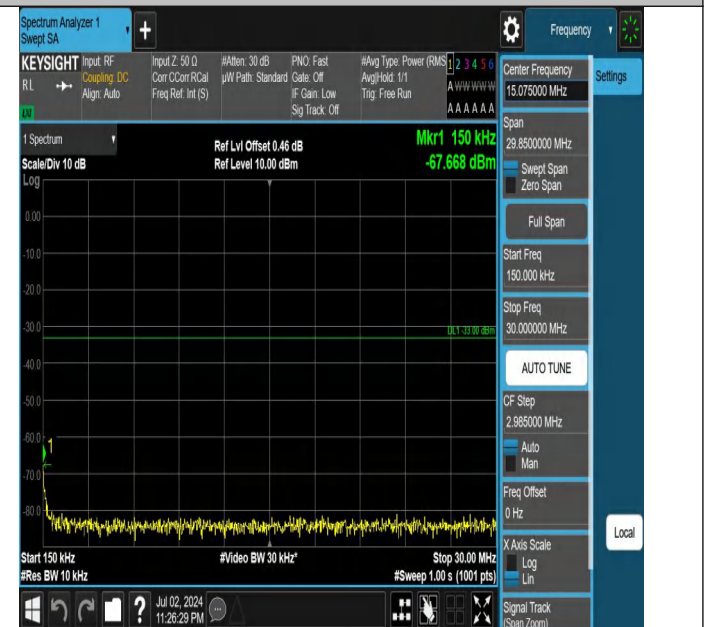
Band66-20MHz-QPSK-132572-1RB#0-0.15~30-PASS
