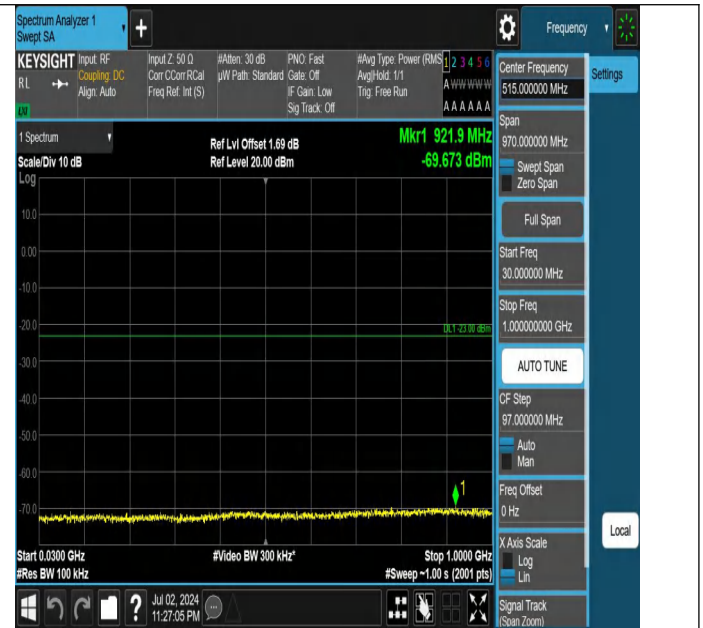
Band66-20MHz-QPSK-132572-1RB#99-30~1000-PASS
