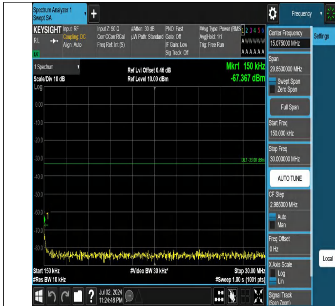
Band66-20MHz-QPSK-132072-1RB#99-0.15~30-PASS
