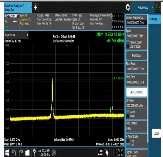
Band66-20MHz-QPSK-132322-1RB#0-1000~3000-PASS
