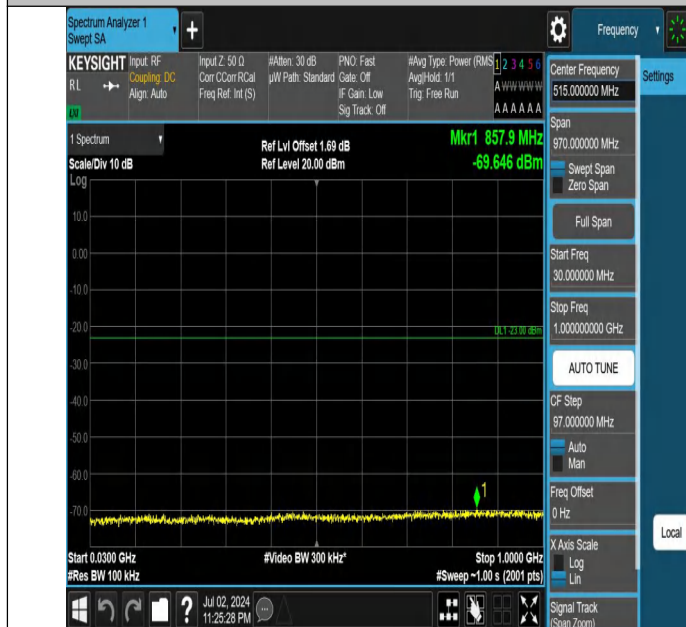
Band66-20MHz-QPSK-132322-1RB#0-30~1000-PASS
