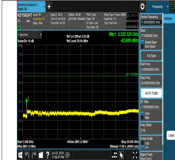
Band66-20MHz-QPSK-132572-1RB#0-3000~20000-PASS
