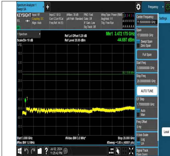
Band66-20MHz-QPSK-132322-1RB#0-3000~20000-PASS
