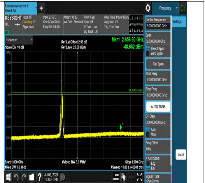
Band66-20MHz-QPSK-132572-1RB#0-1000~3000-PASS
