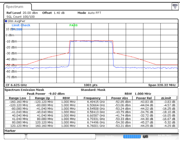
802.11ax (80MHz) 6625MHz Chain D NSS-4
