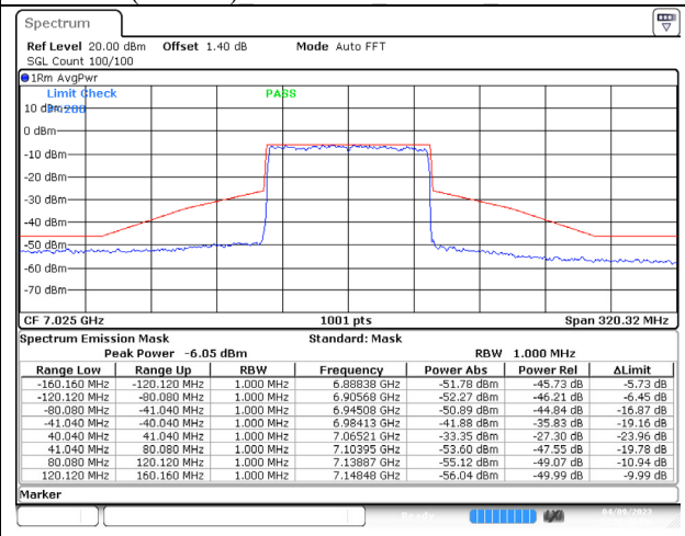
802.11ax (80MHz) 7025MHz Chain D NSS-4
