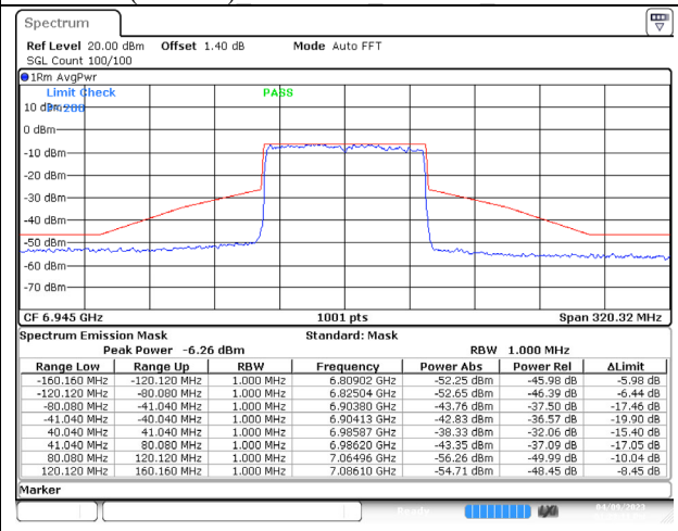
802.11ax (80MHz) 6945MHz Chain B NSS-4
