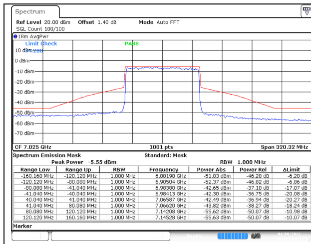
802.11ax (80MHz) 7025MHz Chain A NSS-4
