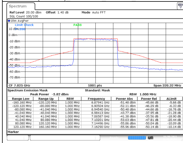
802.11ax (80MHz) 7025MHz Chain C NSS-4
