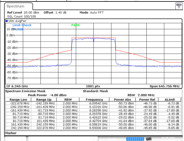
802.11ax (160MHz) 6345 CH79 4Tx Chain B NSS-4
