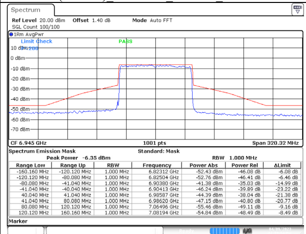
802.11ax (80MHz) 6945MHz Chain D NSS-4
