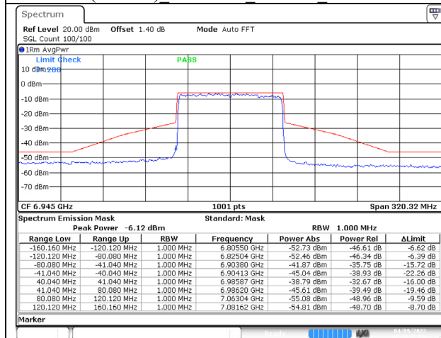
802.11ax (80MHz) 6945MHz Chain C NSS-4
