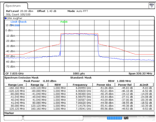
802.11ax (80MHz) 7025MHz Chain B NSS-4
