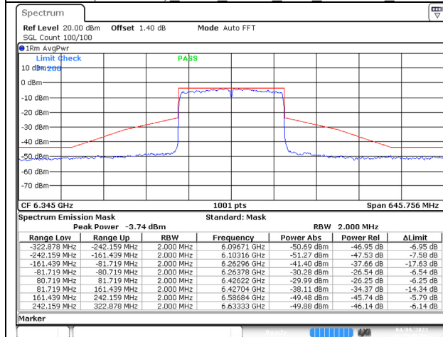
802.11ax (160MHz) 6345 CH79 4Tx Chain C NSS-4
