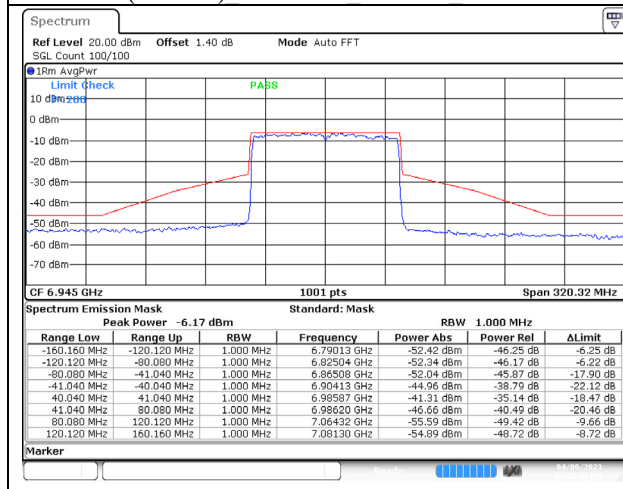
802.11ax (80MHz) 6945MHz Chain A NSS-4
