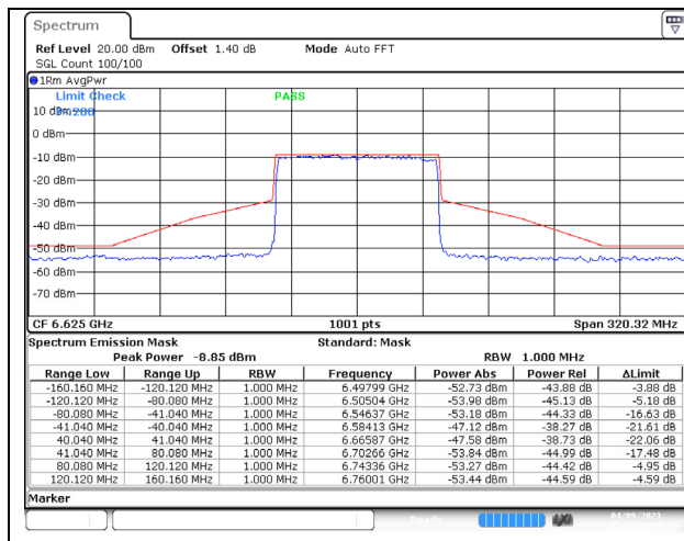
802.11ax (80MHz) 6625MHz Chain C NSS-4
