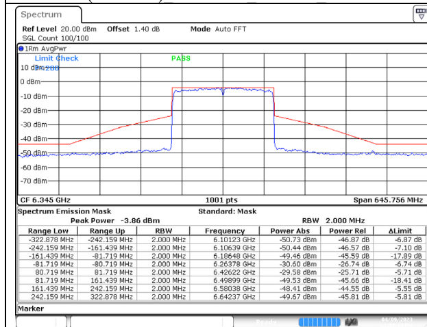
802.11ax (160MHz) 6345 CH79 4Tx Chain A NSS-4
