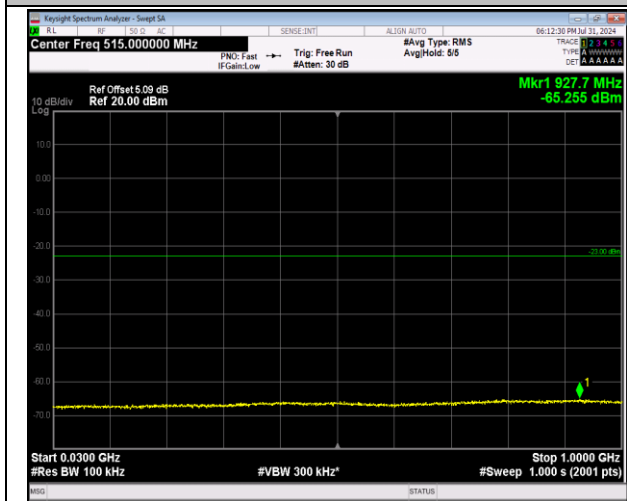
2-2-5MHz-20MHz-64QAM-64QAM-18633-18750-1RB#24-0RB#0-30~1000MHz-PASS
