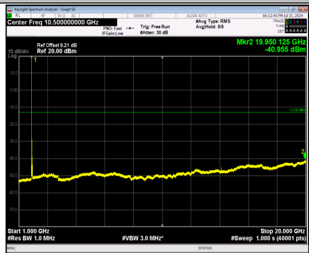
2-2-5MHz-20MHz-64QAM-64QAM-18633-18750-1RB#24-0RB#0-1000~20000MHz-PASS
