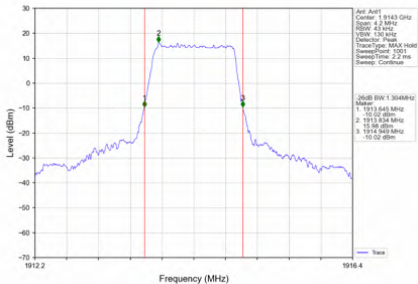
Band25_1.4MHz_256QAM_HCH_1914.3MHz_RB_6_0_NTNV
