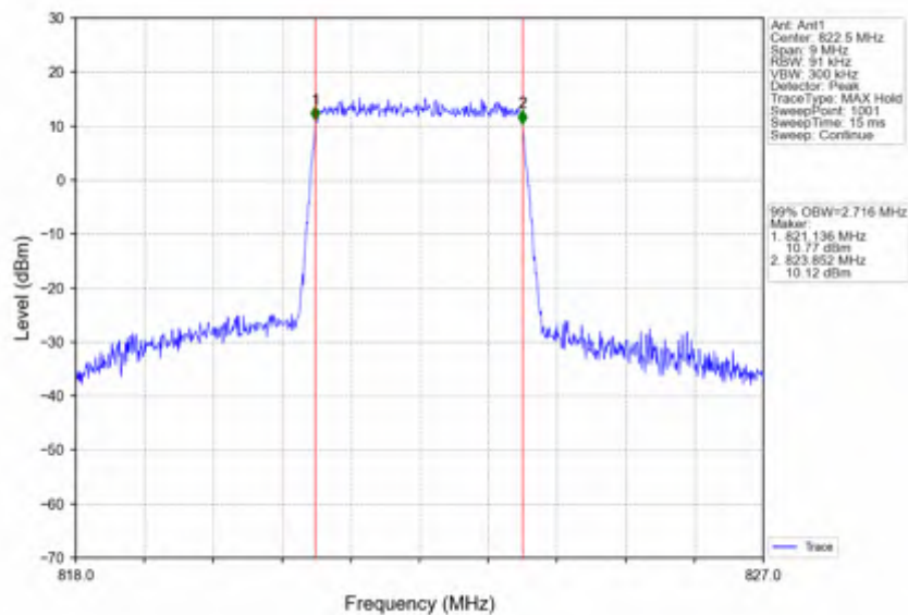
Band26a_3MHz_16QAM_HCH_822.5MHz_RB_15_0_NTNV
