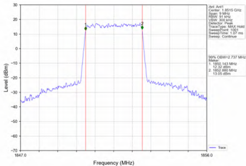
Band25_3MHz_16QAM_LCH_1851.5MHz_RB_15_0_NTNV
