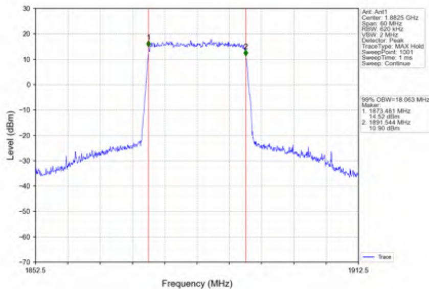
Band25_20MHz_QPSK_MCH_1882.5MHz_RB_100_0_NTNV
