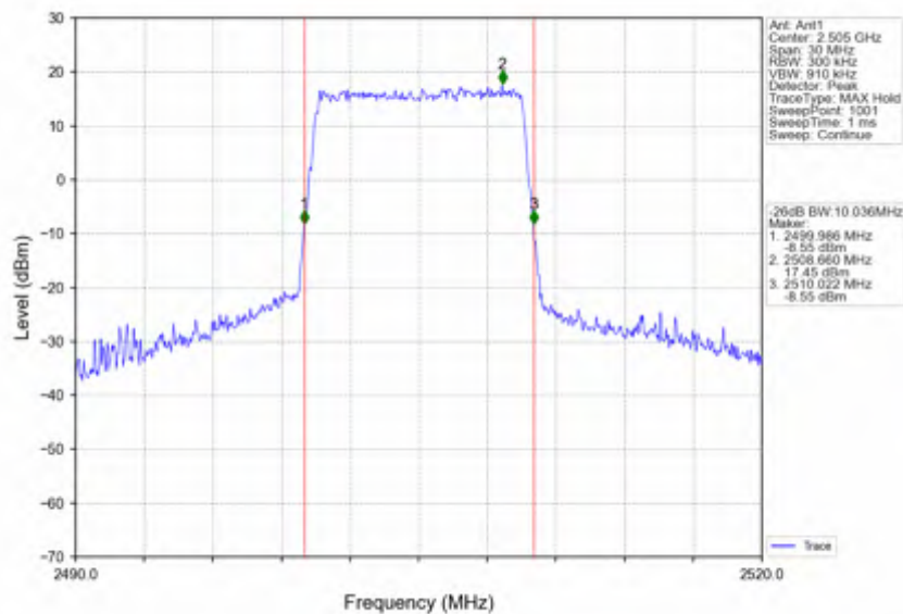
Band7_10MHz_16QAM_LCH_2505MHz_RB_50_0_NTNV
