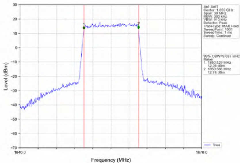
Band25_10MHz_16QAM_LCH_1855MHz_RB_50_0_NTNV
