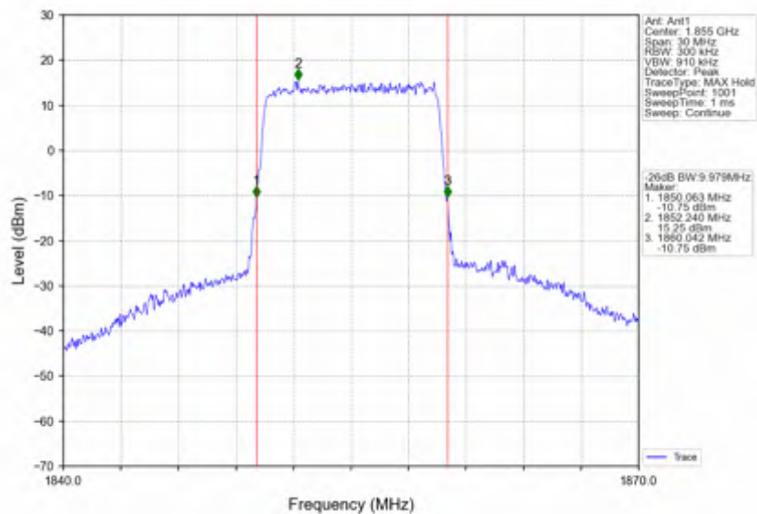
Band25_10MHz_256QAM_LCH_1855MHz_RB_50_0_NTNV
