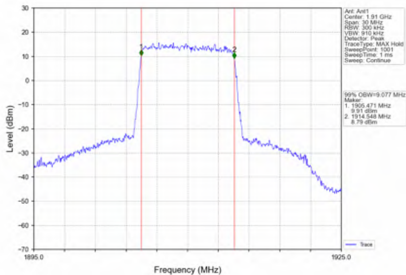
Band25_10MHz_256QAM_HCH_1910MHz_RB_50_0_NTNV
