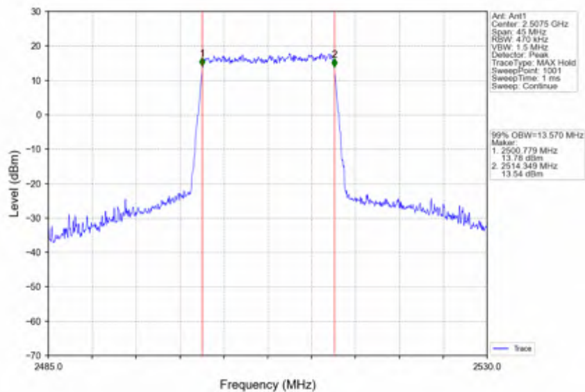
Band7_15MHz_16QAM_LCH_2507.5MHz_RB_75_0_NTNV
