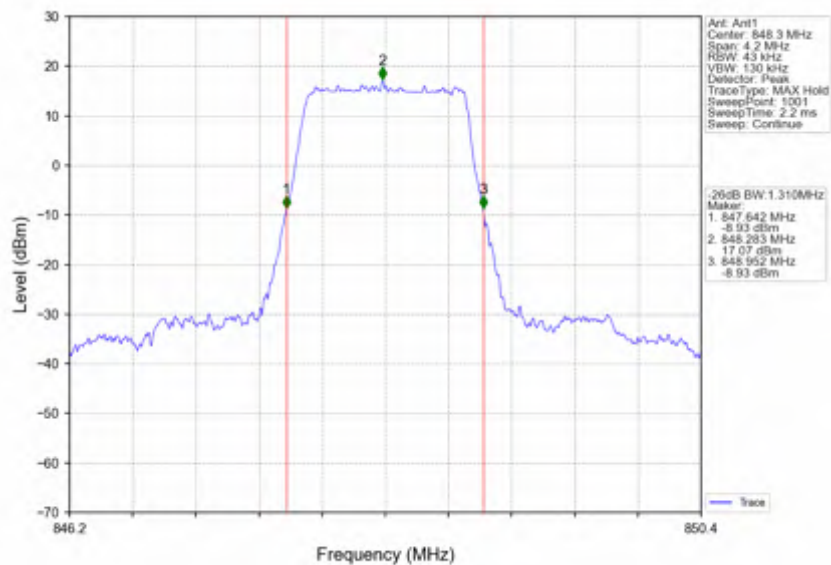
Band5_1.4MHz_256QAM_HCH_848.3MHz_RB_6_0_NTNV
