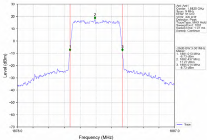
Band25_3MHz_QPSK_MCH_1882.5MHz_RB_15_0_NTNV
