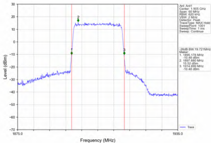
Band25_20MHz_256QAM_HCH_1905MHz_RB_100_0_NTNV
