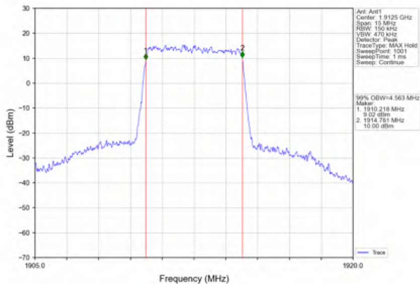
Band25_5MHz_256QAM_HCH_1912.5MHz_RB_25_0_NTNV
