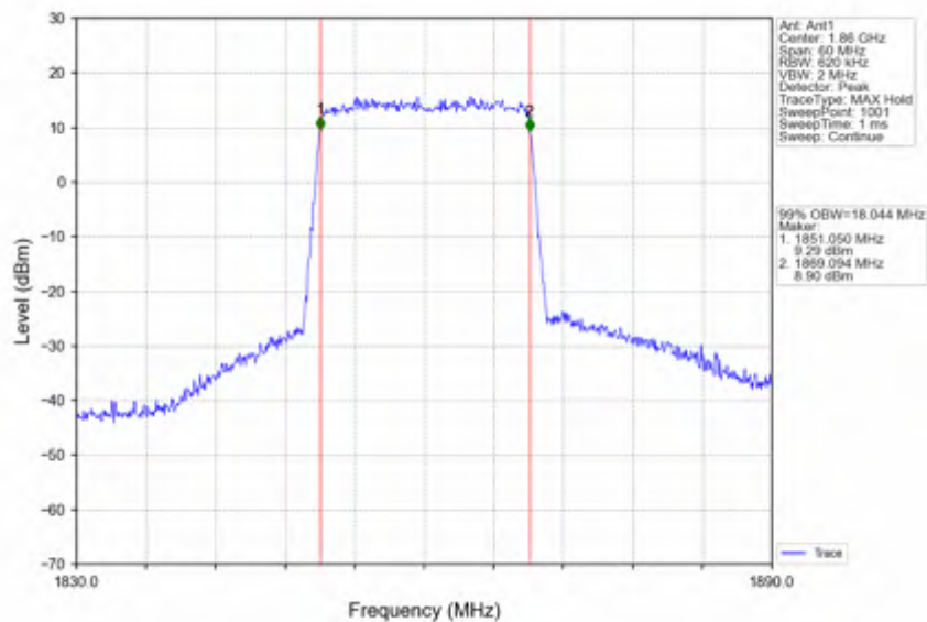
Band25_20MHz_256QAM_LCH_1860MHz_RB_100_0_NTNV
