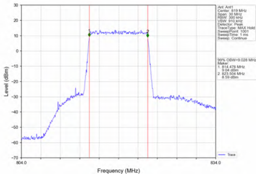
Band26a_10MHz_256QAM_HCH_819MHz_RB_50_0_NTNV
