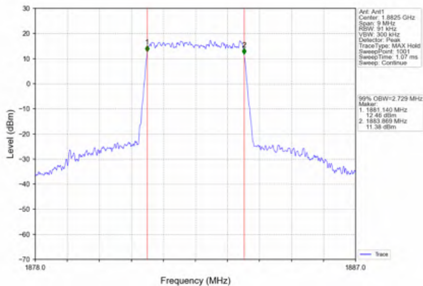
Band25_3MHz_64QAM_MCH_1882.5MHz_RB_15_0_NTNV
