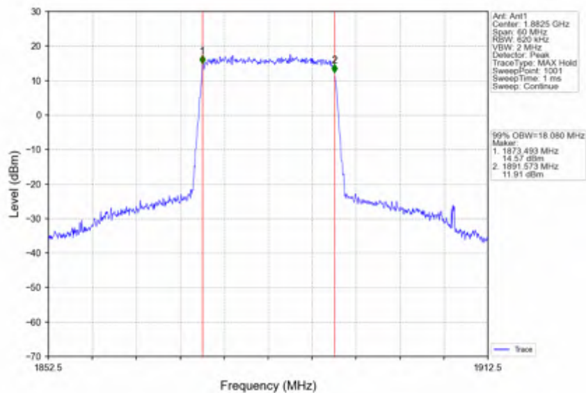
Band25_20MHz_64QAM_MCH_1882.5MHz_RB_100_0_NTNV
