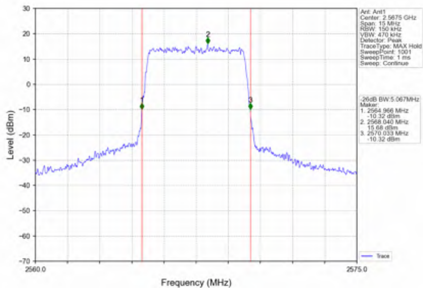
Band7_5MHz_256QAM_HCH_2567.5MHz_RB_25_0_NTNV
