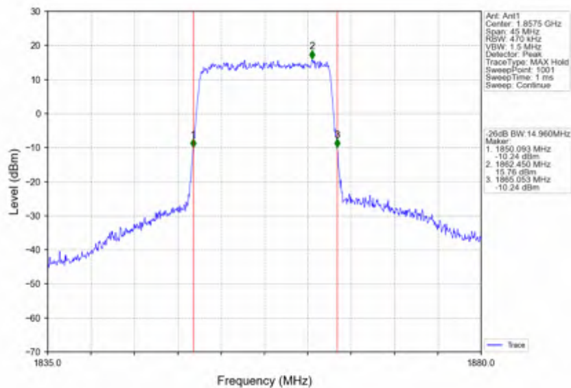
Band25_15MHz_256QAM_LCH_1857.5MHz_RB_75_0_NTNV
