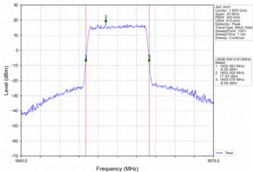
Band25_10MHz_16QAM_LCH_1855MHz_RB_50_0_NTNV
