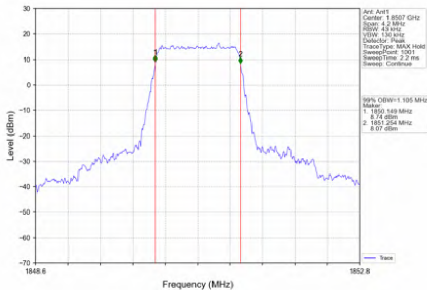
Band25_1.4MHz_256QAM_LCH_1850.7MHz_RB_6_0_NTNV
