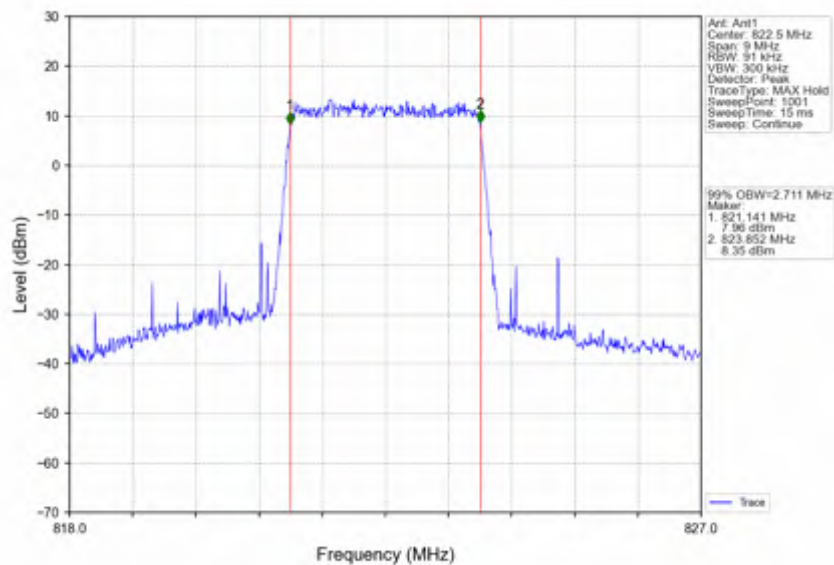
Band26a_3MHz_256QAM_HCH_822.5MHz_RB_15_0_NTNV
