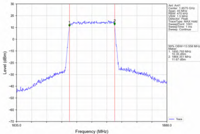
Band25_15MHz_256QAM_LCH_1857.5MHz_RB_75_0_NTNV
