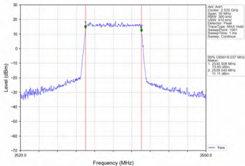
Band7_10MHz_64QAM_MCH_2535MHz_RB_50_0_NTNV
