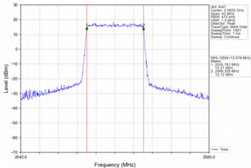
Band7_15MHz_16QAM_HCH_2562.5MHz_RB_75_0_NTNV
