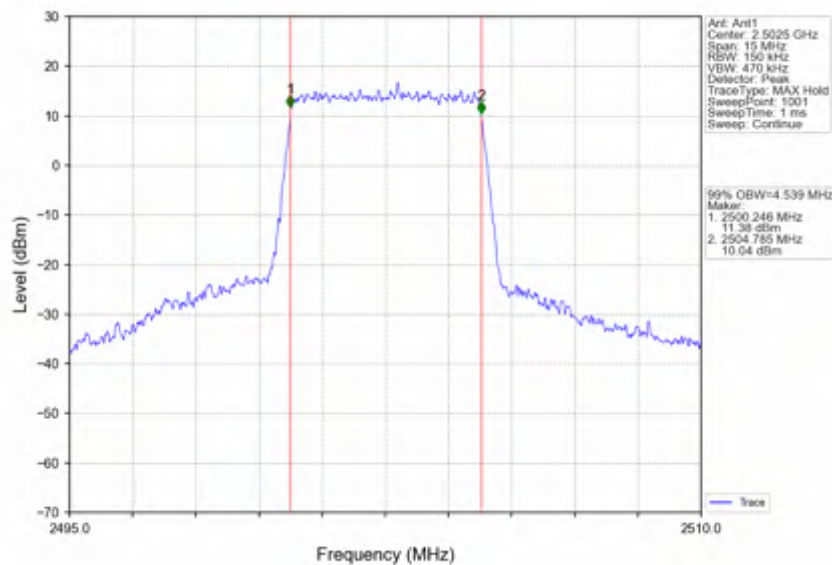
Band7_5MHz_256QAM_LCH_2502.5MHz_RB_25_0_NTNV
