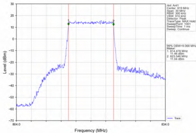
Band26a_10MHz_16QAM_HCH_819MHz_RB_50_0_NTNV
