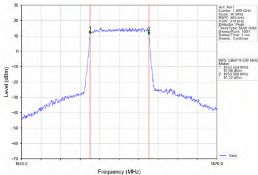
Band25_10MHz_256QAM_LCH_1855MHz_RB_50_0_NTNV
