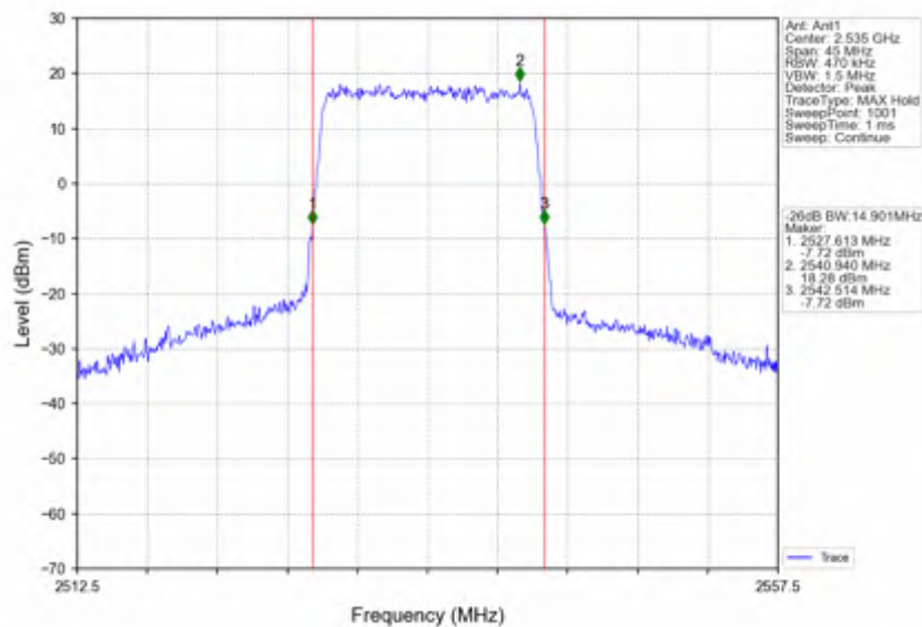
Band7_15MHz_64QAM_MCH_2535MHz_RB_75_0_NTNV
