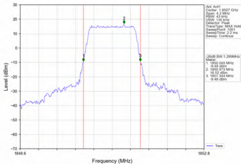
Band25_1.4MHz_256QAM_LCH_1850.7MHz_RB_6_0_NTNV
