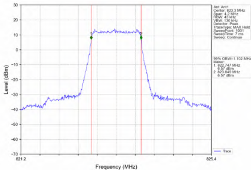
Band26a_1.4MHz_256QAM_HCH_823.3MHz_RB_6_0_NTNV
