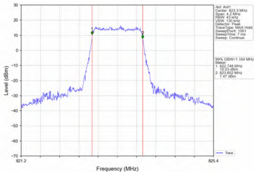
Band26a_1.4MHz_16QAM_HCH_823.3MHz_RB_6_0_NTNV
