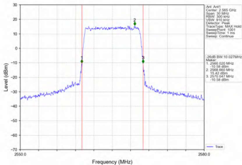
Band7_10MHz_256QAM_HCH_2565MHz_RB_50_0_NTNV
