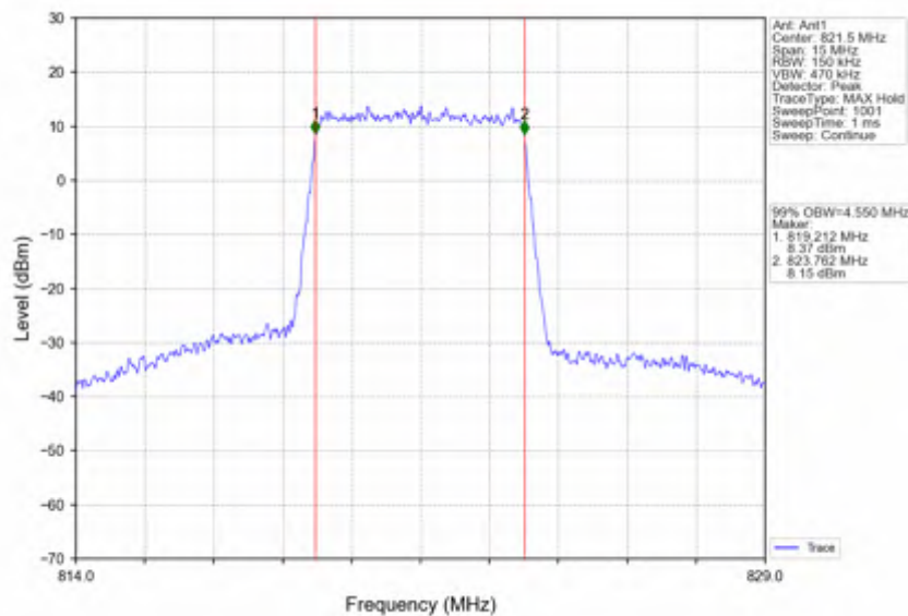
Band26a_5MHz_256QAM_HCH_821.5MHz_RB_25_0_NTNV
