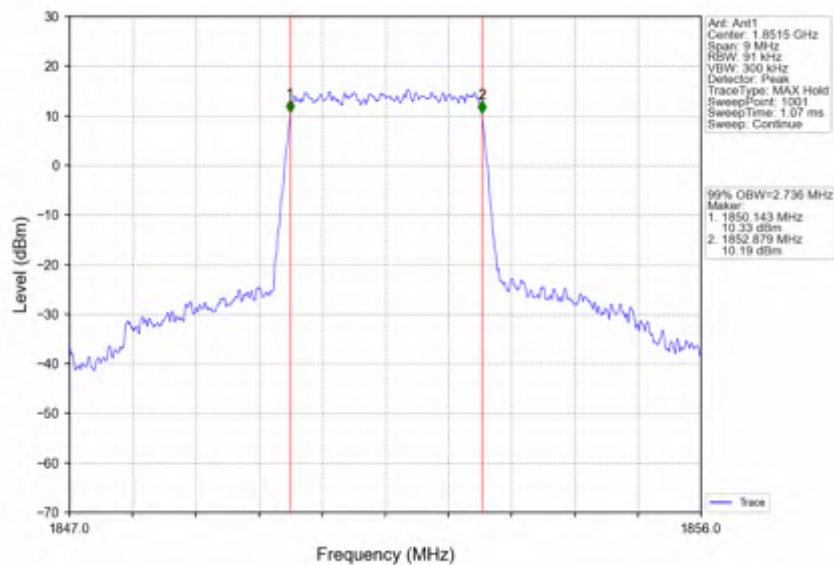
Band25_3MHz_256QAM_LCH_1851.5MHz_RB_15_0_NTNV
