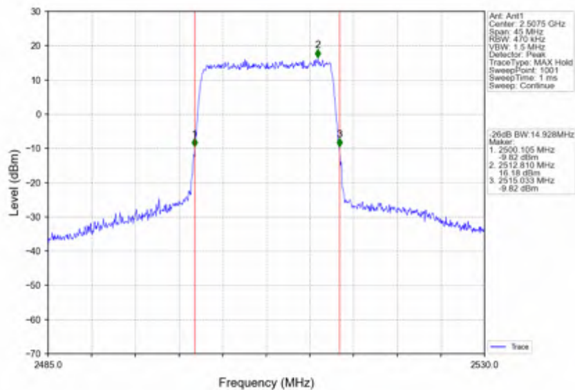
Band7_15MHz_256QAM_LCH_2507.5MHz_RB_75_0_NTNV
