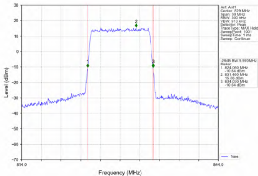
Band5_10MHz_256QAM_LCH_829MHz_RB_50_0_NTNV
