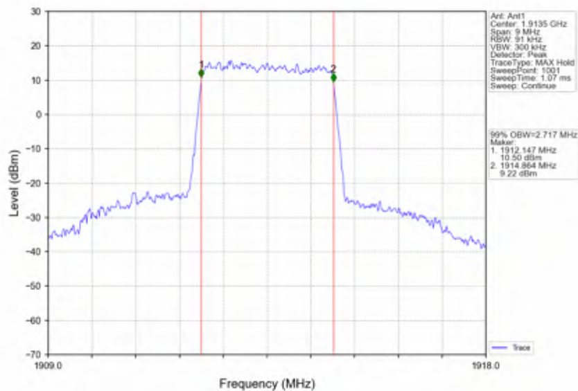
Band25_3MHz_256QAM_HCH_1913.5MHz_RB_15_0_NTNV
