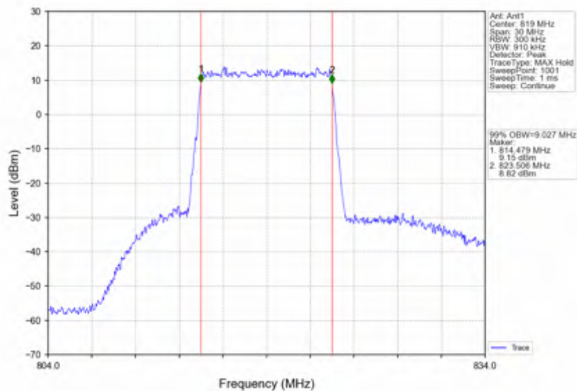
Band26a_10MHz_256QAM_LCH_819MHz_RB_50_0_NTNV
