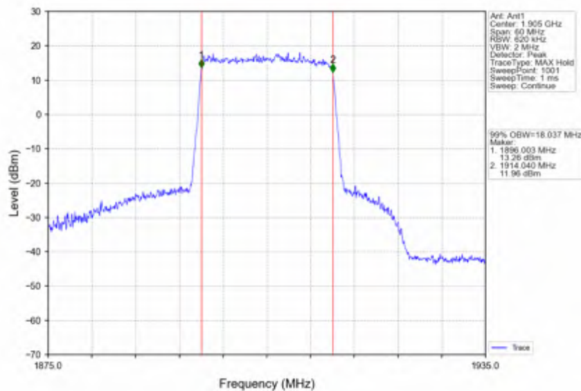
Band25_20MHz_16QAM_HCH_1905MHz_RB_100_0_NTNV
