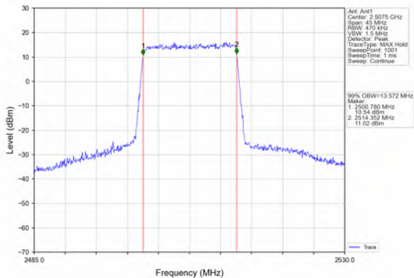
Band7_15MHz_256QAM_LCH_2507.5MHz_RB_75_0_NTNV
