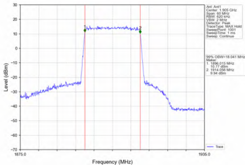
Band25 20MHz 256QAM HCH 1905MHz RB 100 0 NTNV
