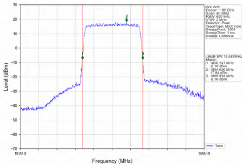
Band25_20MHz_16QAM_LCH_1860MHz_RB_100_0_NTNV
