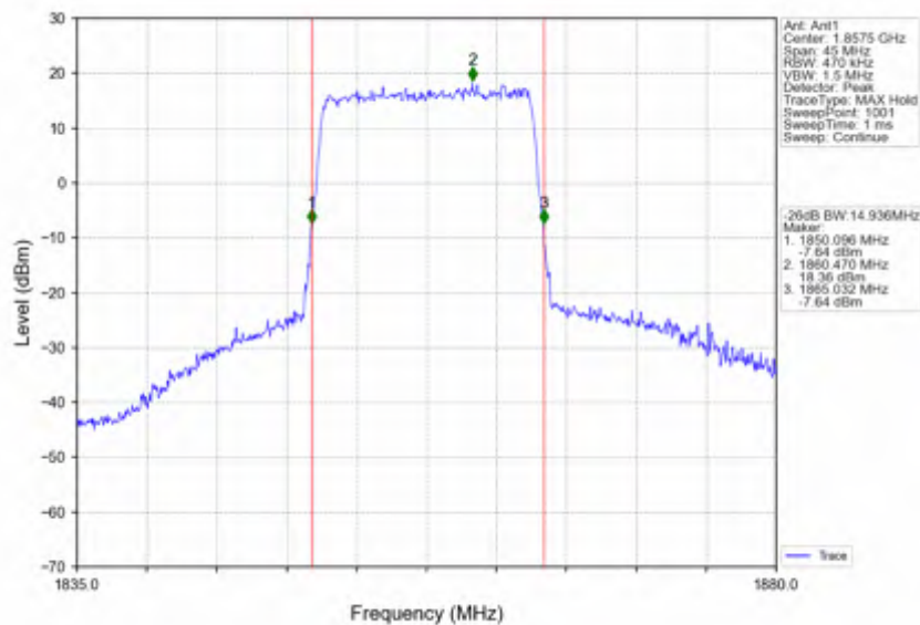
Band25_15MHz_16QAM_LCH_1857.5MHz_RB_75_0_NTNV
