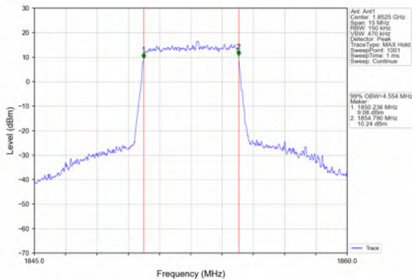
Band25_5MHz_256QAM_LCH_1852.5MHz_RB_25_0_NTNV
