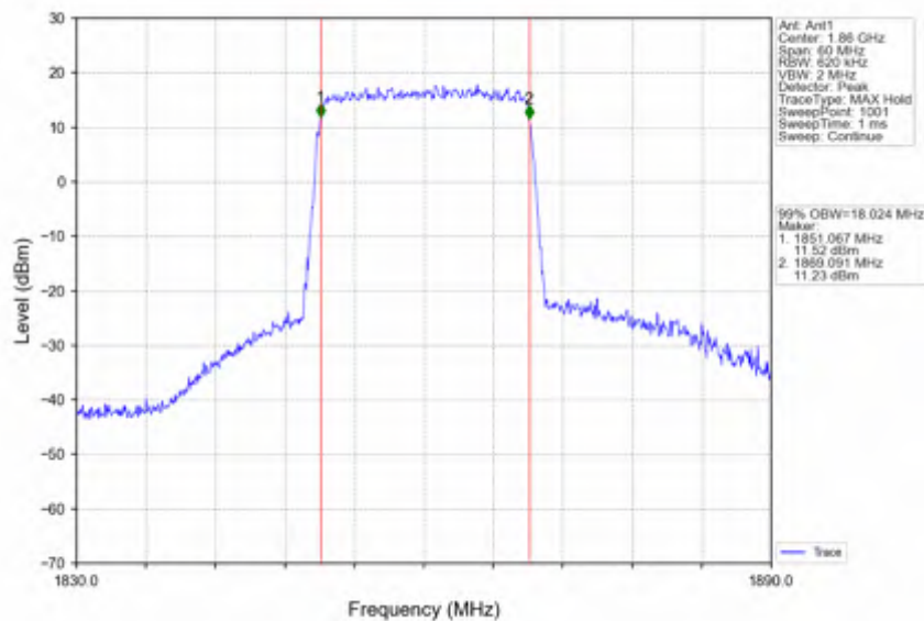
Band25_20MHz_16QAM_LCH_1860MHz_RB_100_0_NTNV
