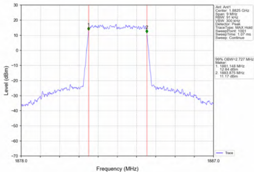
Band25_3MHz_QPSK_MCH_1882.5MHz_RB_15_0_NTNV
