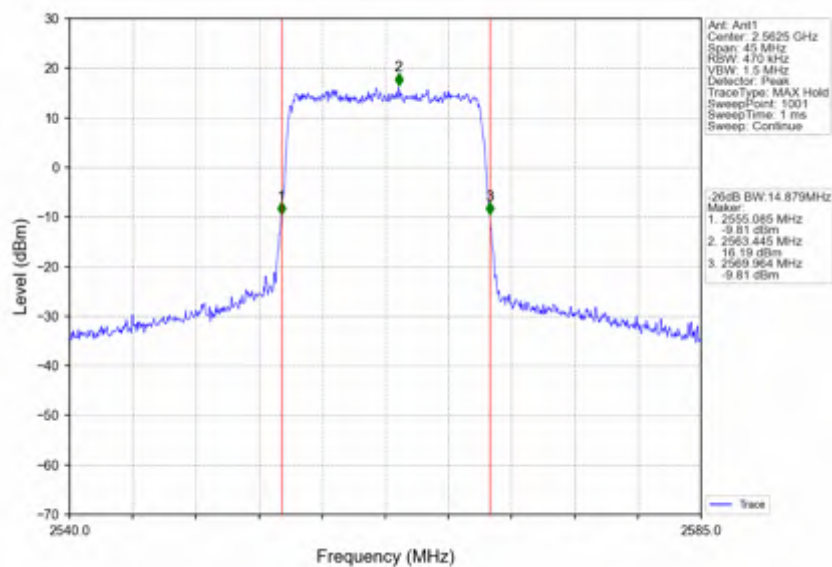
Band7_15MHz_256QAM_HCH_2562.5MHz_RB_75_0_NTNV
