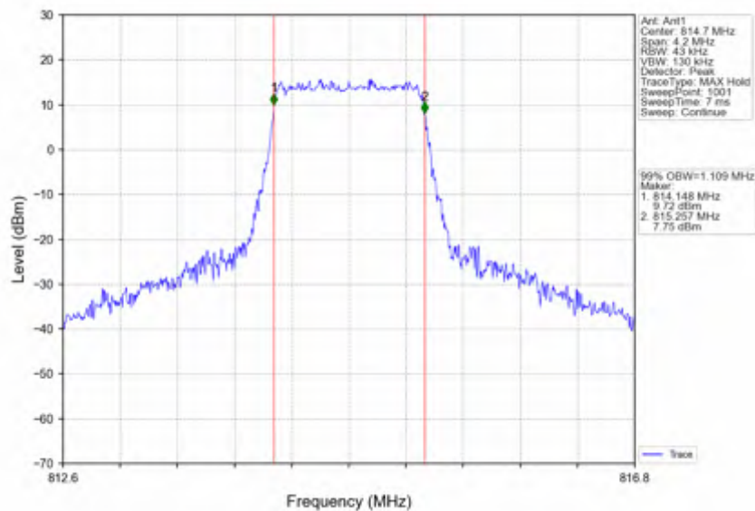
Band26a_1.4MHz_16QAM_LCH_814.7MHz_RB_6_0_NTNV
