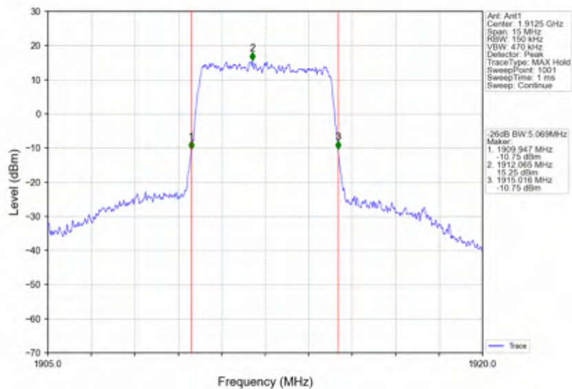
Band25_5MHz_256QAM_HCH_1912.5MHz_RB_25_0_NTNV
