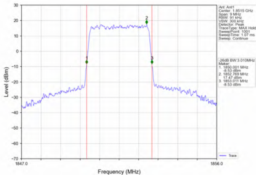
Band25_3MHz_16QAM_LCH_1851.5MHz_RB_15_0_NTNV
