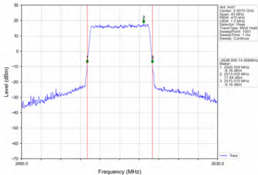
Band7_15MHz_16QAM_LCH_2507.5MHz_RB_75_0_NTNV
