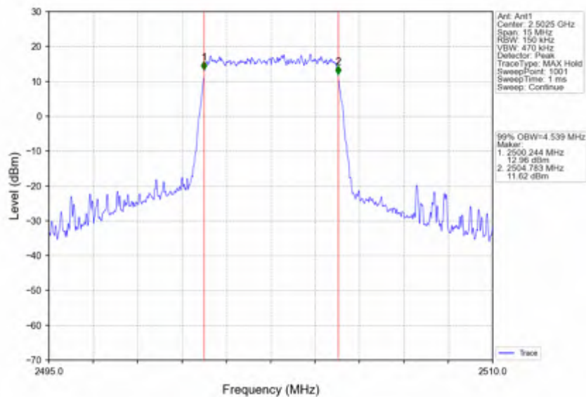
Band7_5MHz_16QAM_LCH_2502.5MHz_RB_25_0_NTNV
