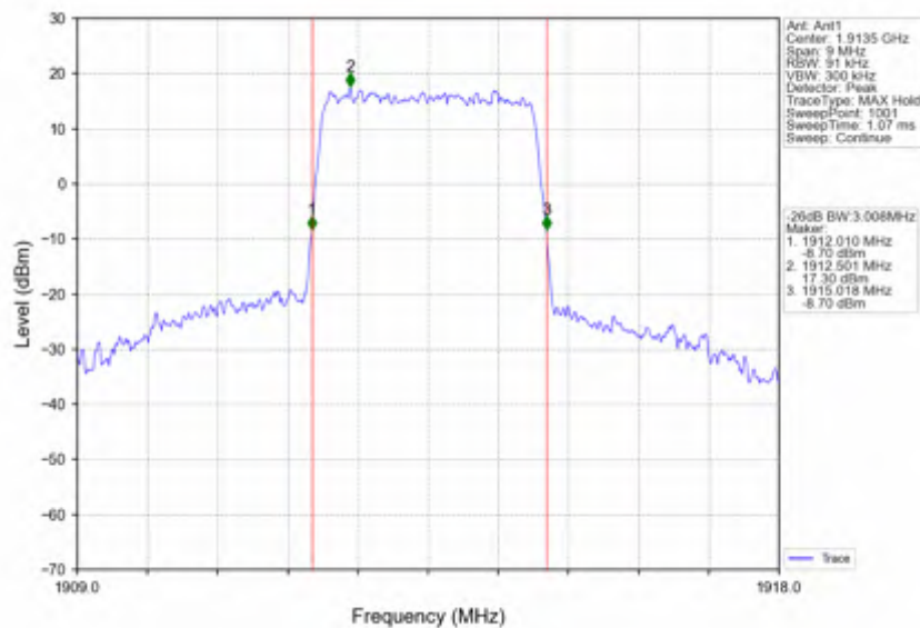
Band25_3MHz_16QAM_HCH_1913.5MHz_RB_15_0_NTNV
