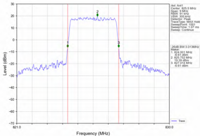
Band5_3MHz_16QAM_LCH_825.5MHz_RB_15_0_NTNV
