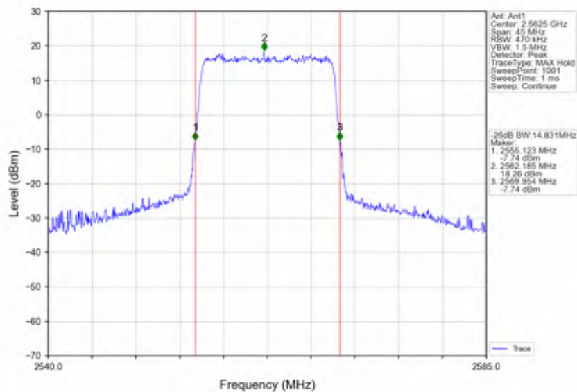
Band7_15MHz_16QAM_HCH_2562.5MHz_RB_75_0_NTNV
