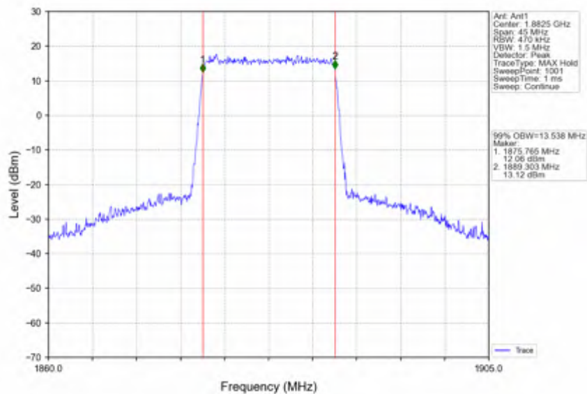
Band25_15MHz_QPSK_MCH_1882.5MHz_RB_75_0_NTNV
