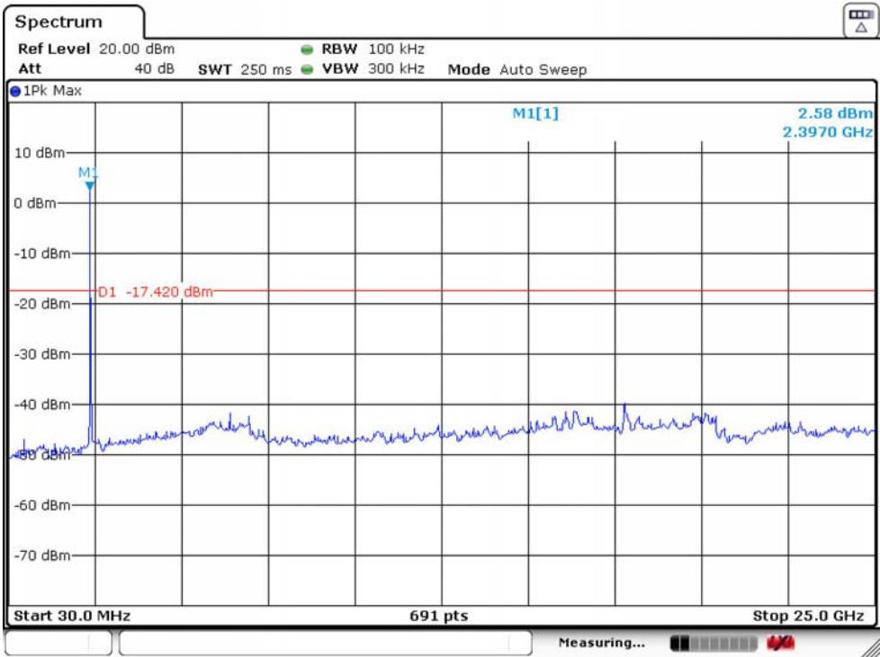
8-DPSK 2402 MHz
