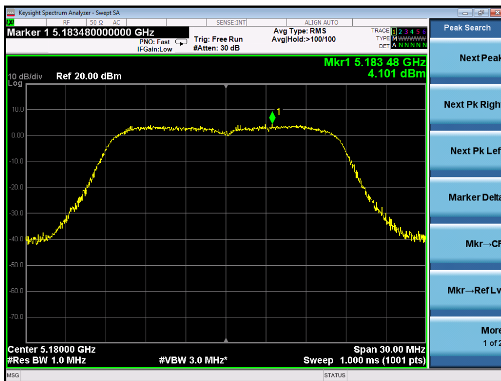
TEST PLOT OF SPECTRAL DENSITY FOR 5180MHz AT CHAIN 2
