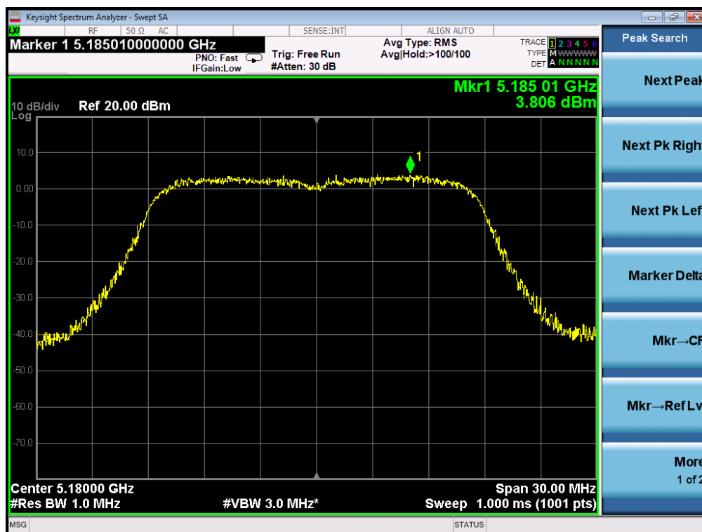
TEST PLOT OF SPECTRAL DENSITY FOR 5180MHz AT CHAIN 2
