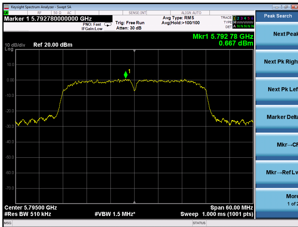
TEST PLOT OF SPECTRAL DENSITY FOR 5795MHz AT CHAIN 2
