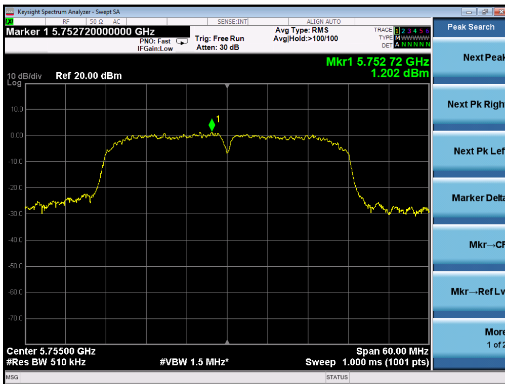
TEST PLOT OF SPECTRAL DENSITY FOR 5755MHz AT CHAIN 2
