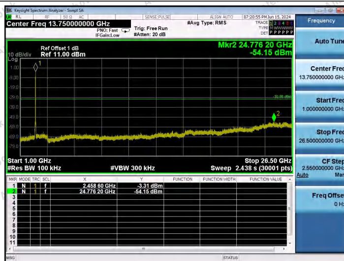
11N20SISO-Ant1-2462-1000~26500-PASS
