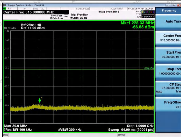
11N20SISO-Ant1-2462-30~1000-PASS
