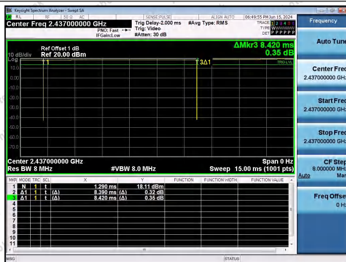
NTNV-11B-Ant1-2437
