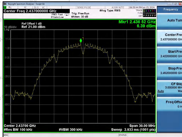
11B-Ant1-2437-0~Reference-PASS
