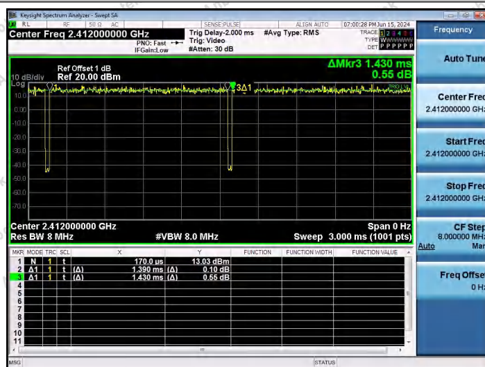
NTNV-11G-Ant1-2412
