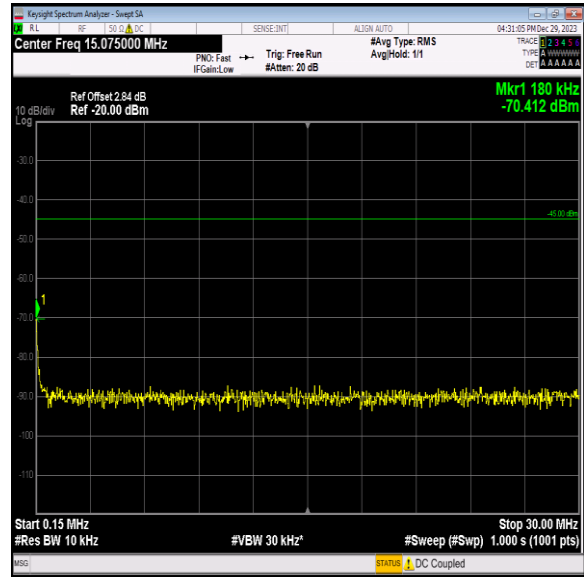
Band7_15MHz_QPSK_21375_1RB#0_0.15~30_0.15~30
