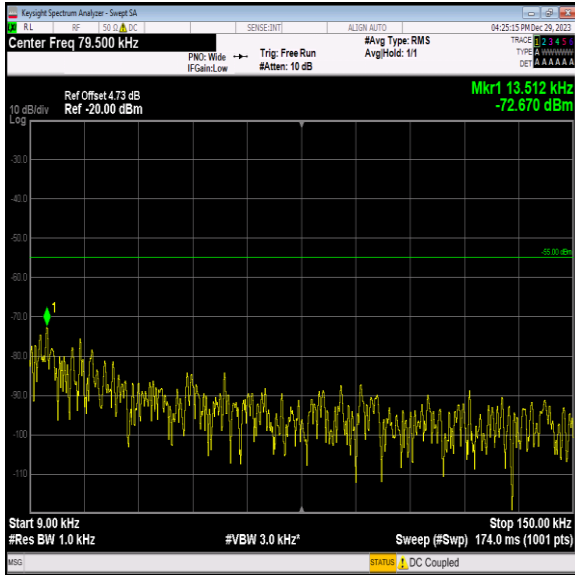
Band7_15MHz_QPSK_20825_1RB#0_0.009~0.15_0.009~0.15 5
