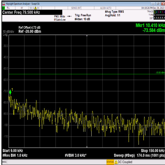
Band7_10MHz_16QAM_21400_1RB#0_0.009~0.15_0.009~0.15
