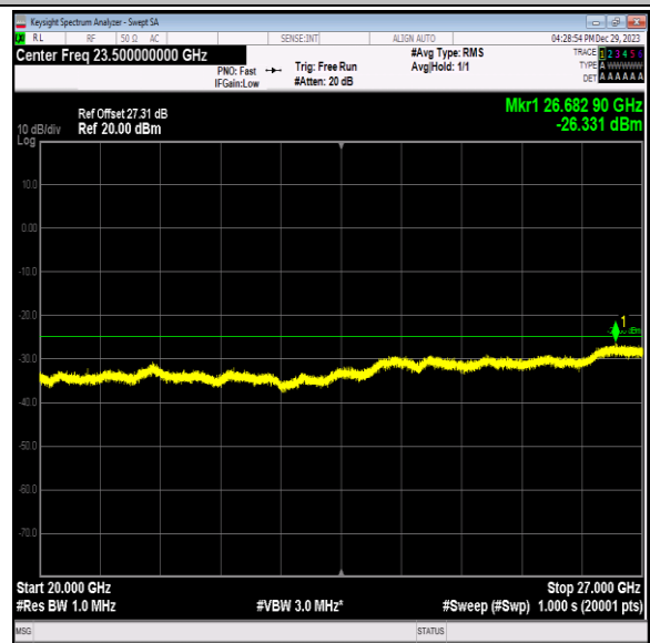
Band7_15MHz_QPSK_21100_1RB#0_20000~27000_20000~27000
