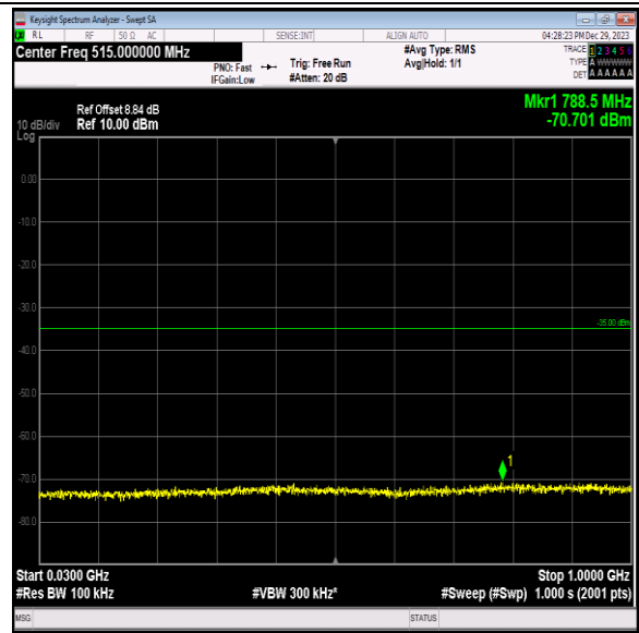
Band7_15MHz_QPSK_21100_1RB#0_30~1000_30~1000
