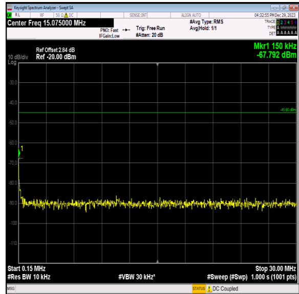
Band7_15MHz_64QAM_21375_1RB#0_0.15~30_0.15~30
