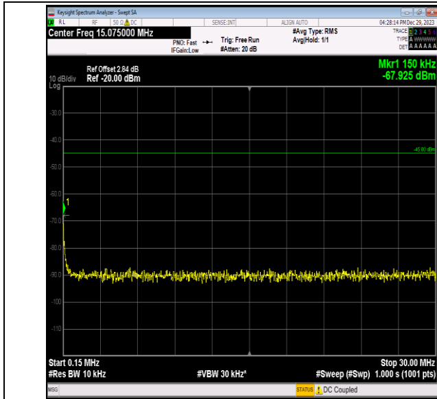
Band7_15MHz_QPSK_21100_1RB#0_0.15~30_0.15~30
