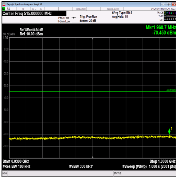
Band7_15MHz_16QAM_21100_1RB#0_30~1000_30~1000
