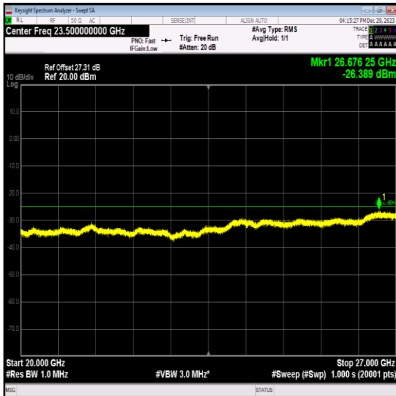
Band7_10MHz_QPSK_21100_1RB#0_20000~27000_20000~27000
