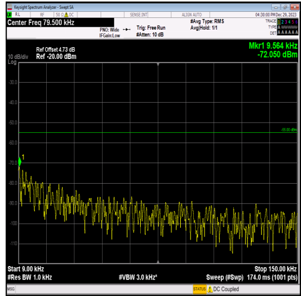
Band7_15MHz_64QAM_21100_1RB#0_0.009~0.15_0.009~0.15
