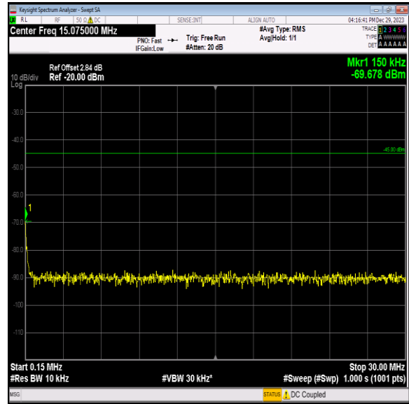
Band7_10MHz_64QAM_21100_1RB#0_0.15~30_0.15~30
