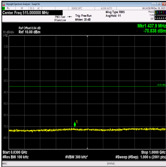
Band7_10MHz_QPSK_21100_1RB#0_30~1000_30~1000
