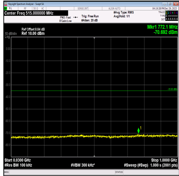
Band7_10MHz_64QAM_21400_1RB#0_30~1000_30~1000
