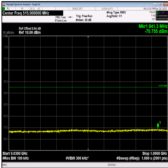
Band7_5MHz_64QAM_21425_1RB#0_30~1000_30~1000
