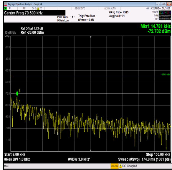
Band7_10MHz_64QAM_21400_1RB#0_0.009~0.15_0.009~0.15
