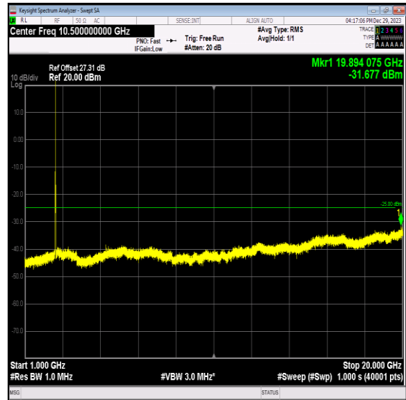
Band7_10MHz_64QAM_21100_1RB#0_1000~20000_1000~20000
