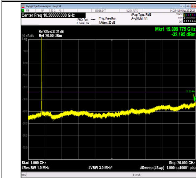
Band7_15MHz_QPSK_21100_1RB#0_1000~20000_1000~20000
