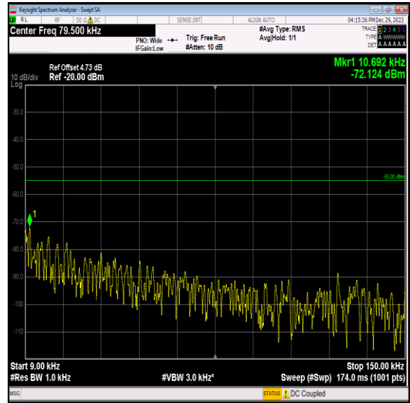
Band7_10MHz_16QAM_21100_1RB#0_0.009~0.15_0.009~0. 15
