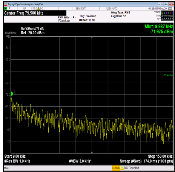
Band7_15MHz_16QAM_20825_1RB#0_0.009~0.15_0.009~0.15
