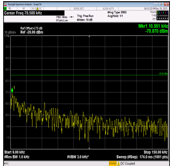
Band7_15MHz_16QAM_21375_1RB#0_0.009~0.15_0.009~0.15
