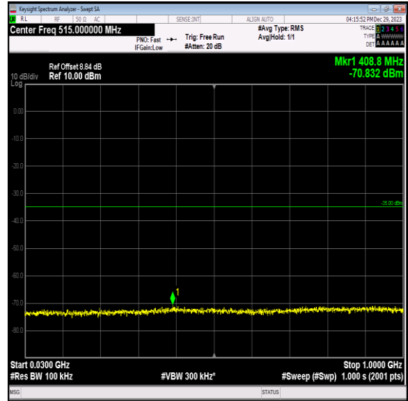
Band7_10MHz_16QAM_21100_1RB#0_30~1000_30~1000
