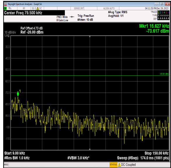
Band7_10MHz_QPSK_20800_1RB#0_0.009~0.15_0.009~0.1 5
