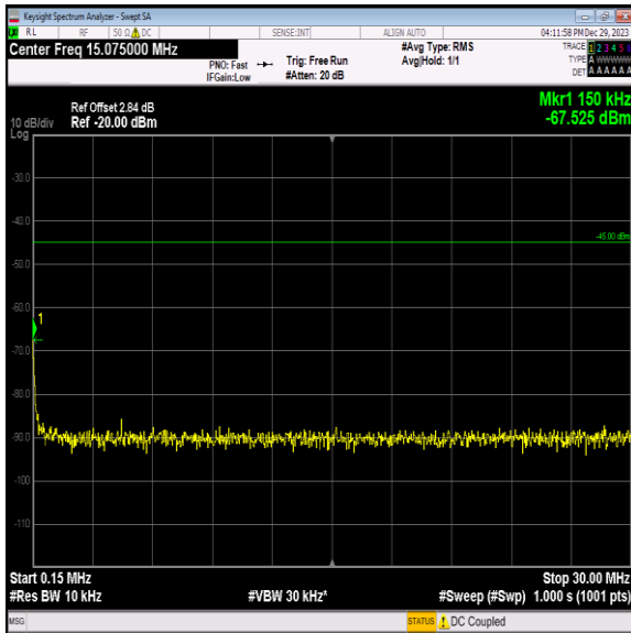
Band7_10MHz_QPSK_20800_1RB#0_0.15~30_0.15~30
