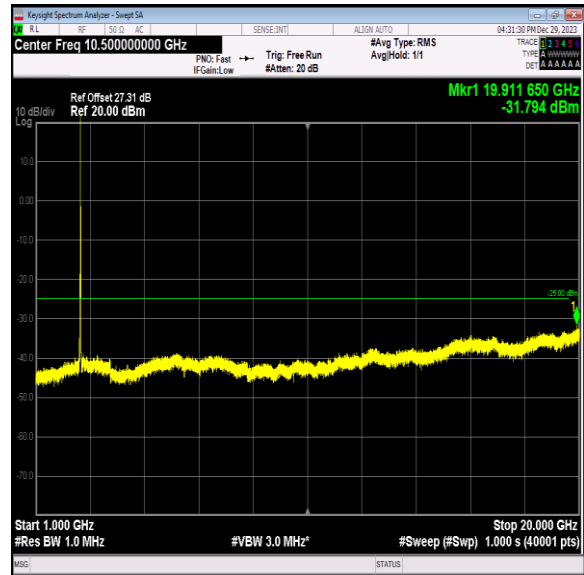
Band7_15MHz_QPSK_21375_1RB#0_1000~20000_1000~20 000
