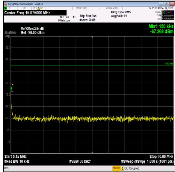
Band7_15MHz_QPSK_20825_1RB#0_0.15~30_0.15~30
