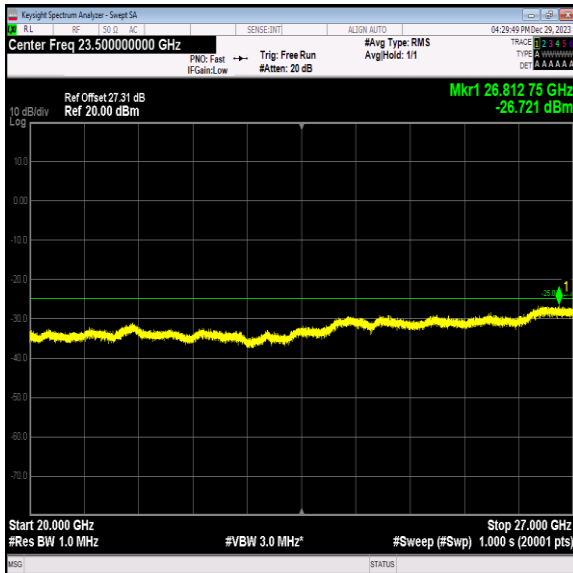
Band7_15MHz_16QAM_21100_1RB#0_20000~27000_20000~27000
