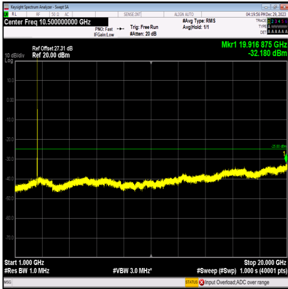
Band7_10MHz_64QAM_21400_1RB#0_1000~20000_1000~20000 0000
