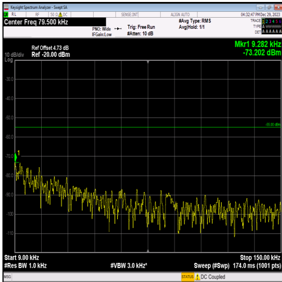
Band7_15MHz_64QAM_21375_1RB#0_0.009~0.15_0.009~0.15
