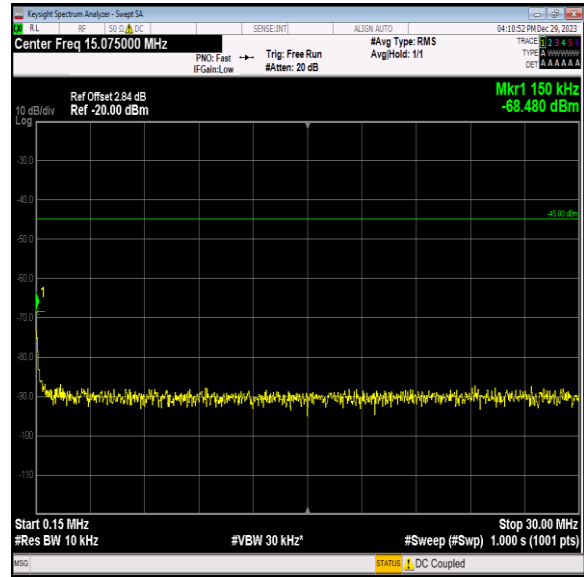
Band7_5MHz_64QAM_21425_1RB#0_0.15~30_0.15~30
