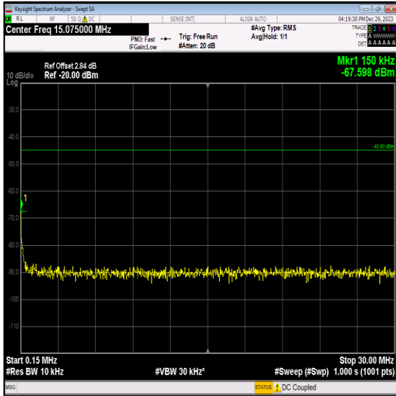
Band7_10MHz_64QAM_21400_1RB#0_0.15~30_0.15~30
