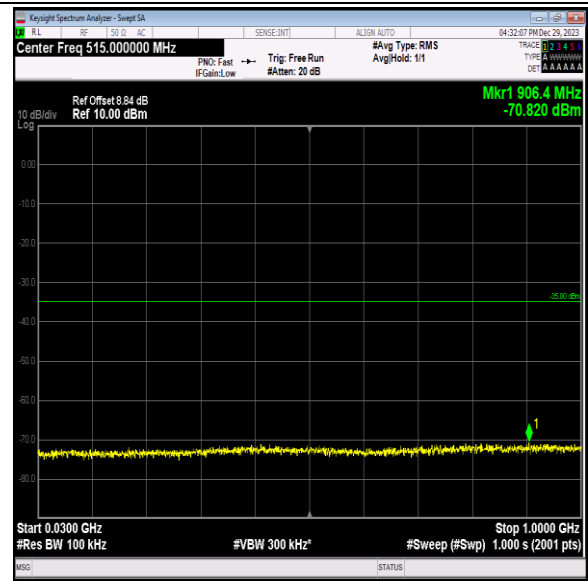
Band7_15MHz_16QAM_21375_1RB#0_30~1000_30~1000
