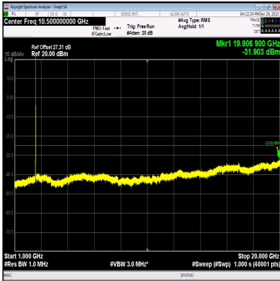
Band7_10MHz_QPSK_20800_1RB#0_1000~20000_1000~20000
