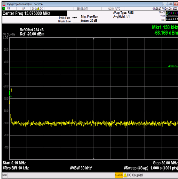
Band7_15MHz_16QAM_20825_1RB#0_0.15~30_0.15~30
