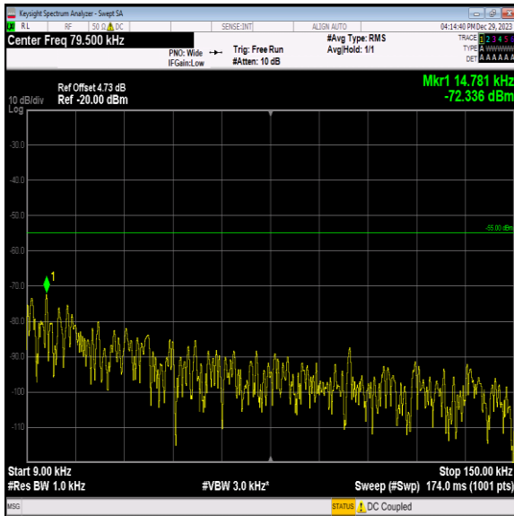
Band7_10MHz_QPSK_21100_1RB#0_0.009~0.15_0.009~0.15
