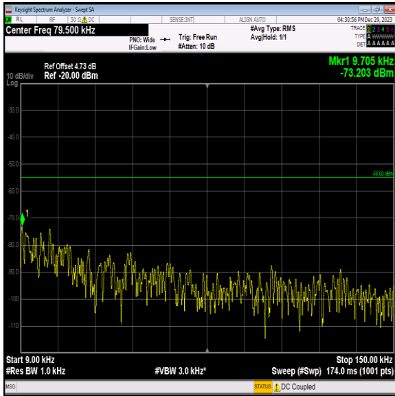
Band7_15MHz_QPSK_21375_1RB#0_0.009~0.15_0.009~0.1 5
