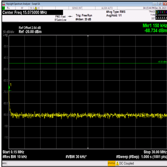
Band7_10MHz_16QAM_21100_1RB#0_0.15~30_0.15~30
