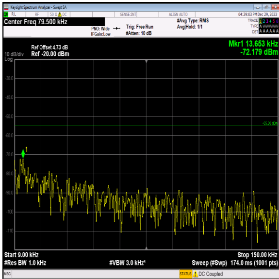
Band7_15MHz_16QAM_21100_1RB#0_0.009~0.15_0.009~0.15 15
