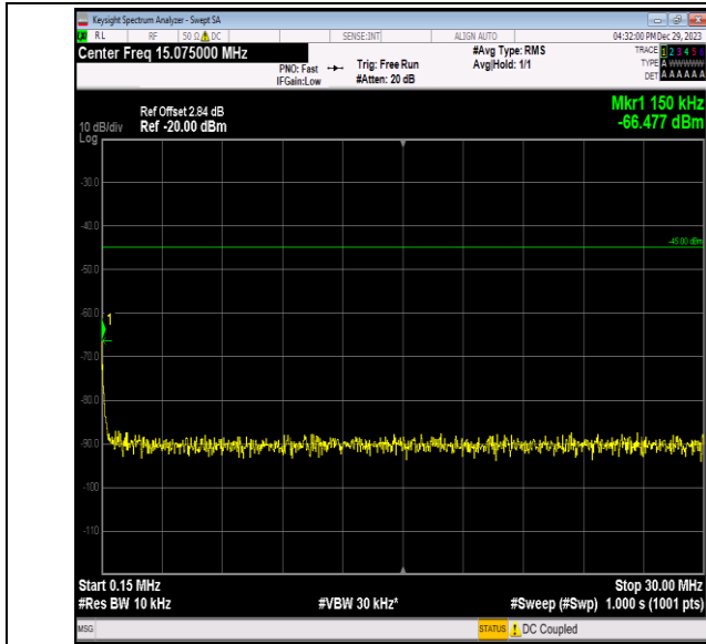
Band7_15MHz_16QAM_21375_1RB#0_0.15~30_0.15~30
