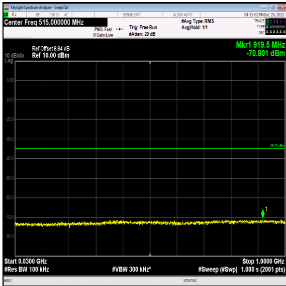
Band7_10MHz_16QAM_20800_1RB#0_30~1000_30~1000
