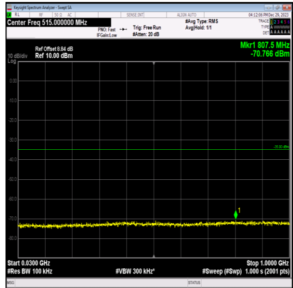
Band7_10MHz_QPSK_20800_1RB#0_30~1000_30~1000
