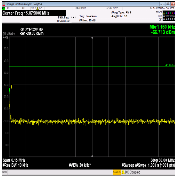
Band7_15MHz_64QAM_21100_1RB#0_0.15~30_0.15~30
