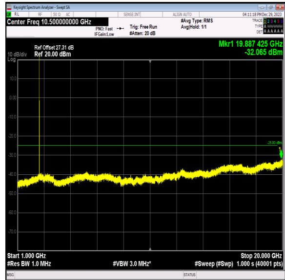
Band7_5MHz_64QAM_21425_1RB#0_1000~20000_1000~20 000
