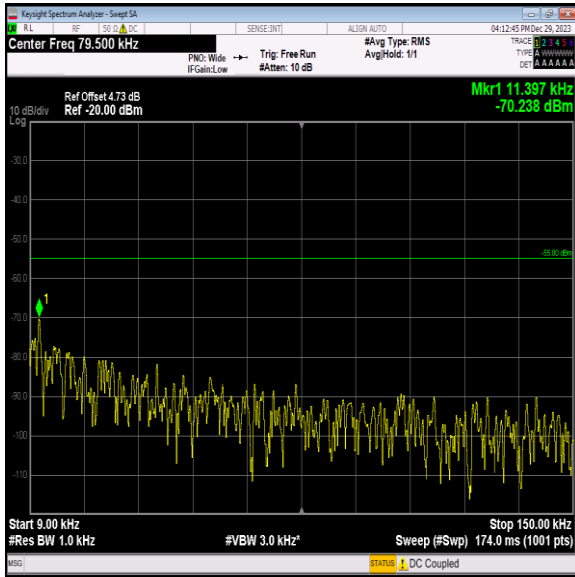
Band7_10MHz_16QAM_20800_1RB#0_0.009~0.15_0.009~0.15
