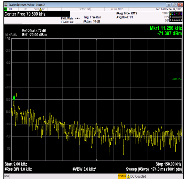
Band7_10MHz_64QAM_20800_1RB#0_0.009~0.15_0.009~0.15
