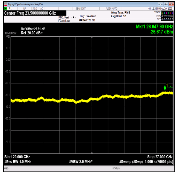
Band7_10MHz_QPSK_20800_1RB#0_20000~27000_20000~27000
