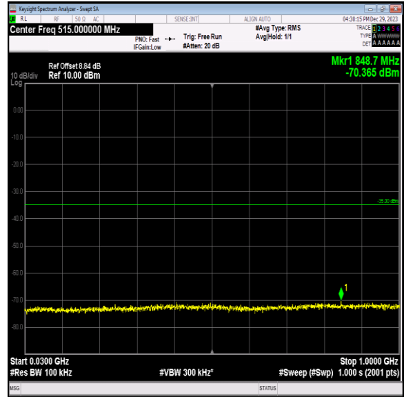
Band7_15MHz_64QAM_21100_1RB#0_30~1000_30~1000
