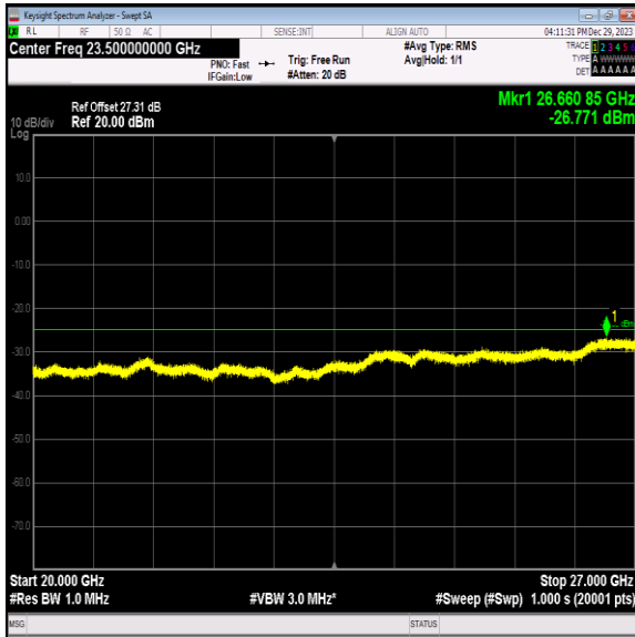
Band7_5MHz_64QAM_21425_1RB#0_20000~27000_20000~27000
