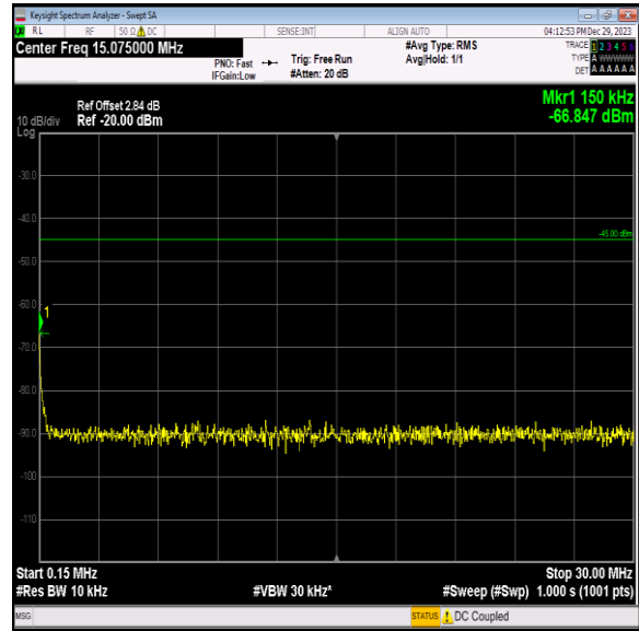
Band7_10MHz_16QAM_20800_1RB#0_0.15~30_0.15~30
