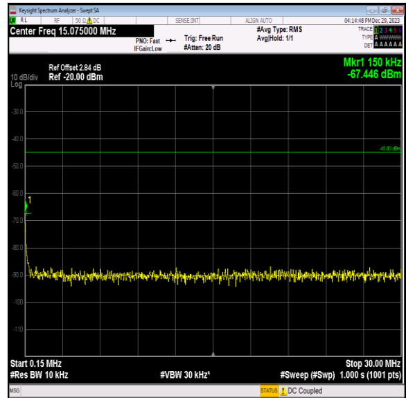
Band7_10MHz_QPSK_21100_1RB#0_0.15~30_0.15~30
