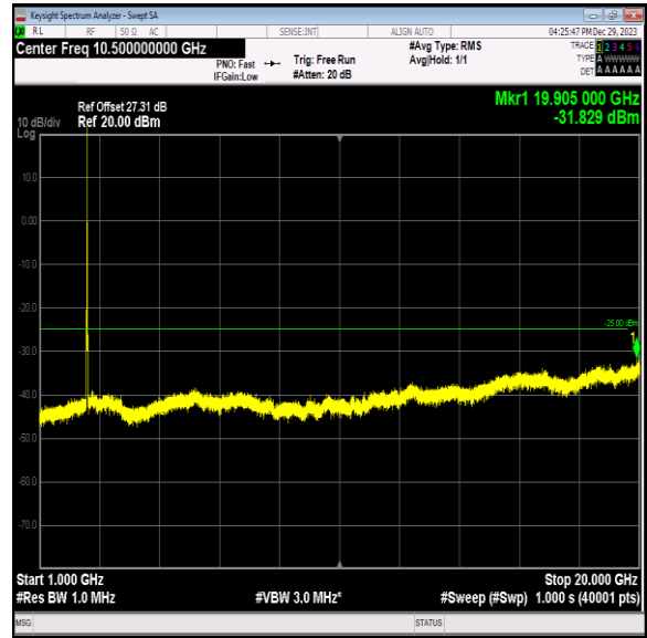
Band7_15MHz_QPSK_20825_1RB#0_1000~20000_1000~20000
