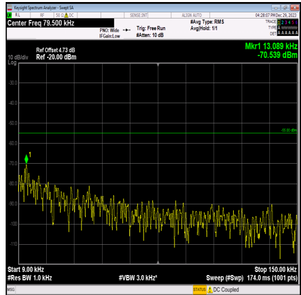
Band7_15MHz_QPSK_21100_1RB#0_0.009~0.15_0.009~0.15
