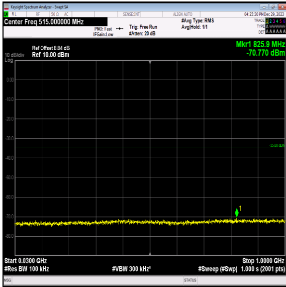
Band7_15MHz_QPSK_20825_1RB#0_30~1000_30~1000
