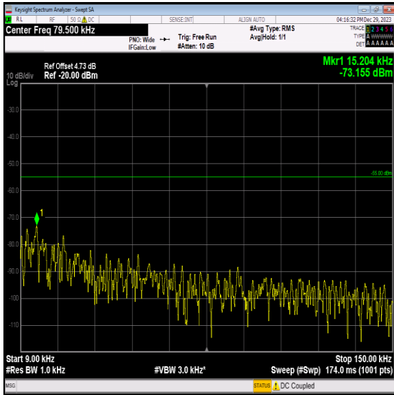
Band7_10MHz_64QAM_21100_1RB#0_0.009~0.15_0.009~0.15
