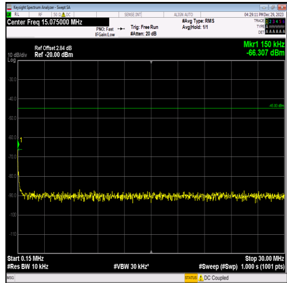
Band7_15MHz_16QAM_21100_1RB#0_0.15~30_0.15~30
