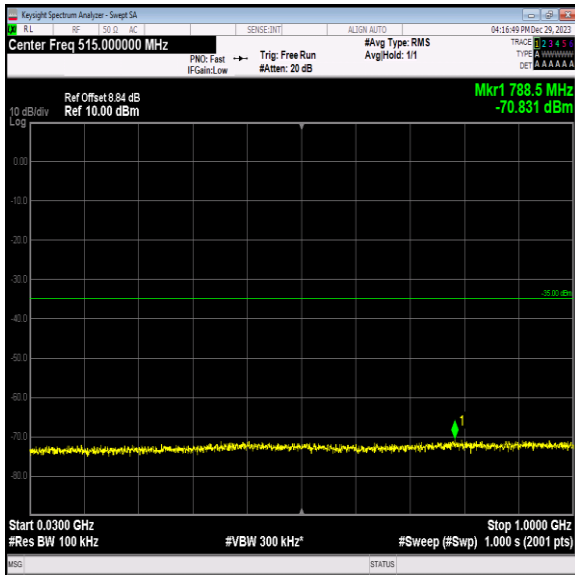
Band7_10MHz_64QAM_21100_1RB#0_30~1000_30~1000
