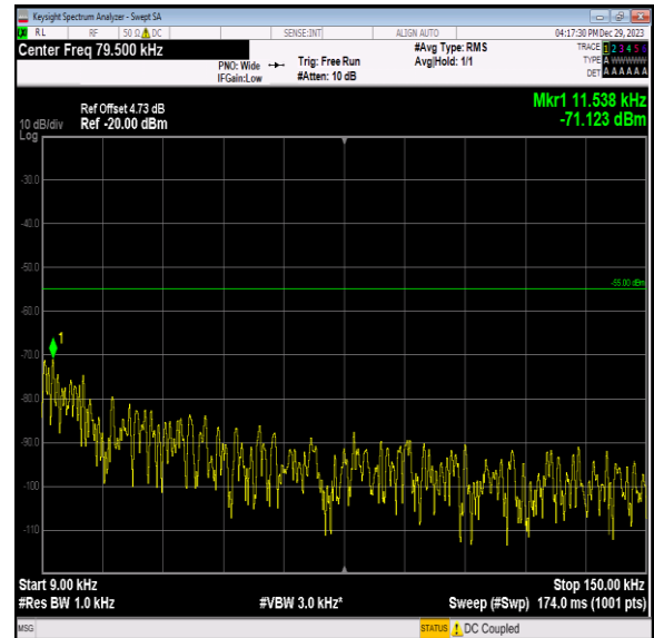
Band7_10MHz_QPSK_21400_1RB#0_0.009~0.15_0.009~0.15
