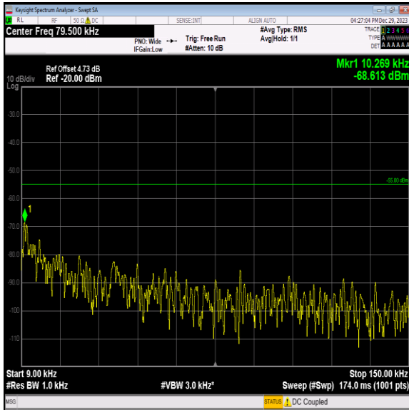
Band7_15MHz_64QAM_20825_1RB#0_0.009~0.15_0.009~0.15
