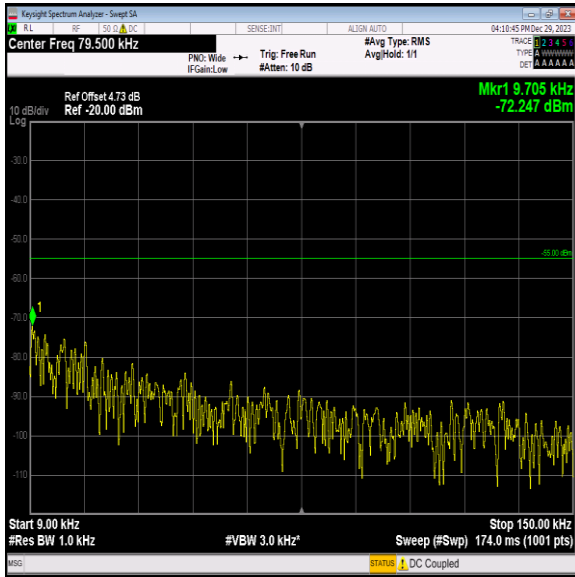
Band7_5MHz_64QAM_21425_1RB#0_0.009~0.15_0.009~0.1 5
