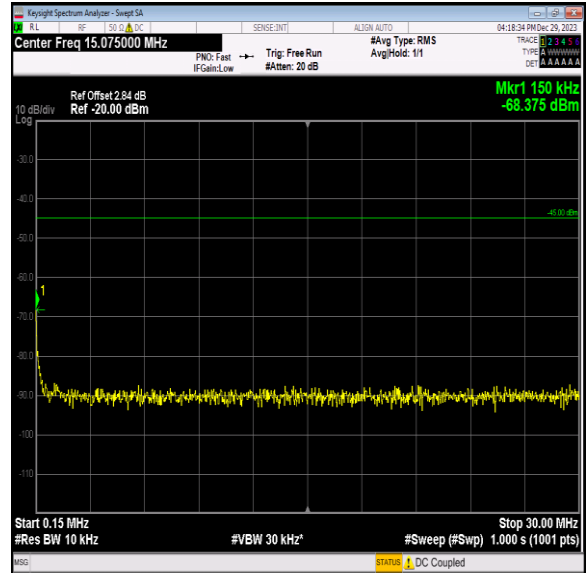
Band7_10MHz_16QAM_21400_1RB#0_0.15~30_0.15~30
