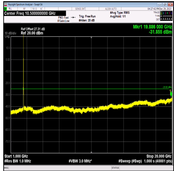
Band7_15MHz_64QAM_20825_1RB#0_1000~20000_1000~20000
