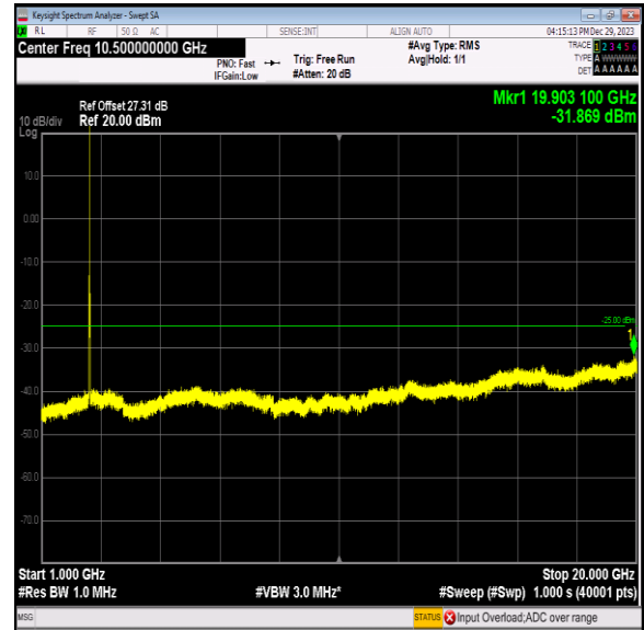
Band7_10MHz_QPSK_21100_1RB#0_1000~20000_1000~20000
