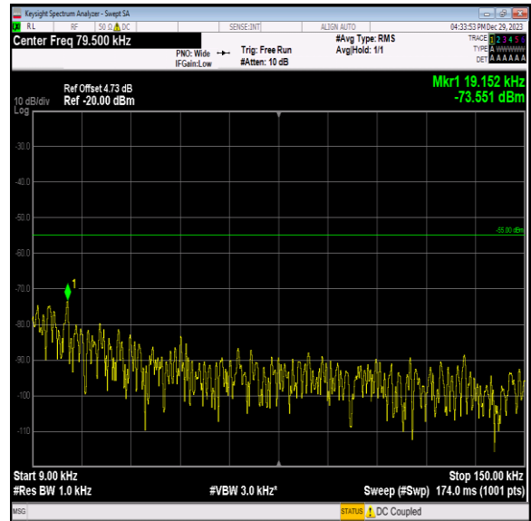
Band7_20MHz_QPSK_20850_1RB#0_0.009~0.15_0.009~0.15
