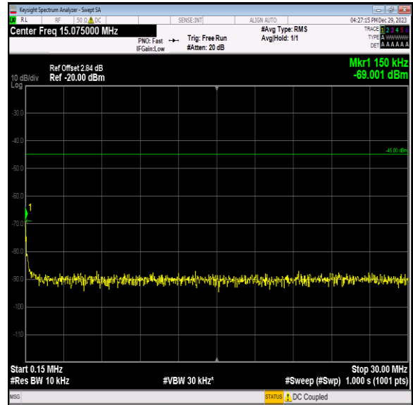
Band7_15MHz_64QAM_20825_1RB#0_0.15~30_0.15~30
