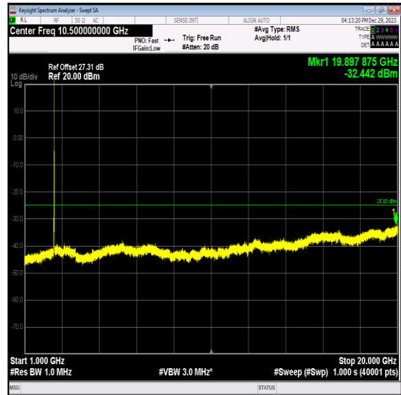
Band7_10MHz_16QAM_20800_1RB#0_1000~20000_1000~20000
