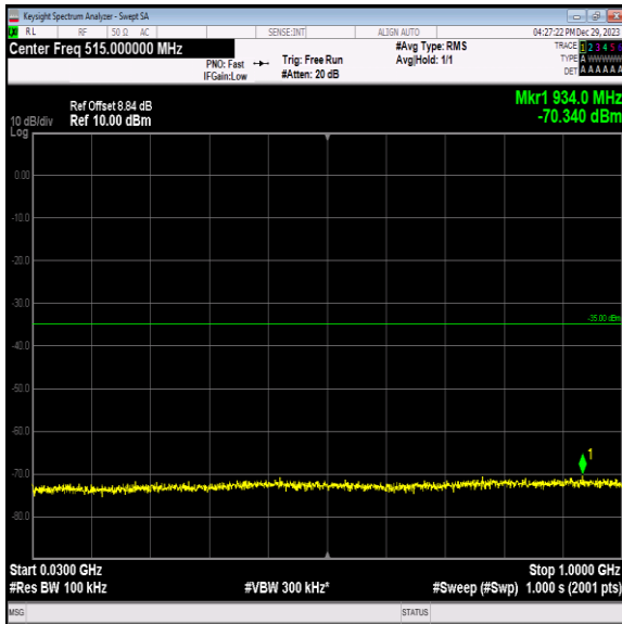
Band7_15MHz_64QAM_20825_1RB#0_30~1000_30~1000
