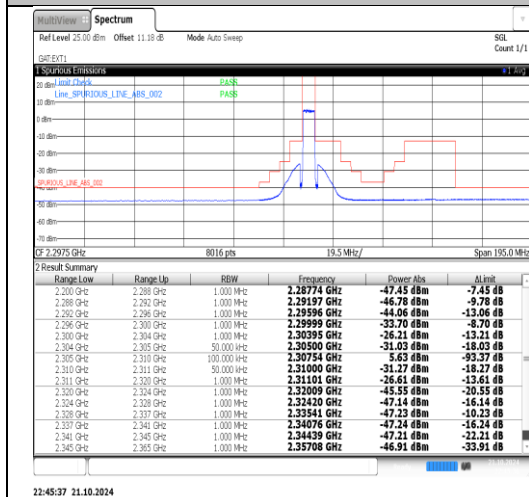
Band40(2305-2315)-5MHz-16QAM-38775-1RB#0-PASS
