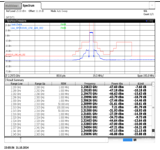
Band40(2305-2315)-5MHz-16QAM-38725-1RB#0-PASS
