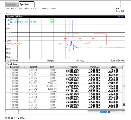
Band40(2305-2315)-5MHz-QPSK-38775-25RB#0-PASS
