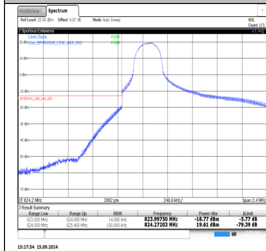
Band5-1.4MHz-16QAM-20407-1RB#5-PASS
