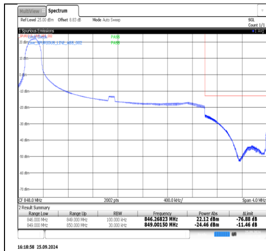
Band5-3MHz-QPSK-20635-1RB#14-Pre-scan
