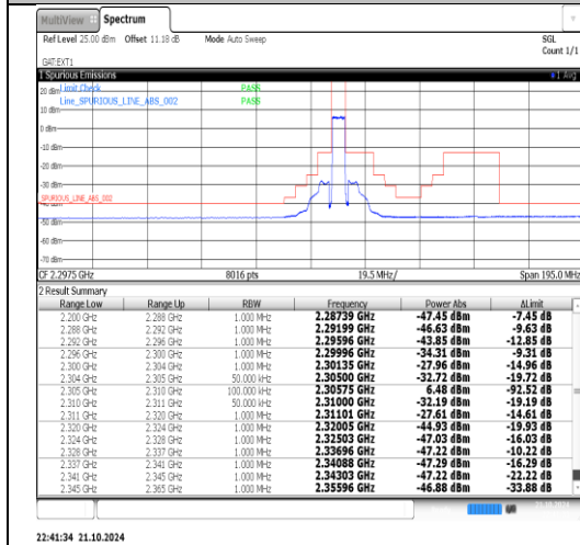
Band40(2305-2315)-5MHz-QPSK-38775-1RB#0-PASS
