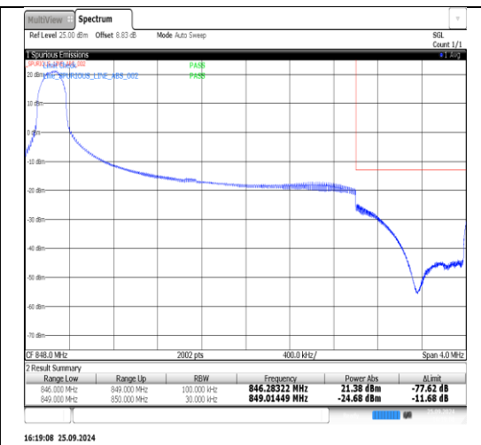
Band5-3MHz-16QAM-20635-1RB#14-Pre-scan
