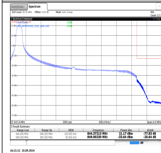
Band5-5MHz-16QAM-20625-1RB#24-PASS
