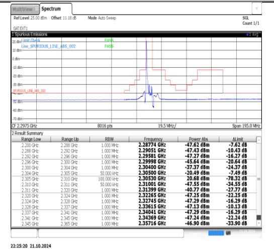
Band40(2305-2315)-5MHz-QPSK-38725-1RB#24-PASS
