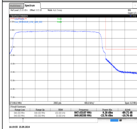
Band5-3MHz-16QAM-20635-1RB#14- PASS_Final1
