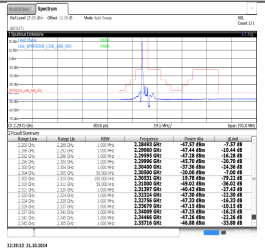
Band40(2305-2315)-5MHz-16QAM-38725-1RB#24-PASS
