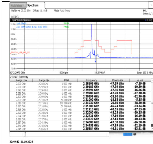
Band40(2305-2315)-5MHz-QPSK-38775-1RB#24-PASS
