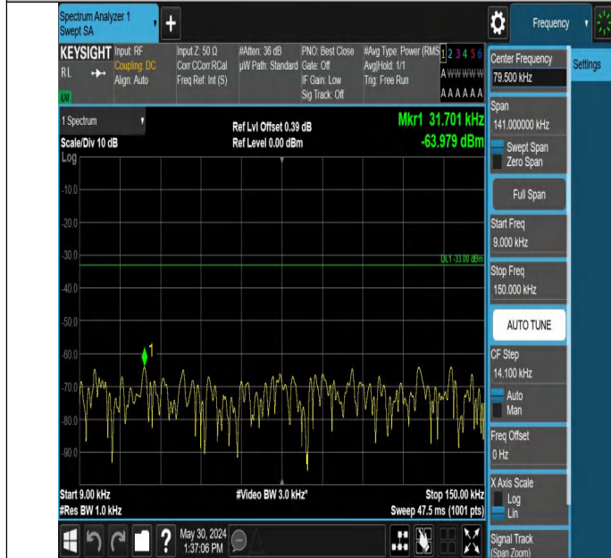
Band13_10MHz_QPSK_23230_1RB#0_0.009~0.15_0.009~0.15
