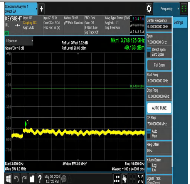
Band13_10MHz_QPSK_23230_1RB#0_3000~10000_3000~10000
