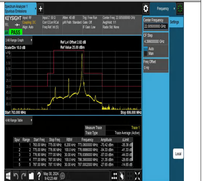
Band13_10MHz_QPSK_23230_1RB#49
