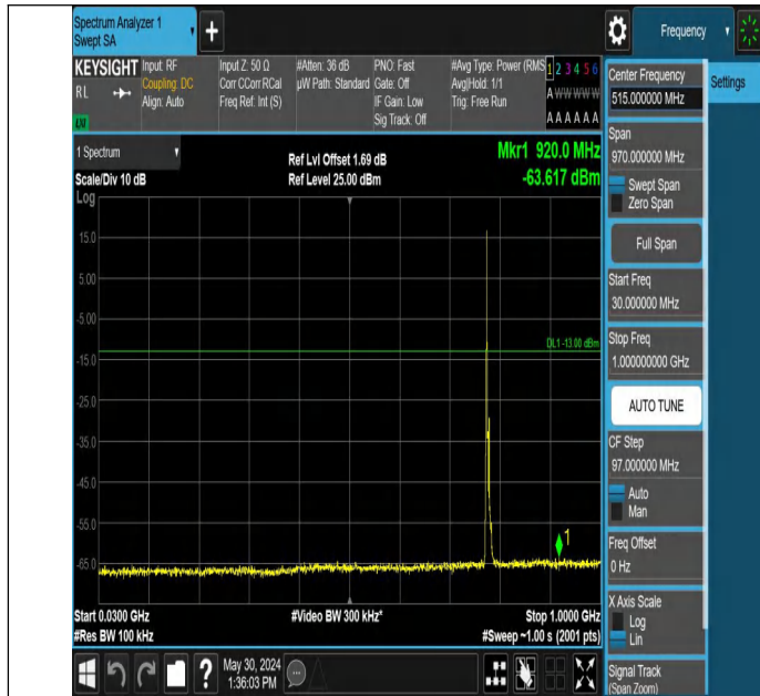
Band13_5MHz_QPSK_23230_1RB#0_30~1000_30~1000
