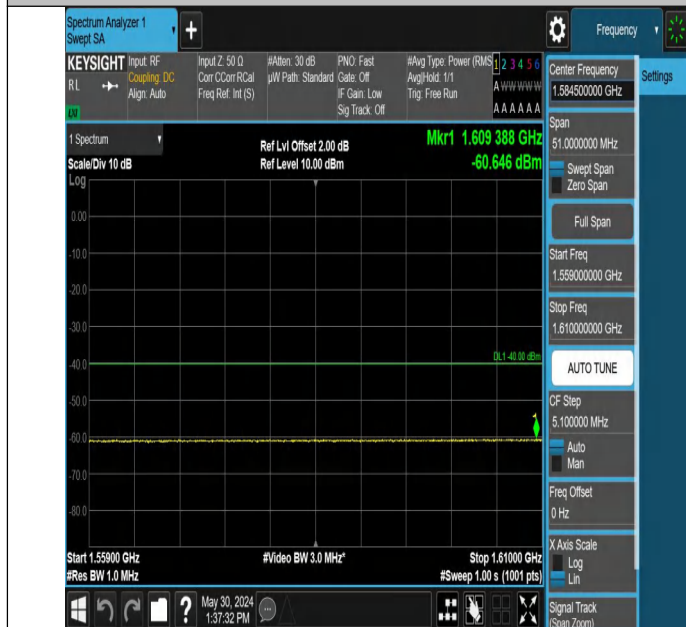
Band13_10MHz_QPSK_23230_1RB#0_1559~1610_1559~1610
