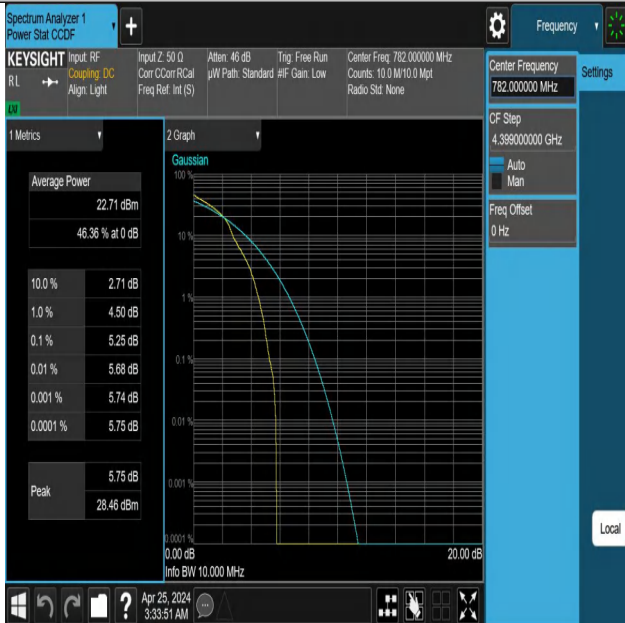
Band13-10MHz-16QAM-23230-1RB#0-PASS
