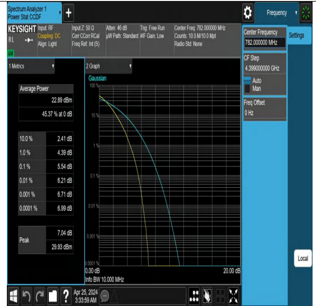
Band13-10MHz-QPSK-23230-50RB#0-PASS
