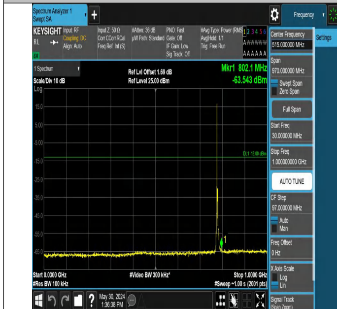
Band13_5MHz_QPSK_23255_1RB#0_30~1000_30~1000
