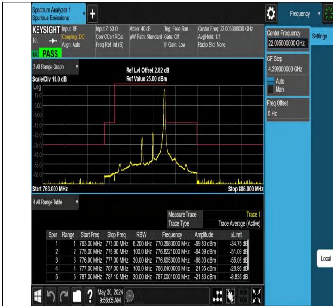
Band13_5MHz_QPSK_23255_1RB#24
