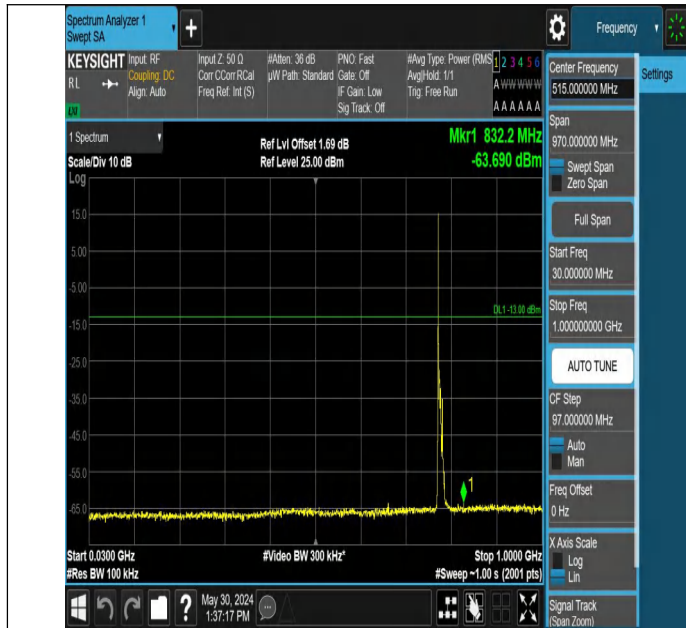
Band13_10MHz_QPSK_23230_1RB#0_30~1000_30~1000
