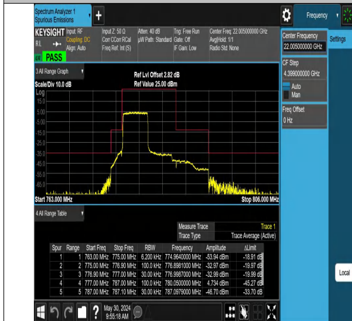
Band13_5MHz_QPSK_23205_25RB#0
