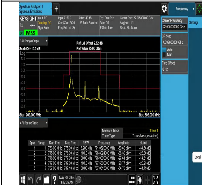
Band13_10MHz_QPSK_23230_1RB#0
