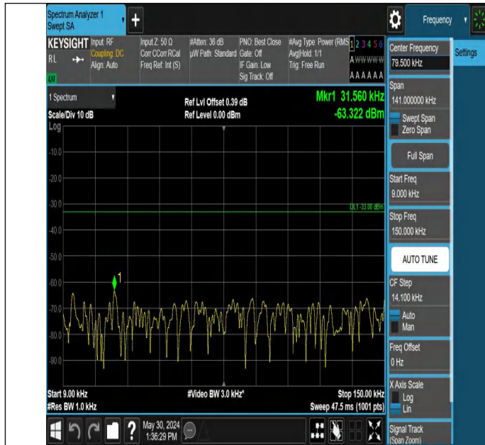
Band13_5MHz_QPSK_23255_1RB#0_0.009~0.15_0.009~0.15
