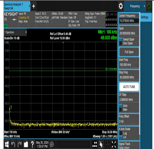
Band13_5MHz_QPSK_23230_1RB#0_0.15~30_0.15~30
