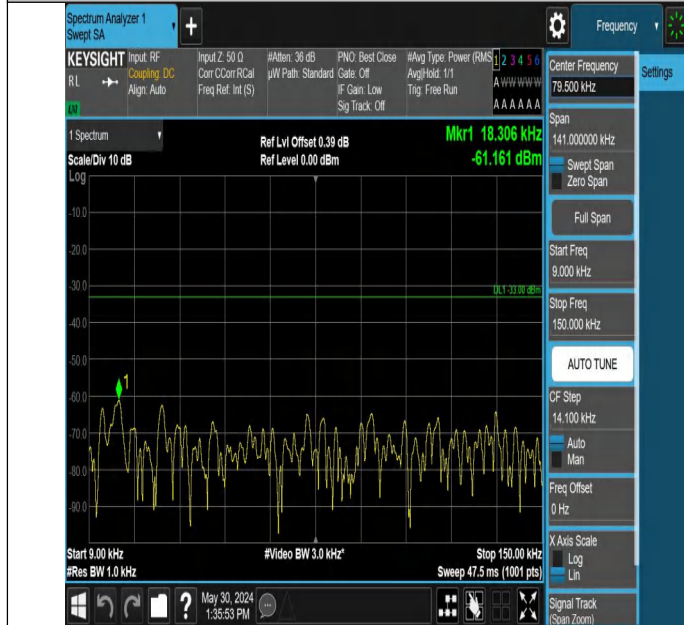
Band13_5MHz_QPSK_23230_1RB#0_0.009~0.15_0.009~0.15
