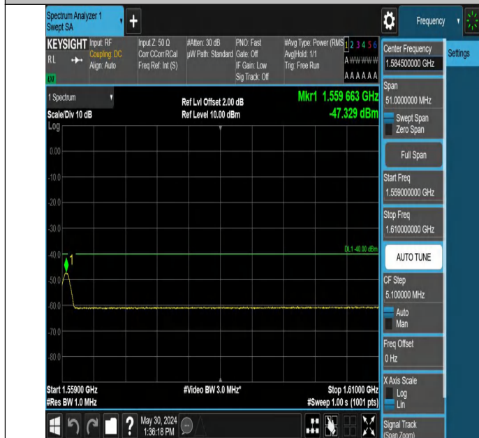
Band13_5MHz_QPSK_23230_1RB#0_1559~1610_1559~1610
