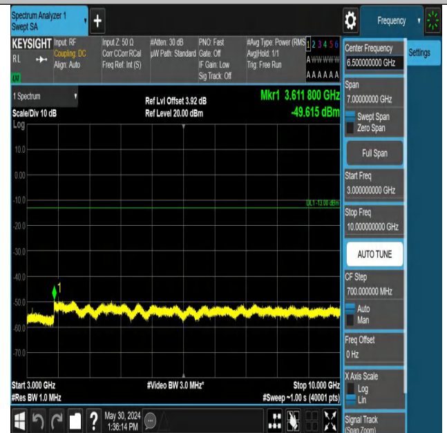
Band13_5MHz_QPSK_23230_1RB#0_3000~10000_3000~10000
