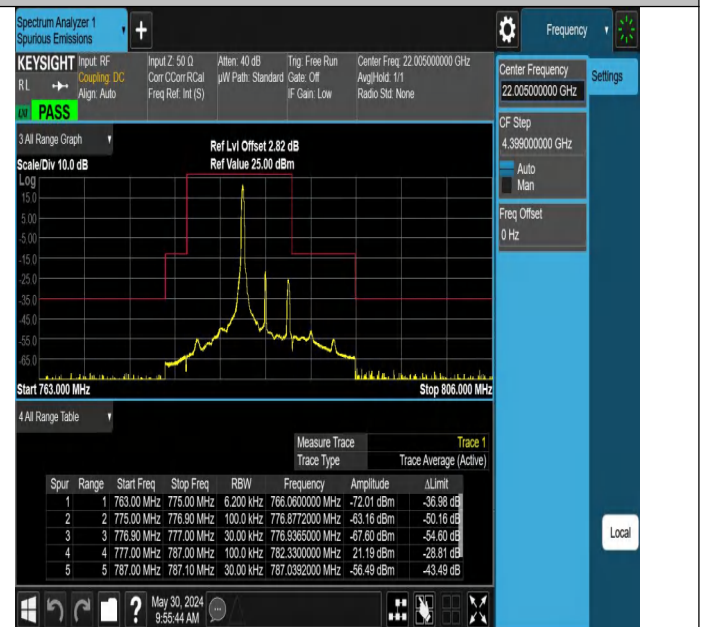
Band13_5MHz_QPSK_23255_1RB#0
