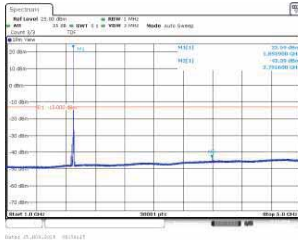
Band2_15MHz_16QAM_19125_1RB#0
