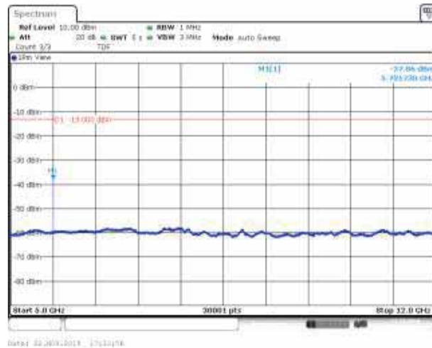
Band2_10MHz_16QAM_19150_1RB#0
