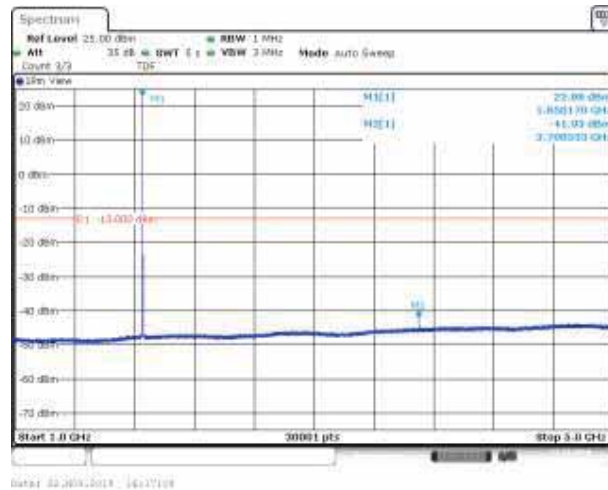
Band2_3MHz_16QAM_18615_1RB#0
