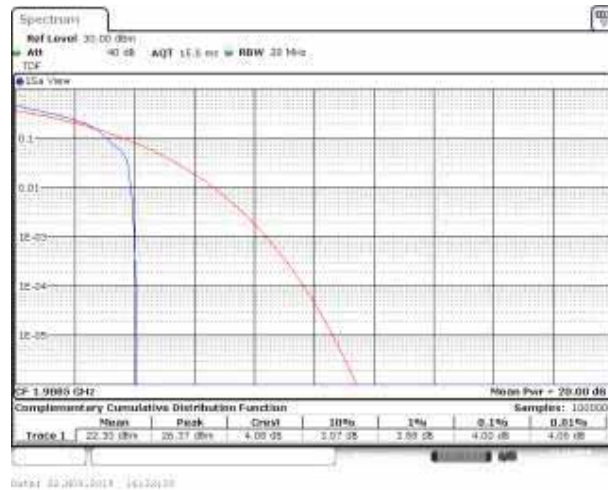
Band2_3MHz_16QAM_19185_15RB#0
