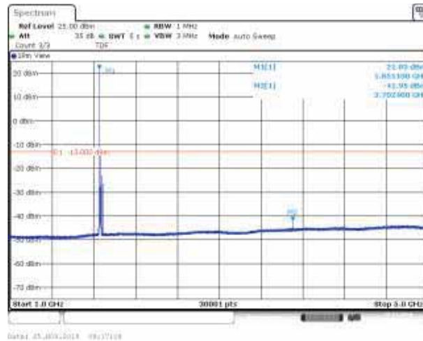
Band2_20MHz_16QAM_18700_1RB#0
