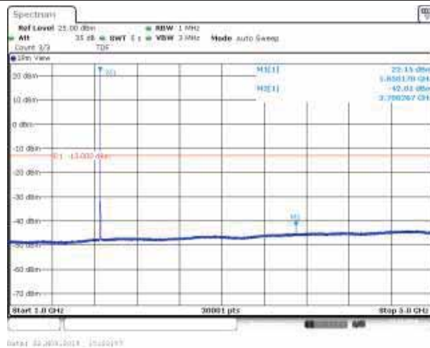
Band2_1.4MHz_16QAM_18607_1RB#0
