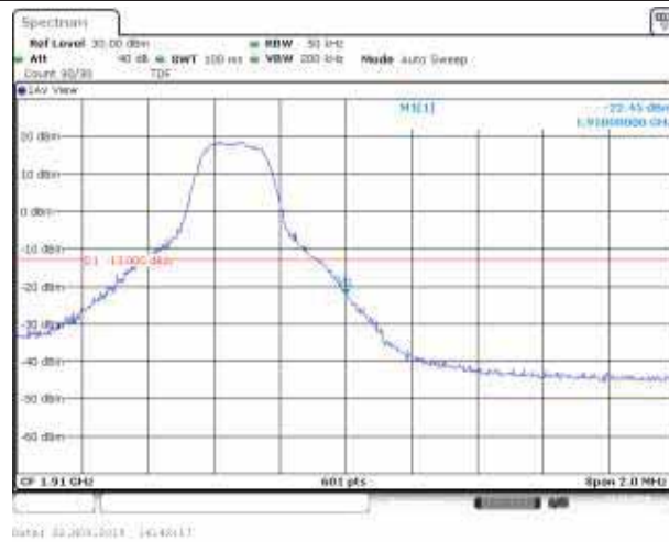
Band2_5MHz_QPSK_19175_25RB#0
