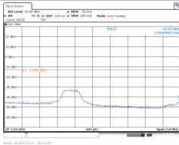
Band2_3MHz_16QAM_19185_1RB#14
