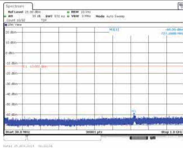
Band2_20MHz_16QAM_18900_1RB#0
