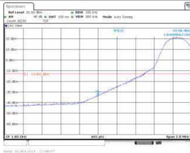
Band2_15MHz_QPSK_18675_1RB#74
