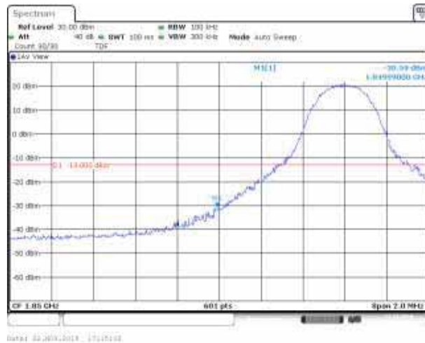
Band2_10MHz_16QAM_18650_1RB#49
