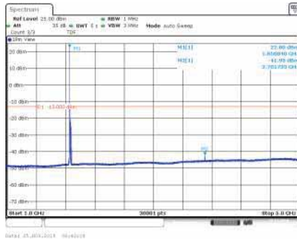
Band2_15MHz_QPSK_18675_1RB#0
