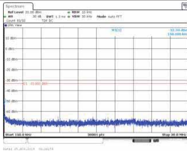
Band2_20MHz_16QAM_19100_1RB#0
