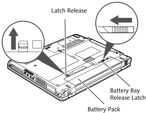
Figure 4-3. Removing a Battery
