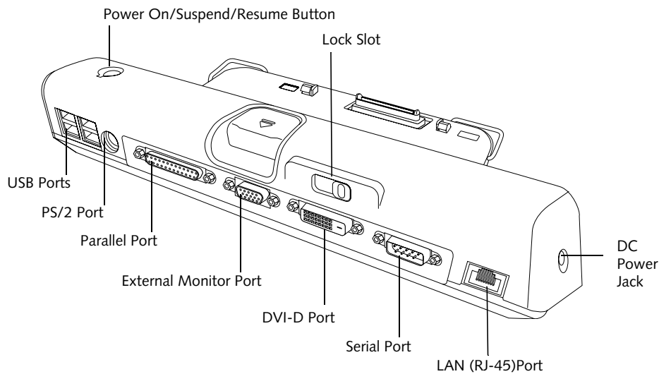
Figure 4-13. Port Replicator back panel
