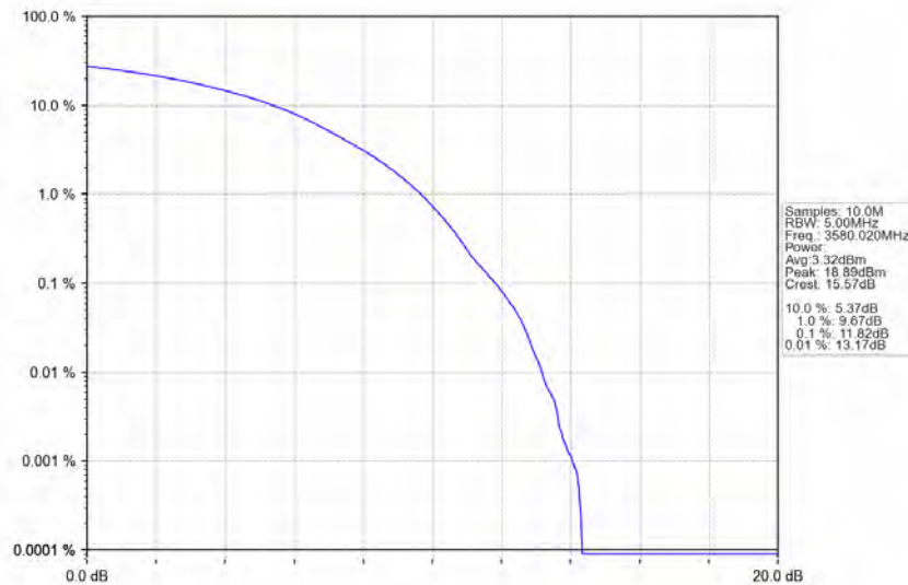
n78d_30kHz_MIMO_NTNV_60MHz_CP-OFDM_16_QAM_3580.02MHz_Outer_Full
