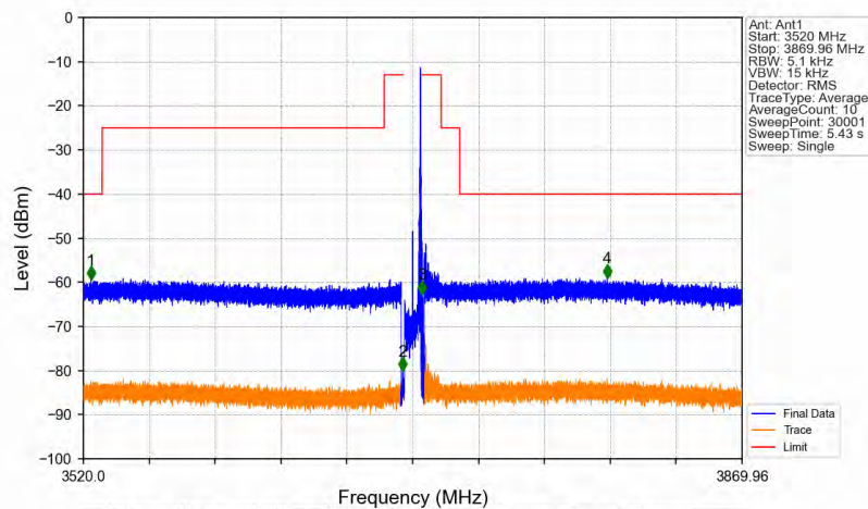
n78d_30kHz_MIMO_NTNV_10MHz_CP-OFDM QPSK_3694.98MHz_Edge_1RB_Right
