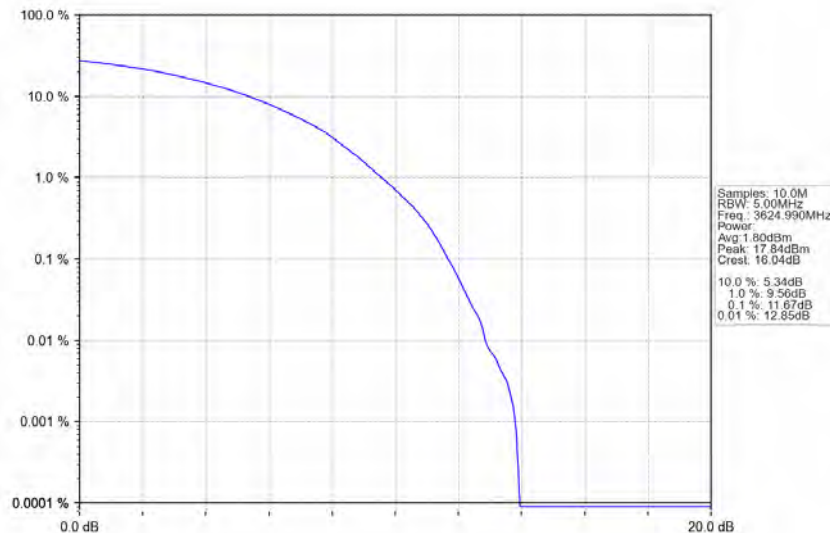
n78d_30kHz_MIMO_NTNV_80MHz_CP-OFDM QPSK_3624.99MHz_Outer_Full
