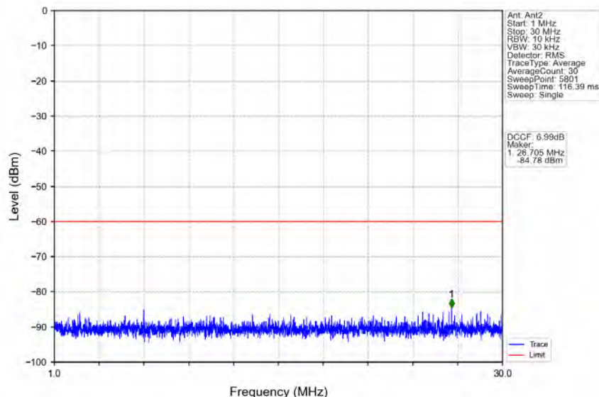
n78d_30kHz_MIMO_NTNV_20MHz_CP-OFDM_QPSK_3560.01MHz_Edge_1RB_Left
