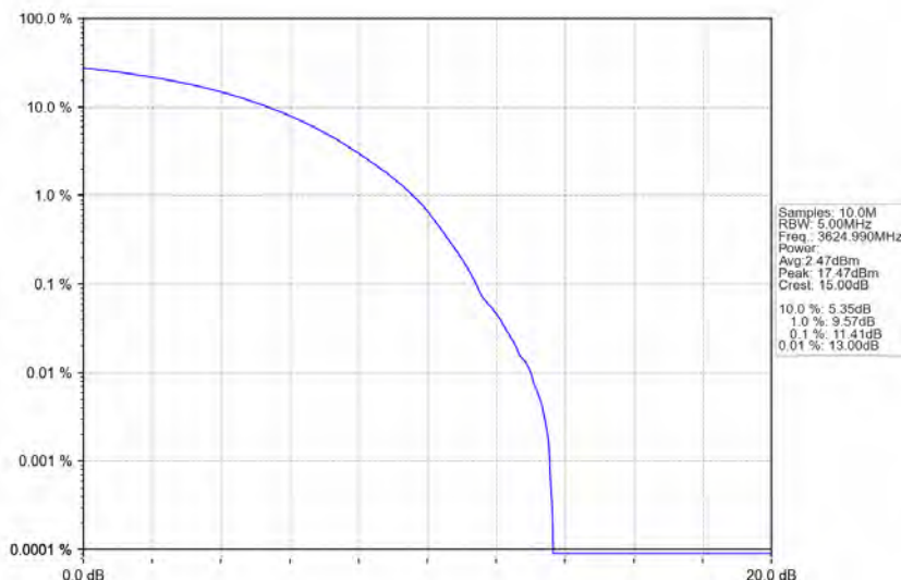
n78d_30kHz_MIMO_NTNV_70MHz_CP-OFDM_16_QAM_3624.99MHz_Outer_Full
