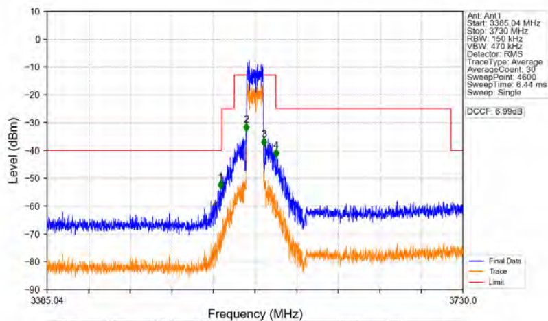
n78d_30kHz_MIMO_NTNV_15MHz_CP-OFDM_QPSK_3557.52MHz_Outer_Full
