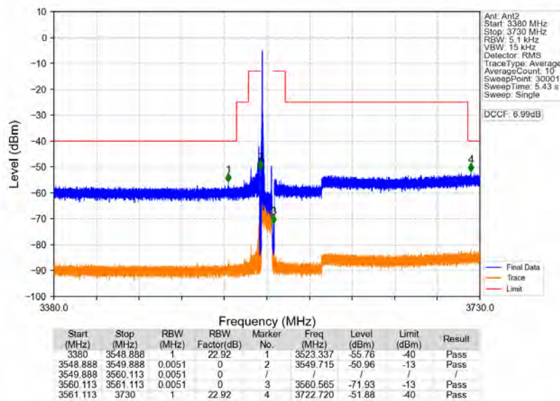
n78d_30kHz_MIMO_NTNV_10MHz_CP-OFDM_QPSK_3555MHz_Inner_1RB_Left
