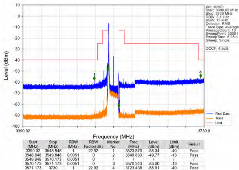
n78d_30kHz_MIMO_NTNV_20MHz_CP-OFDM_QPSK_3560.01MHz_Edge_1RB_Left
