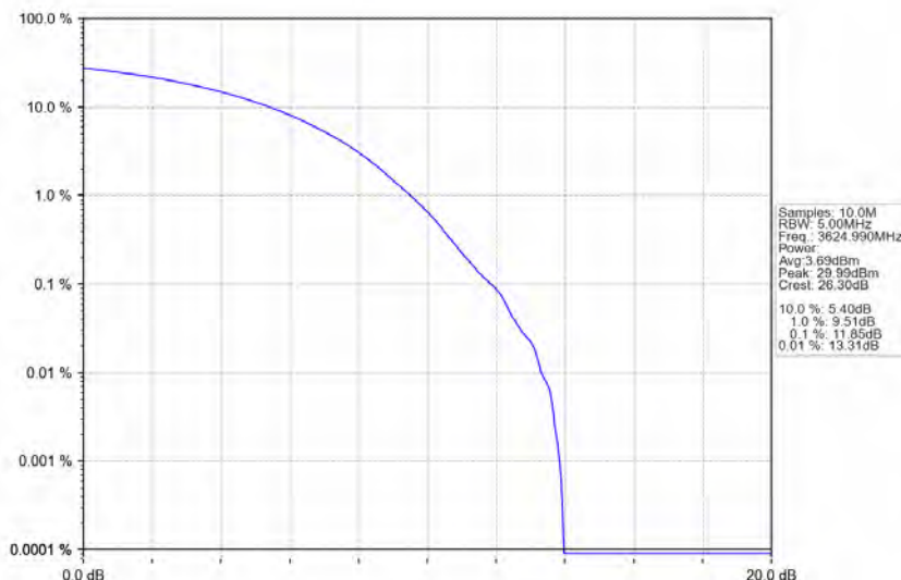
n78d_30kHz_MIMO_NTNV_50MHz_CP-OFDM_64_QAM_3624.99MHz_Outer_Full
