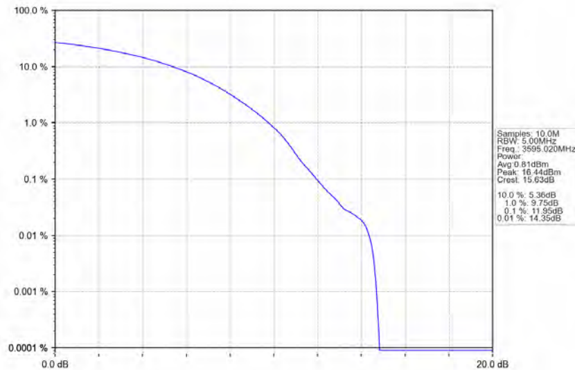
n78d_30kHz_MIMO_NTNV_90MHz_CP-OFDM_64_QAM_3595.02MHz_Outer_Full
