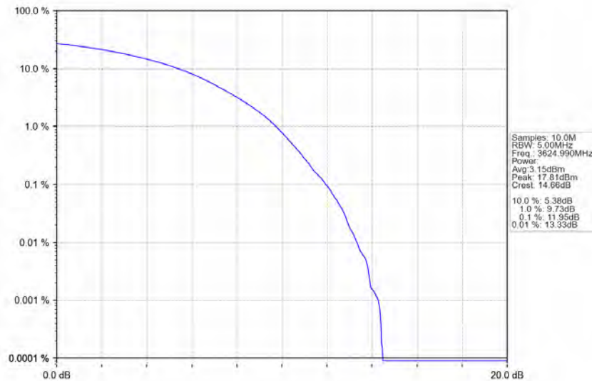
n78d_30kHz_MIMO_NTNV_60MHz_CP-OFDM_16_QAM_3624.99MHz_Outer_Full
