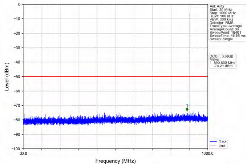
n78d_30kHz_MIMO_NTNV_15MHz_CP-OFDM_QPSK_3692.49MHz_Edge_1RB_Right
