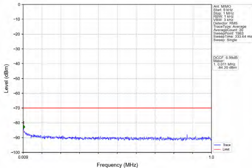
n78d_30kHz_MIMO_NTNV_10MHz_CP-OFDM QPSK_3694.98MHz_Edge_1RB_Right
