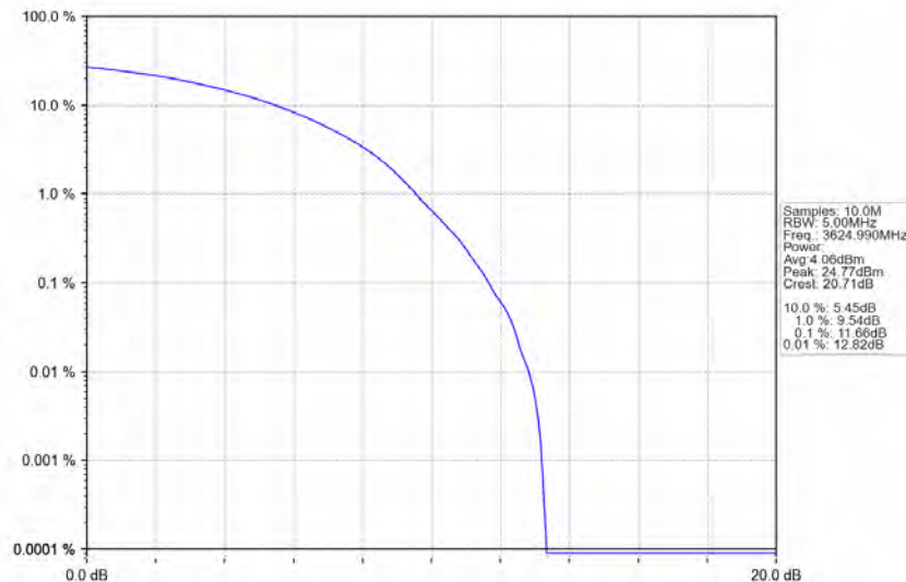
n78d_30kHz_MIMO_NTNV_50MHz_CP-OFDM_16_QAM_3624.99MHz_Outer_Full
