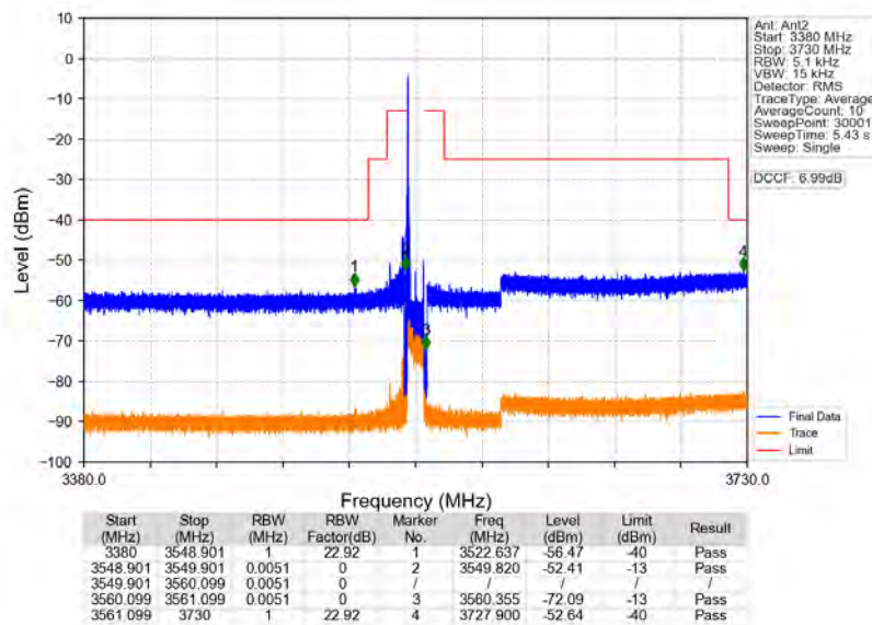
n78d_30kHz_MIMO_NTNV_10MHz_CP-OFDM_QPSK_3555MHz_Edge_1RB_Left
