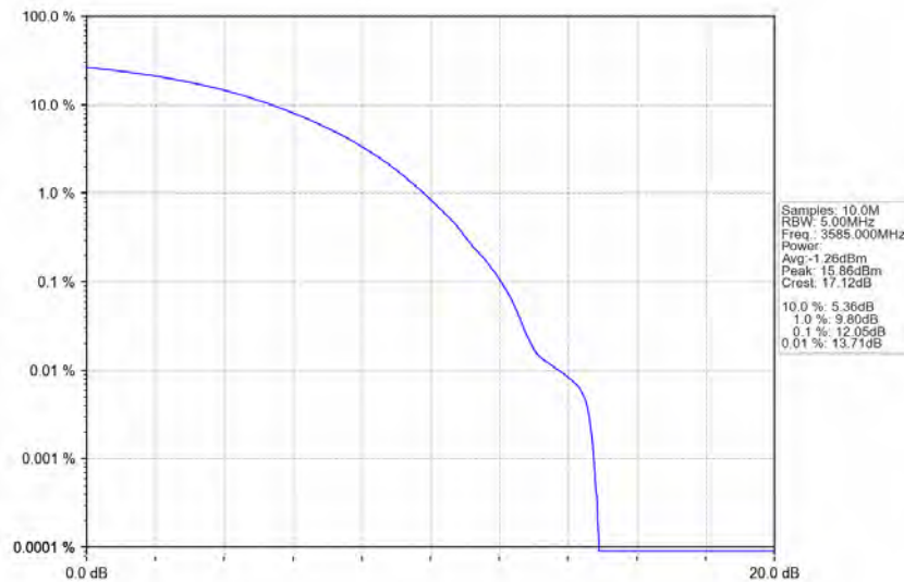
n78d_30kHz_MIMO_NTNV_70MHz_CP-OFDM_256_QAM_3585MHz_Outer_Full
