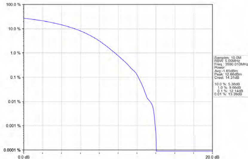
n78d_30kHz_MIMO_NTNV_80MHz_CP-OFDM_256_QAM_3590.01MHz_Outer_Full
