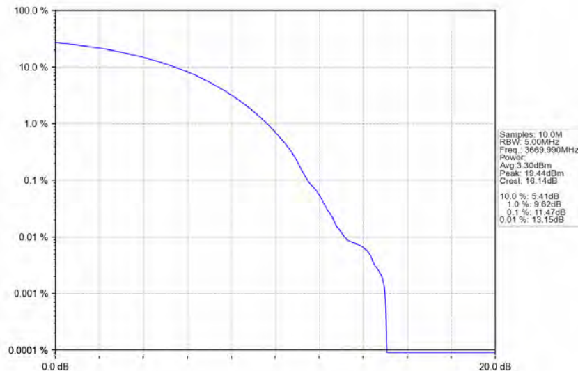
n78d_30kHz_MIMO_NTNV_60MHz_CP-OFDM QPSK_3669.99MHz_Outer_Full
