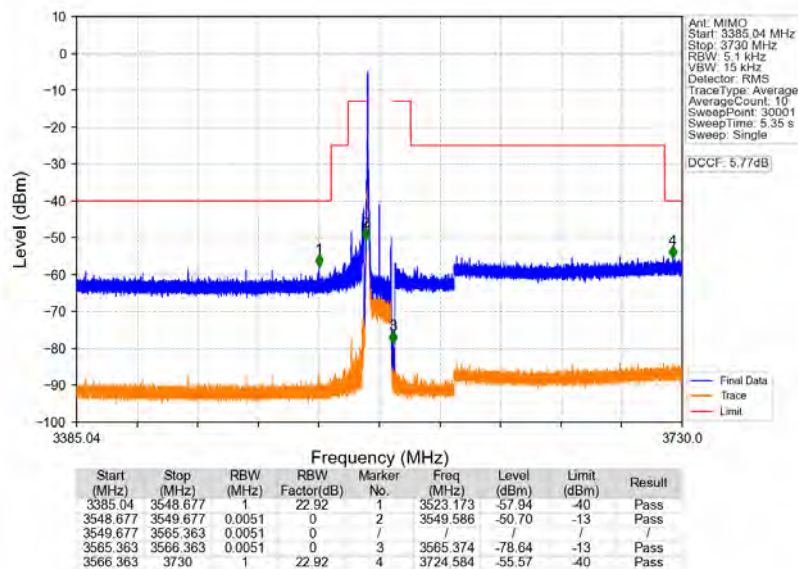
n78d_30kHz_MIMO_NTNV_15MHz_CP-OFDM_QPSK_3557.52MHz_Edge_1RB_Left
