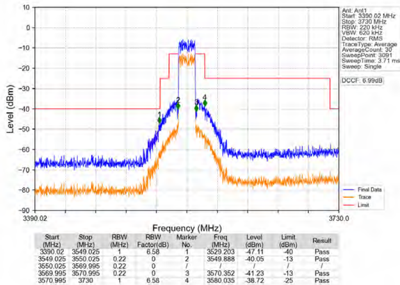
n78d_30kHz_MIMO_NTNV_20MHz_CP-OFDM_QPSK_3560.01MHz_Outer_Full
