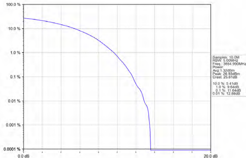
n78d_30kHz_MIMO_NTNV_90MHz_CP-OFDM_QPSK_3654.99MHz_Outer_Full
