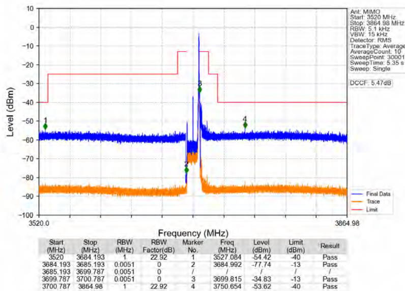
n78d_30kHz_MIMO_NTNV_15MHz_CP-OFDM_QPSK_3692.49MHz_Edge_1RB_Right
