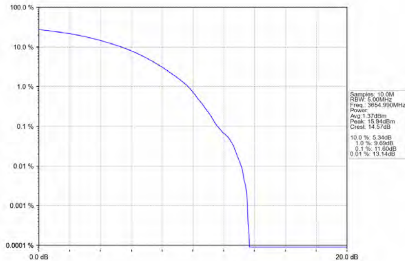
n78d_30kHz_MIMO_NTNV_90MHz_CP-OFDM_16_QAM_3654.99MHz_Outer_Full
