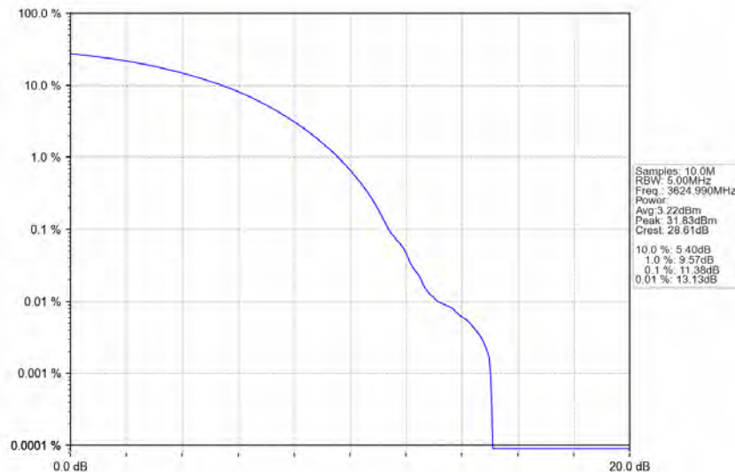
n78d_30kHz_MIMO_NTNV_60MHz_CP-OFDM QPSK_3624.99MHz_Outer_Full
