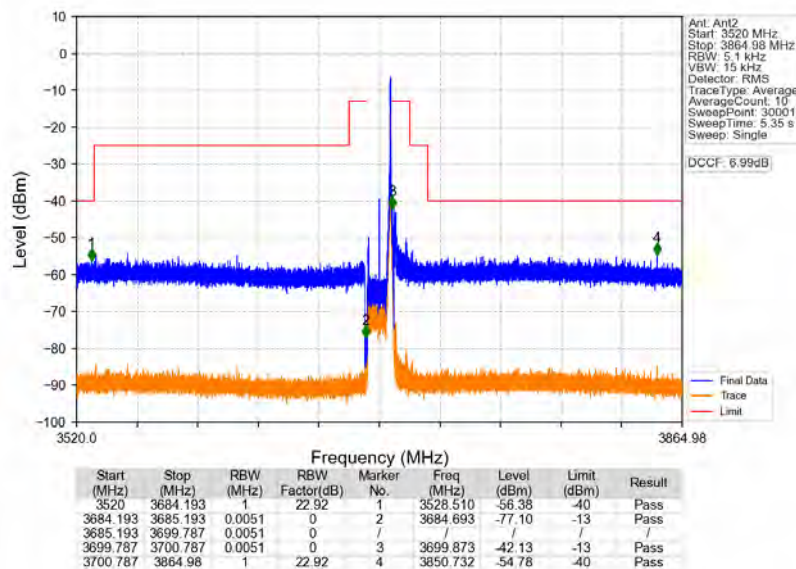
n78d_30kHz_MIMO_NTNV_15MHz_CP-OFDM_QPSK_3692.49MHz_Inner_1RB_Right
