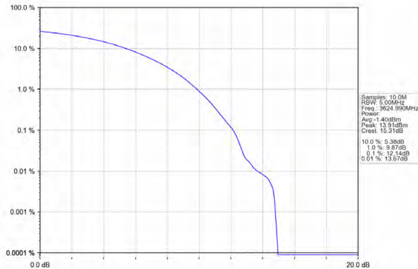
n78d_30kHz_MIMO_NTNV_70MHz_CP-OFDM_256_QAM_3624.99MHz_Outer_Full
