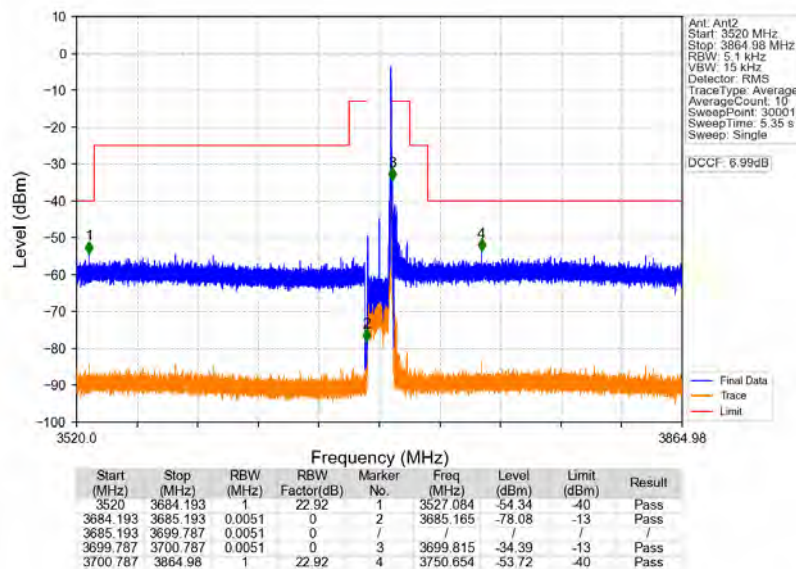
n78d_30kHz_MIMO_NTNV_15MHz_CP-OFDM_QPSK_3692.49MHz_Edge_1RB_Right
