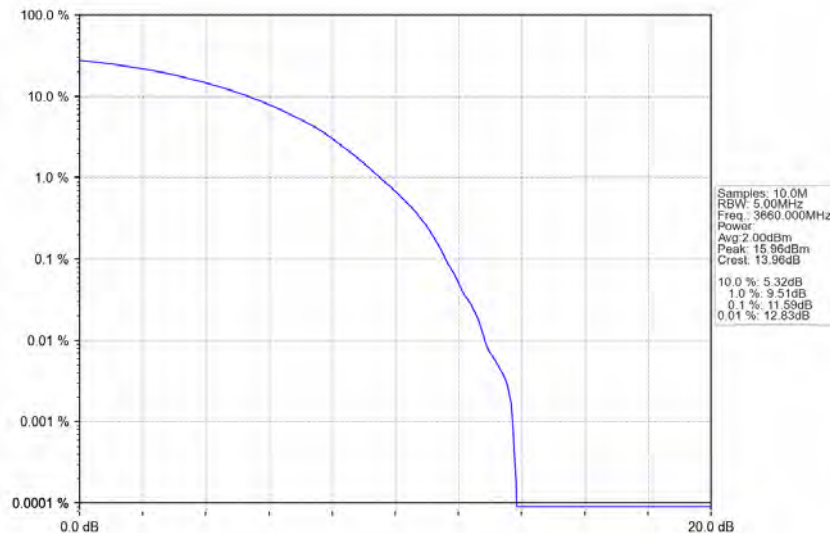
n78d_30kHz_MIMO_NTNV_80MHz_CP-OFDM QPSK_3660MHz_Outer_Full
