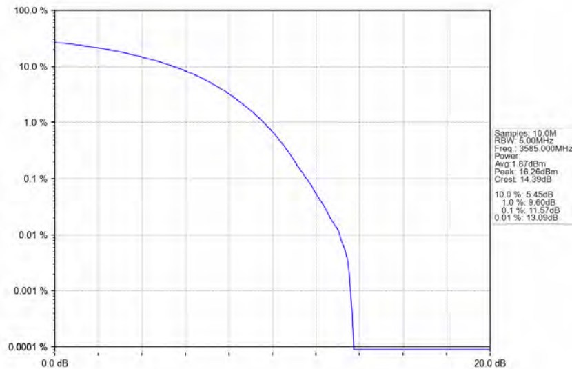
n78d_30kHz_MIMO_NTNV_70MHz_CP-OFDM_64_QAM_3585MHz_Outer_Full
