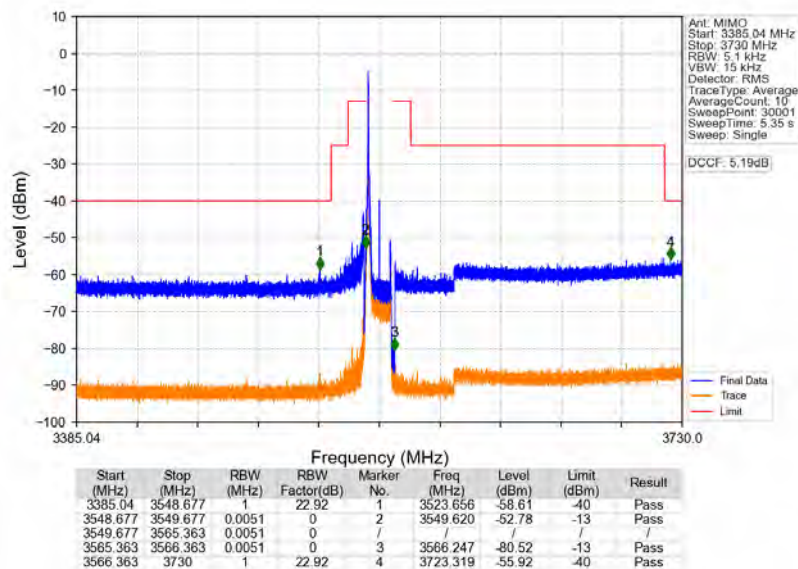
n78d_30kHz_MIMO_NTNV_15MHz_CP-OFDM_QPSK_3557.52MHz_Inner_1RB_Left
