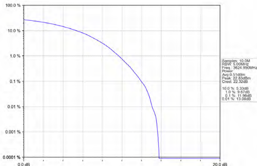
n78d_30kHz_MIMO_NTNV_50MHz_CP-OFDM_256_QAM_3624.99MHz_Outer_Full
