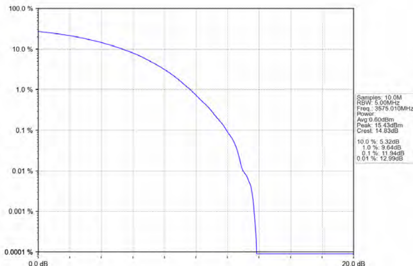
n78d_30kHz_MIMO_NTNV_50MHz_CP-OFDM_256_QAM_3575.01MHz_Outer_Full
