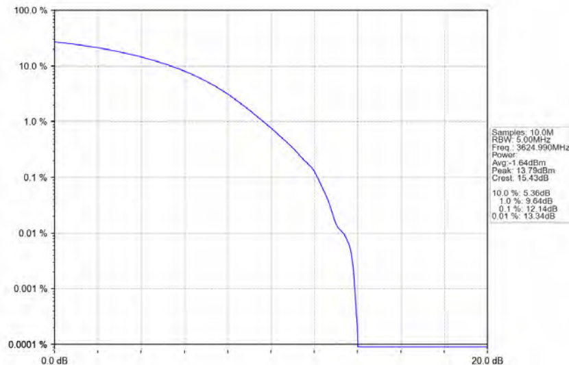
n78d_30kHz_MIMO_NTNV_80MHz_CP-OFDM_256_QAM_3624.99MHz_Outer_Full
