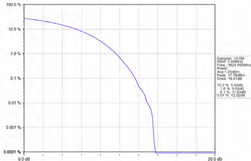
n78d_30kHz_MIMO_NTNV_90MHz_CP-OFDM_QPSK_3624.99MHz_Outer_Full
