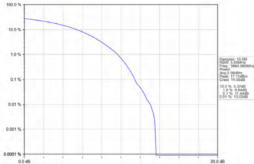
n78d_30kHz_MIMO_NTNV_70MHz_CP-OFDM_16_QAM_3664.98MHz_Outer_Full
