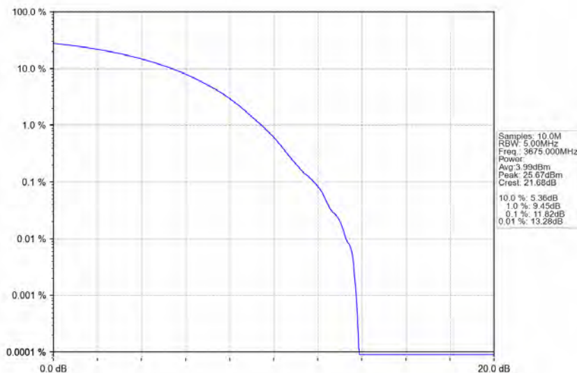
n78d_30kHz_MIMO_NTNV_50MHz_CP-OFDM_64_QAM_3675MHz_Outer_Full
