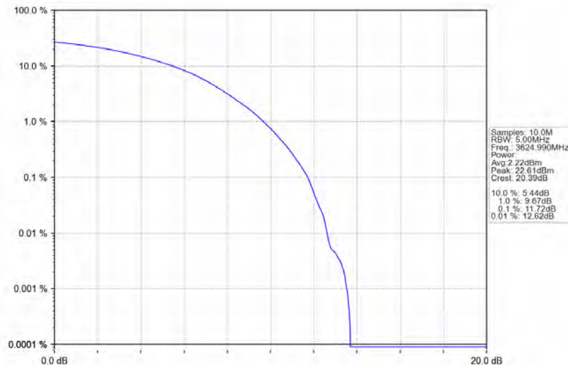
n78d_30kHz_MIMO_NTNV_70MHz_CP-OFDM QPSK_3624.99MHz_Outer_Full
