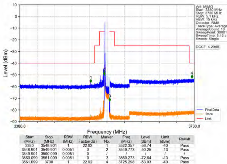
n78d_30kHz_MIMO_NTNV_10MHz_CP-OFDM_QPSK_3555MHz_Edge_1RB_Left
