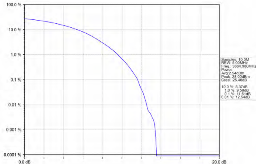
n78d_30kHz_MIMO_NTNV_70MHz_CP-OFDM QPSK_3664.98MHz_Outer_Full
