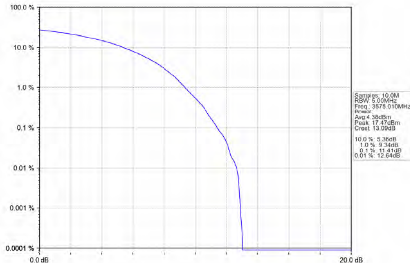
n78d_30kHz_MIMO_NTNV_50MHz_CP-OFDM_16_QAM_3575.01MHz_Outer_Full
