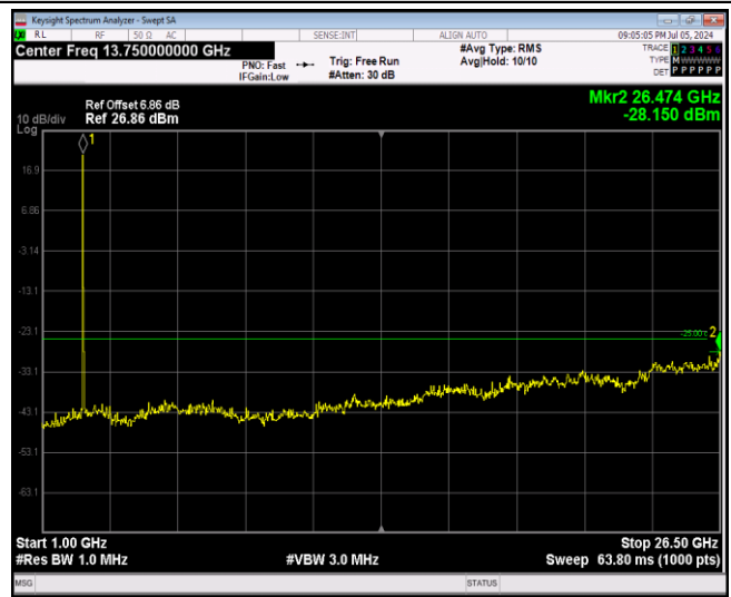
Band41-20MHz-16QAM-40140-1RB#0-Range2:1000~26500MHz
