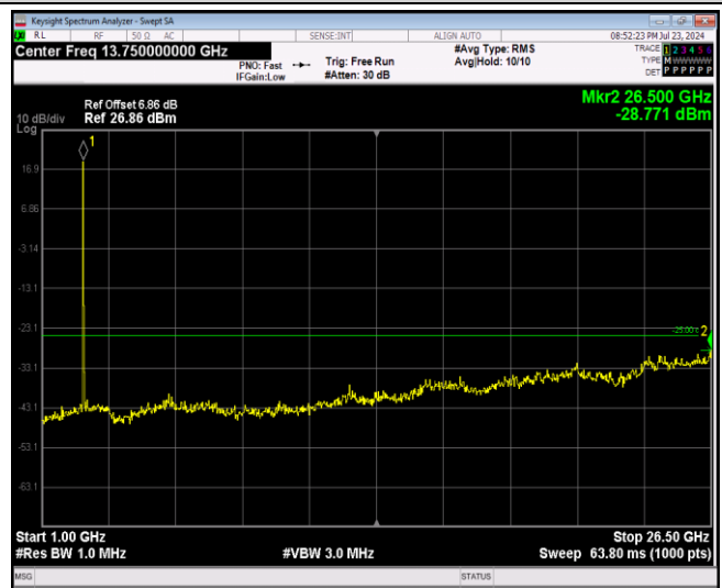
Band41-20MHz-64QAM-41140-1RB#0-Range2:1000~26500MHz
