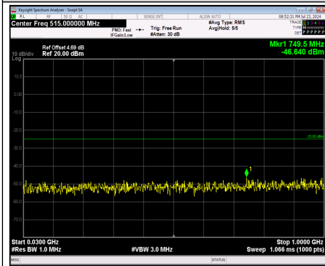
Band41-20MHz-64QAM-41140-1RB#0-Range1:30~1000MHz
