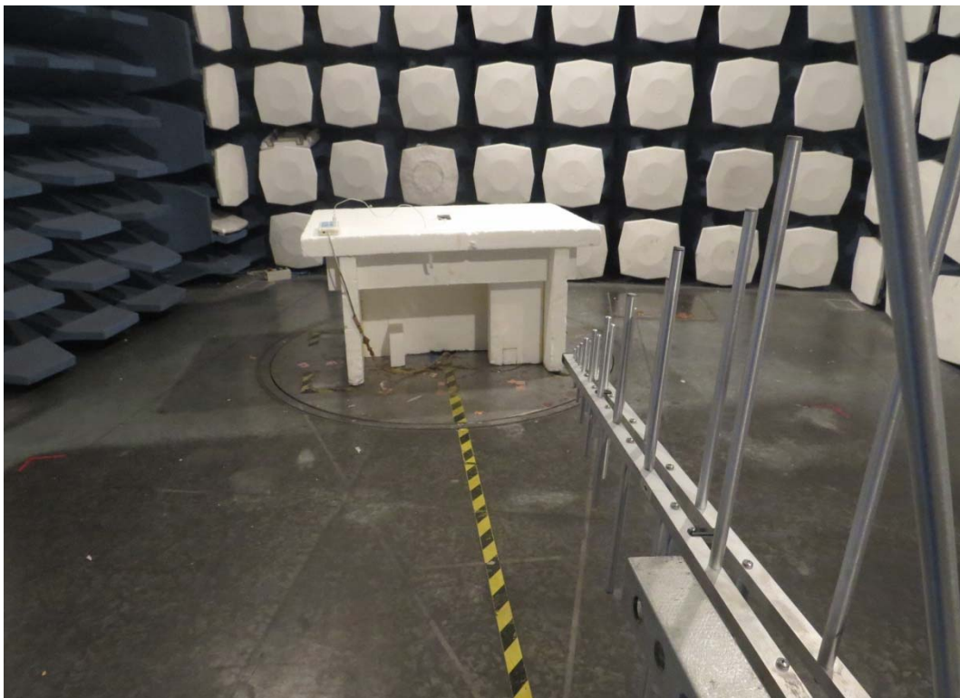
30M Hz-1GHz
