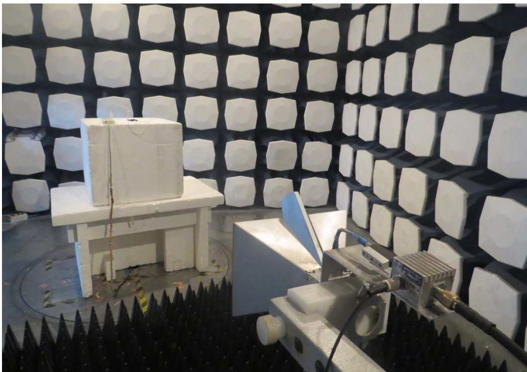
Above 1GHz
