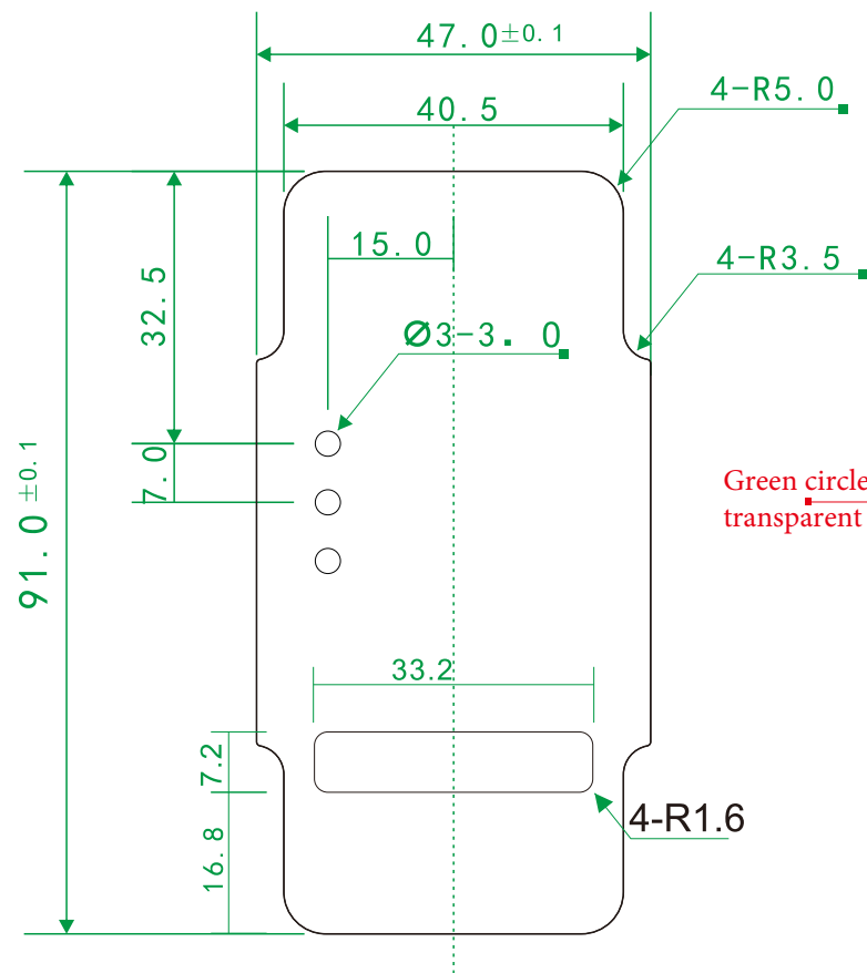
(Dimensional drawing)
