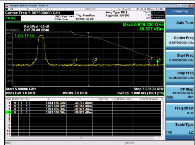
11A(10MHZ)-Ant1-5820-PASS
