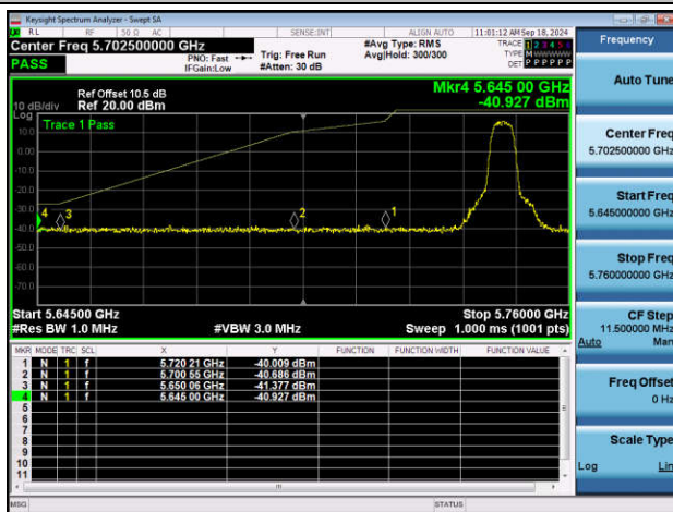
11A(10MHZ)-Ant1-5740-PASS
