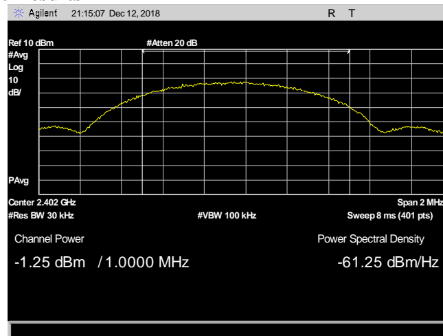
Plot 4. Maximum Conducted Output Power, 2402 MHz, Channel Power
