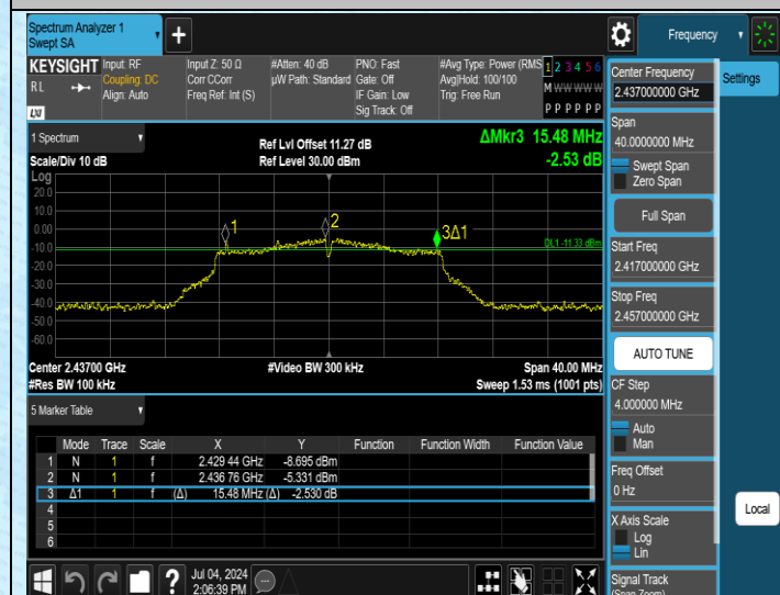
11G-Ant1-2437-PASS
