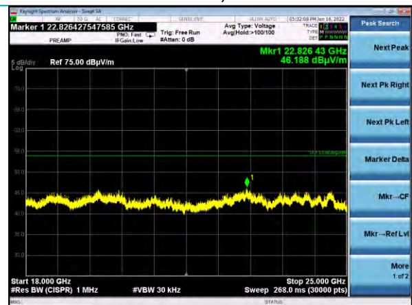
18-25 GHz, Vertical Antenna Flat EUT, Channel 38
