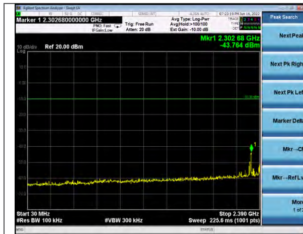
DH5 30-2390 MHz Channel 0
