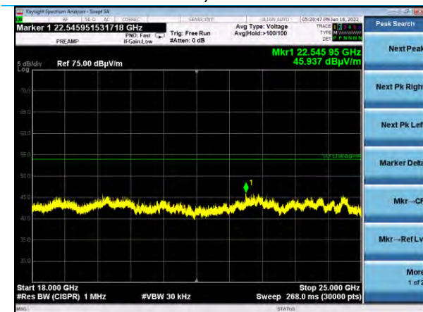
18-25 GHz, Horizontal Antenna Flat EUT, Channel 38
