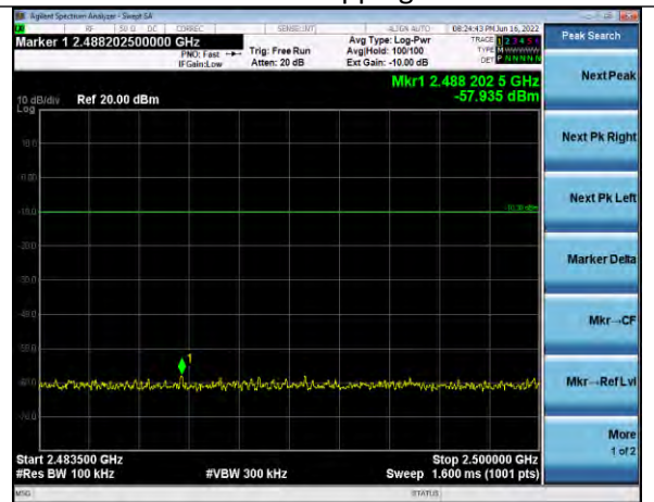
2-DH5 Hopping
