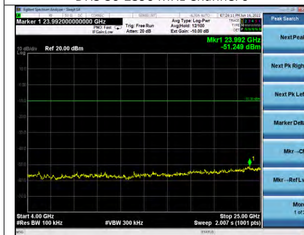
DH5 4000-25000 MHz Channel 0
