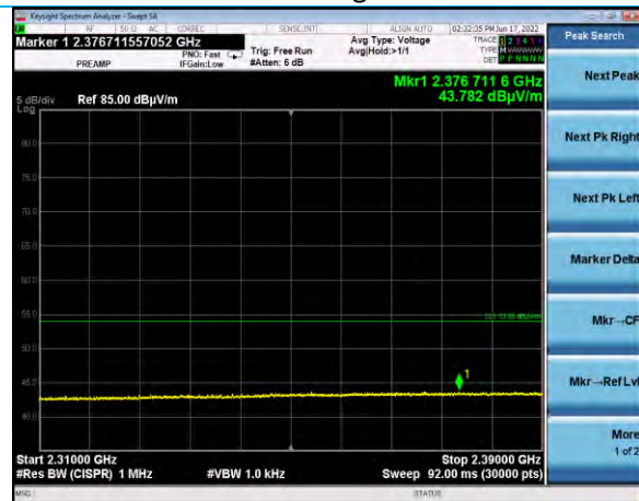
3-DH5 2.31-2.39 GHz, Vertical Antenna Horizontal EUT, Hopping Average
