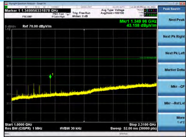
1-2.31 GHz, Vertical Antenna Vertical EUT, Channel 38
