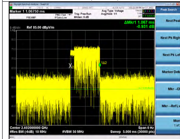
3-DH5 (1 kHz)
