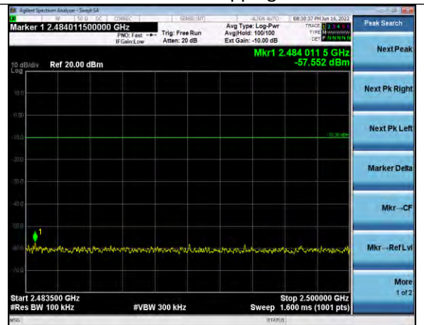
3-DH5 Hopping
