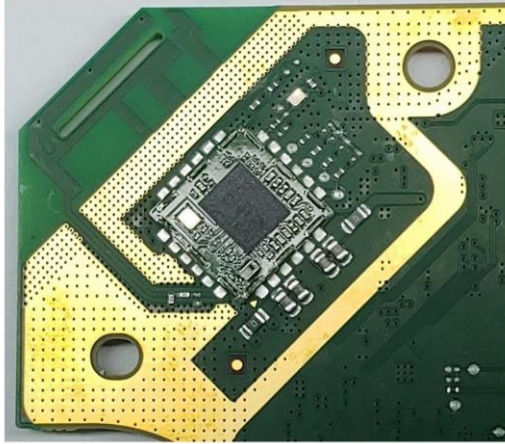
-Antenna#2 (TOP view)-
