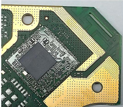
-Antenna#1 (TOP view)-
