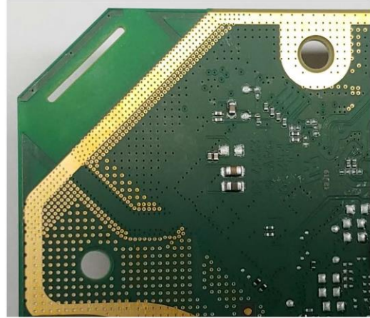
-Antenna#1 (Bottom view)-
