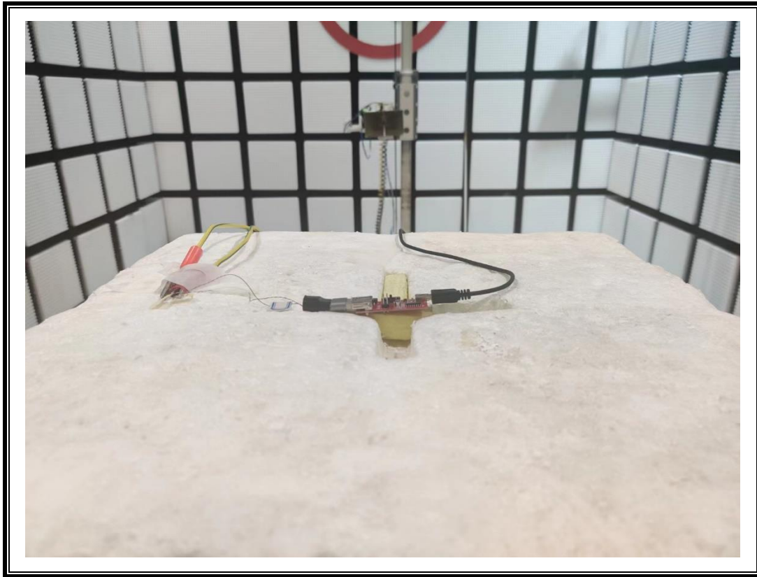
RADIATED RF MEASUREMENT SETUP (Above 1G – X axis)
