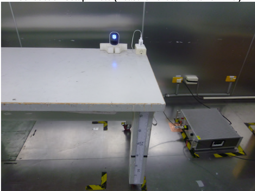
Conduction Setup Photo (Measurement at AC Power Line )
