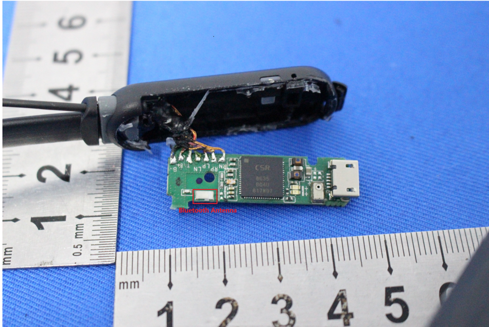
Antenna of EUT
