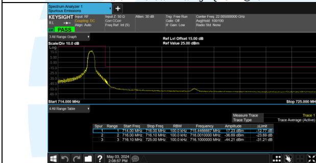
Band 12 23130/711.0/High 16QAM 1@49
