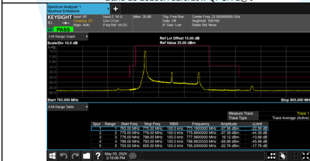
Band 13 23230/782.0/Low 16QAM 1@0
