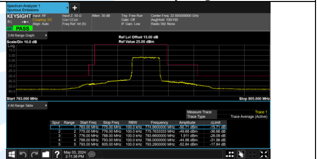
Band 13 23255/784.5/High QPSK 25@0
