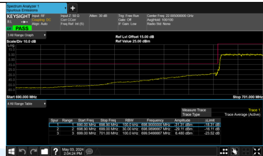
Band 12 23025/700.5/Low QPSK 15@0
