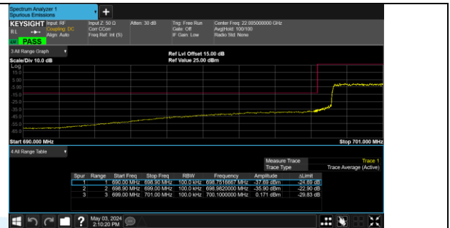
Band 12 23060/704.0/Low 16QAM 50@0
