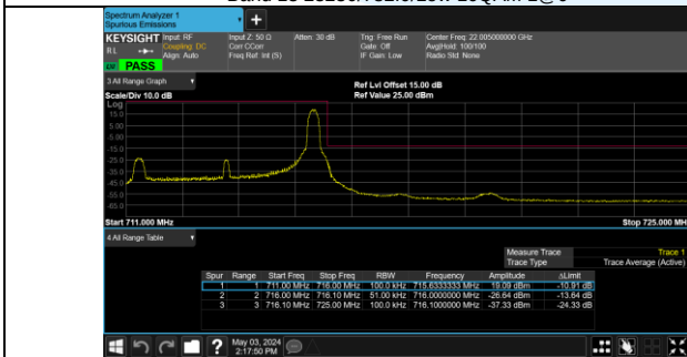
Band 17 23825/713.5/High QPSK 1@24
