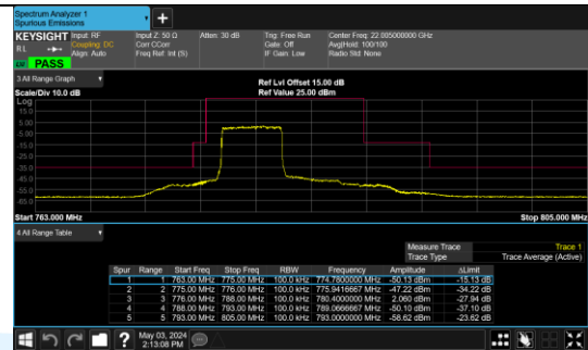
Band 13 23205/779.5/Low QPSK 25@0
