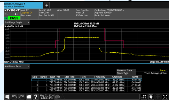
Band 13 23230/782.0/Low QPSK 50@0
