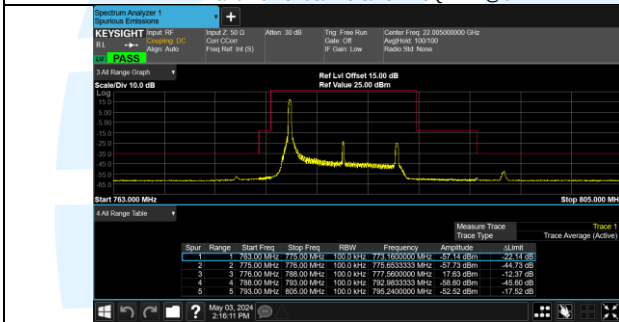
Band 13 23230/782.0/Low QPSK 1@0
