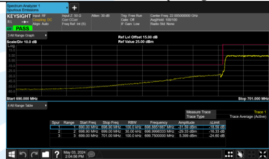
Band 12 23025/700.5/Low 16QAM 15@0
