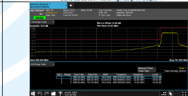
Band 12 23017/699.7/Low QPSK 6@0
