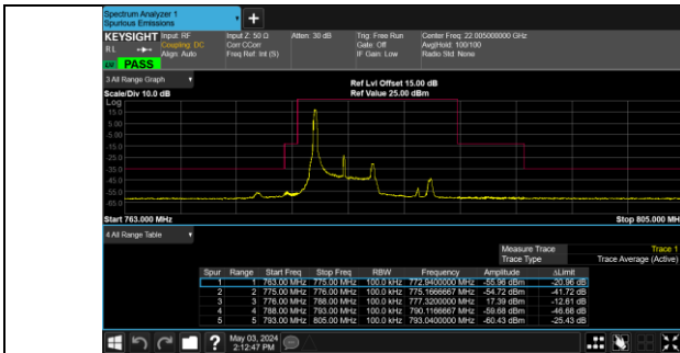
Band 13 23205/779.5/Low QPSK 1@0
