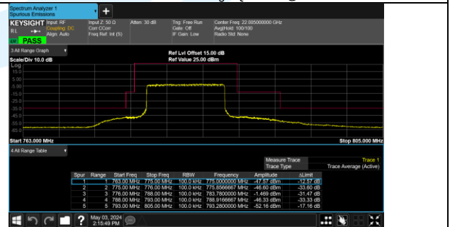
Band 13 23230/782.0/High 16QAM 50@0
