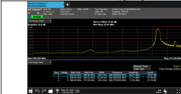
Band 12 23025/700.5/Low 16QAM 1@0
