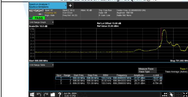
Band 12 23017/699.7/Low QPSK 1@0
