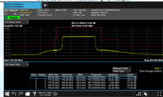
Band 13 23230/782.0/Low 16QAM 50@0
