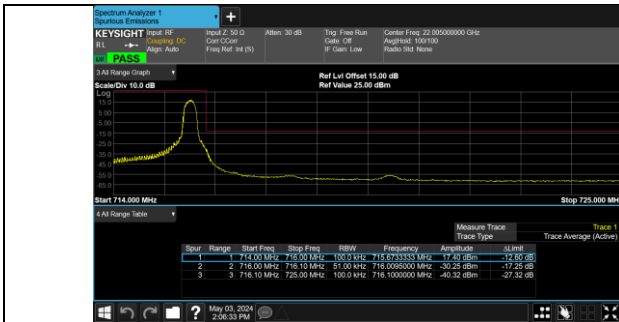
Band 12 23155/713.5/High 16QAM 1@24
