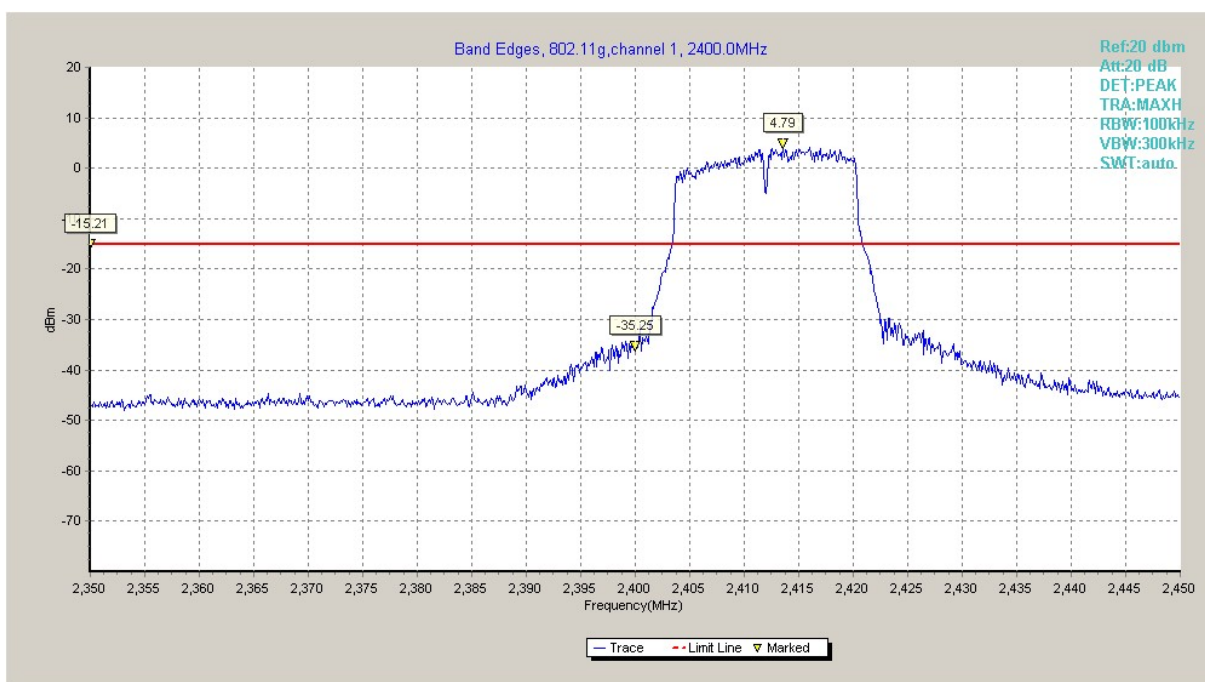
Fig.A.5.5 Band Edges (802.11g, Ch 1)
