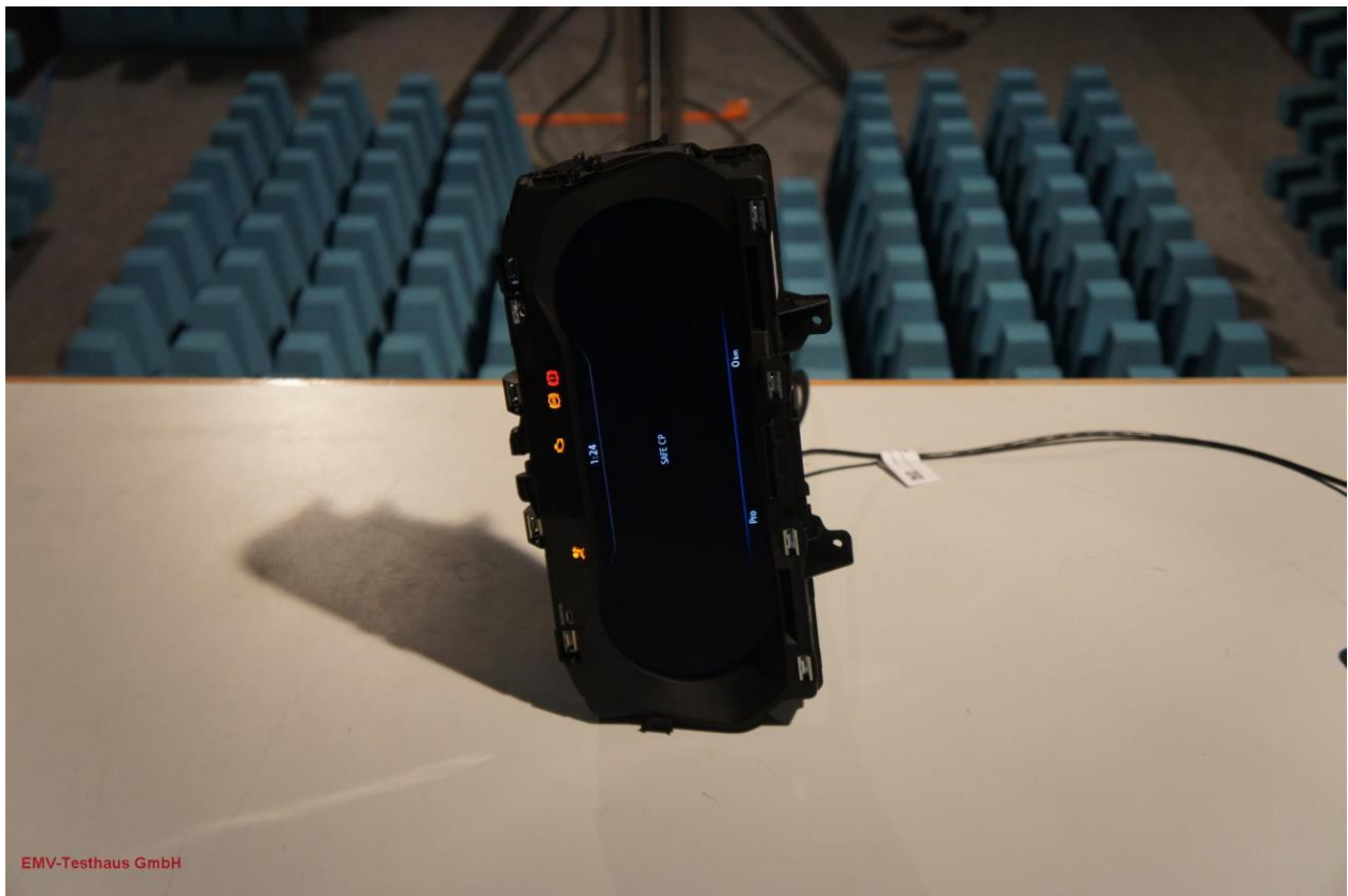
Picture 8: EUT-position 3
