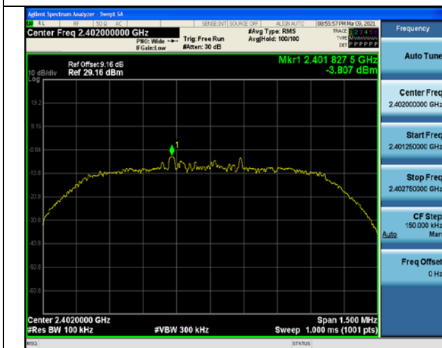
GFSK on Channel 00
