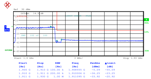
10MHz_High_QPSK_50@0
