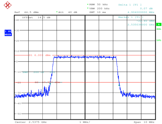
26dB Bandwidth
