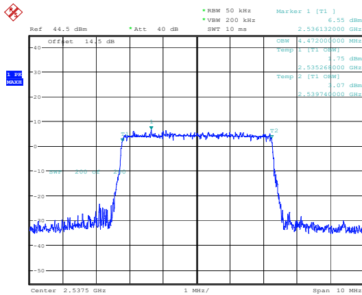
Occupied Bandwidth
