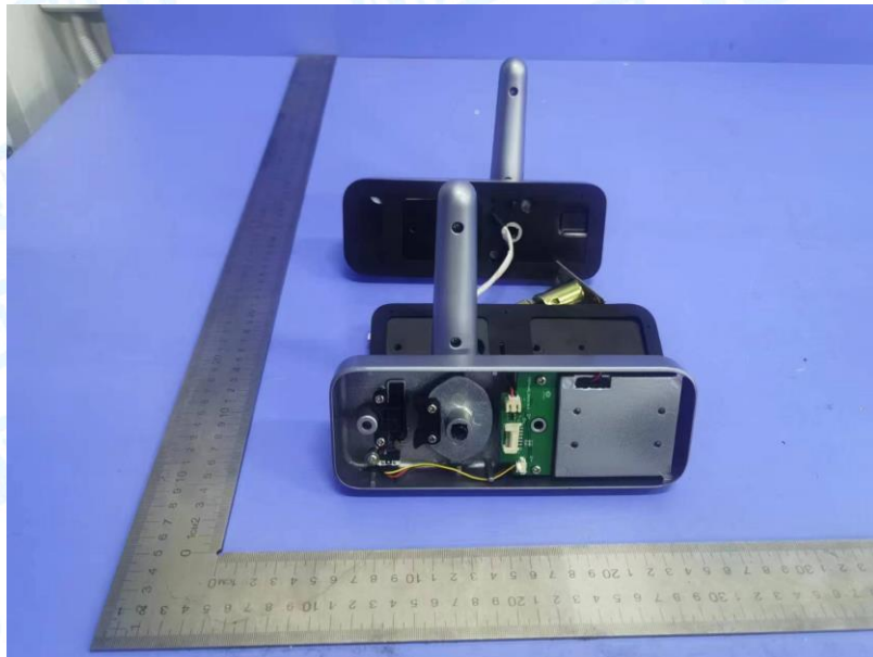
Photo 15 Internal of EUT
