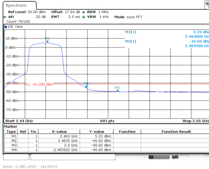
11G_Ant1_High_2462_Peak
