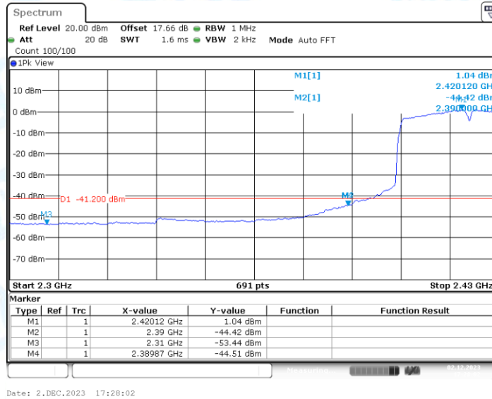
11N40SISO_Ant1_Low_2422_Peak
