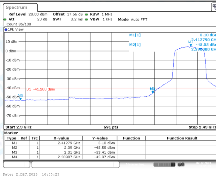
11N20SISO_Ant1_Low_2412_Peak
