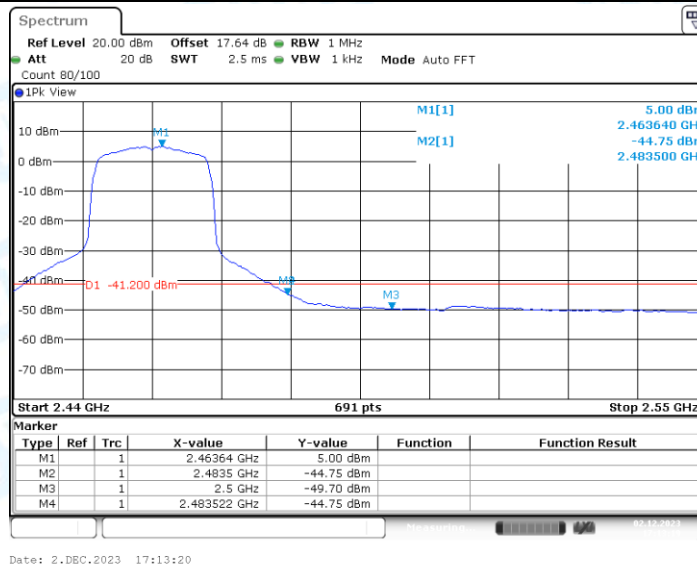
11N20SISO_Ant1_High_2462_Peak
