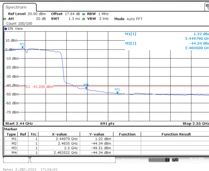
11N40SISO_Ant1_High_2452_Peak
