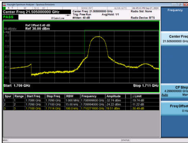
Band66_1.4MHz_QPSK_131979_1RB#0
