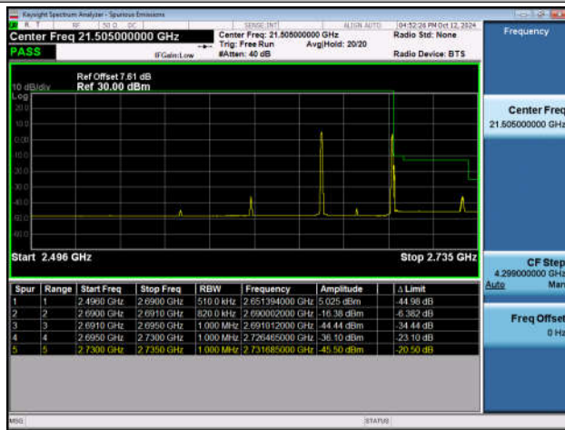
10MHz-20MHz_QPSK@QPSK-QPSK@QPSK_20805-209 49_1RB#0@50RB#0-1RB#99@100RB#0
