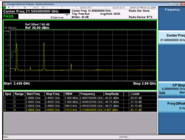
20MHz-20MHz_QPSK@QPSK-QPSK@QPSK_41292-414 90_1RB#0@100RB#0-1RB#99@100RB#0
