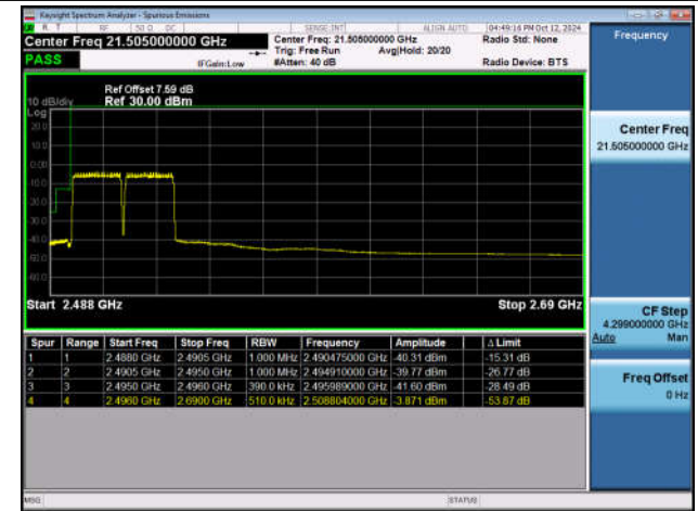
20MHz-20MHz_QPSK@QPSK-QPSK@QPSK_41292-4149 0_100RB#0@100RB#0-100RB#0@100RB#0
