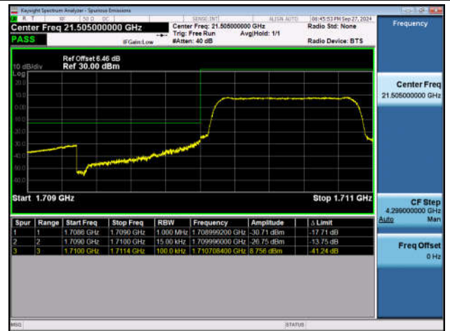
Band66_1.4MHz_QPSK_131979_6RB#0
