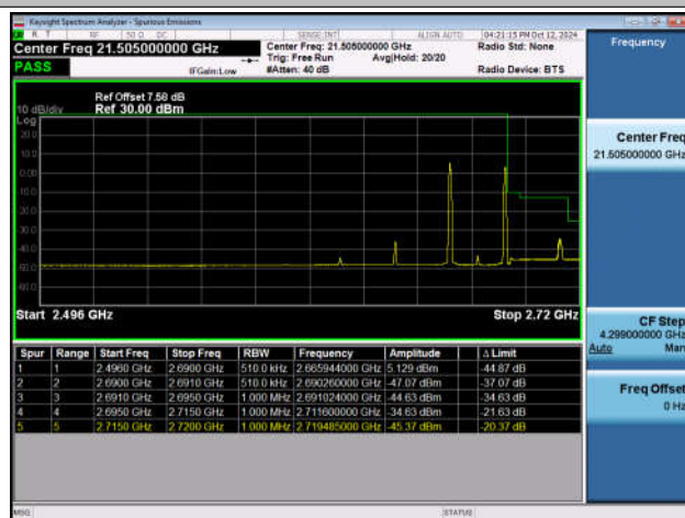
20MHz-10MHz_QPSK@QPSK-QPSK@QPSK_39750-398 94_1RB#0@100RB#0-1RB#49@50RB#0
