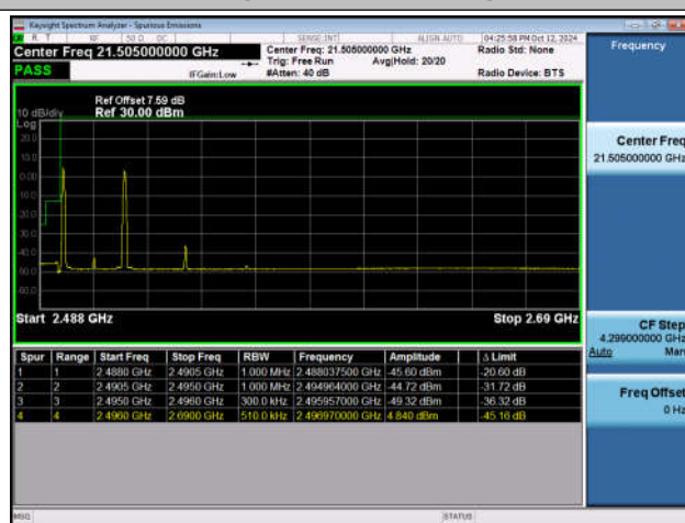
20MHz-10MHz_QPSK@QPSK-QPSK@QPSK_39750-398 94_1RB#0@100RB#0-1RB#49@50RB#0
