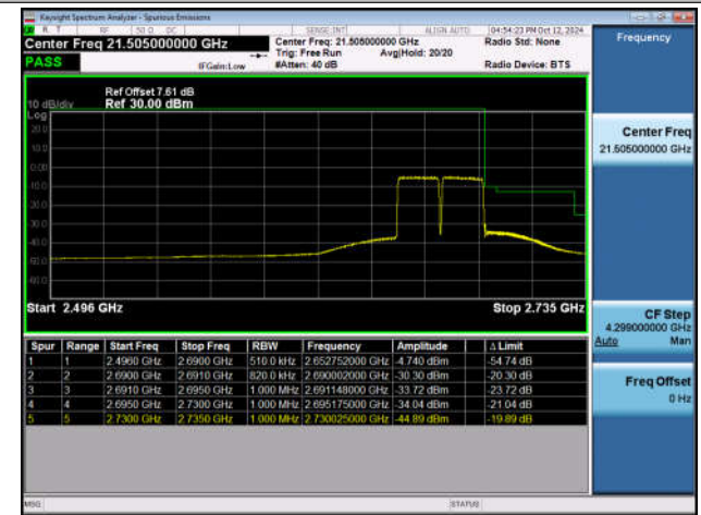
10MHz-20MHz_QPSK@QPSK-QPSK@QPSK_20805-2094 9_50RB#0@50RB#0-100RB#0@100RB#0
