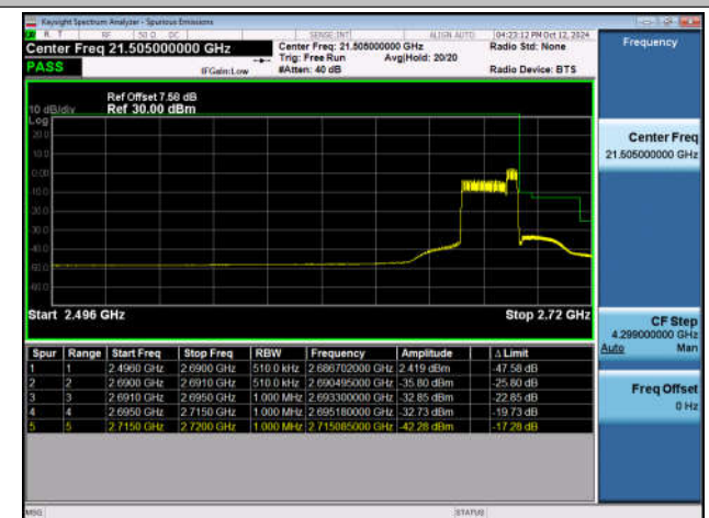
20MHz-10MHz_QPSK@QPSK-QPSK@QPSK_39750-3989 4_100RB#0@100RB#0-50RB#0@50RB#0
