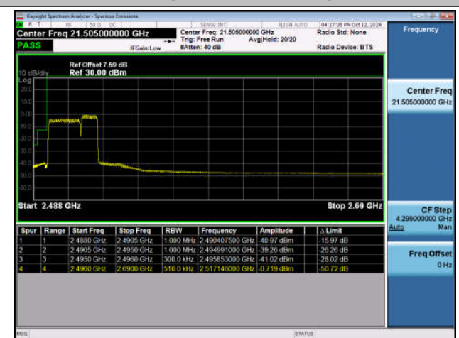
20MHz-10MHz_QPSK@QPSK-QPSK@QPSK_39750-3989 4_100RB#0@100RB#0-50RB#0@50RB#0
