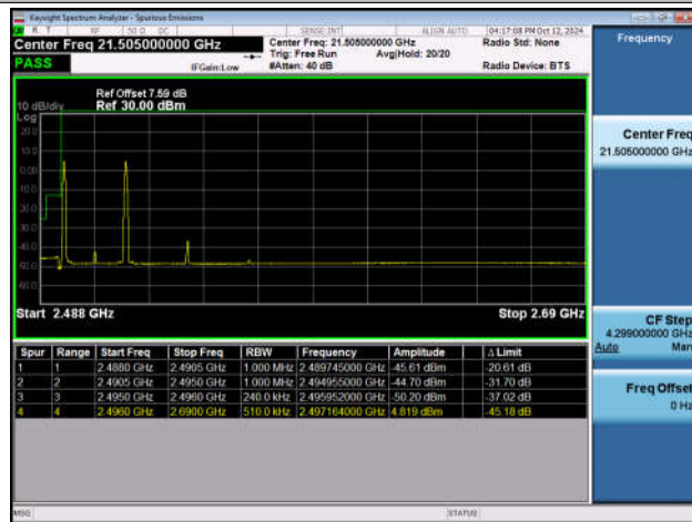
20MHz-5MHz_QPSK@QPSK-QPSK@QPSK_41440-4155 7_1RB#0@100RB#0-1RB#24@25RB#0
