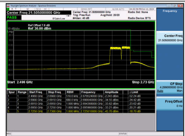
20MHz-15MHz_QPSK@QPSK-QPSK@QPSK_41341-4151 2_100RB#0@100RB#0-75RB#0@75RB#0
