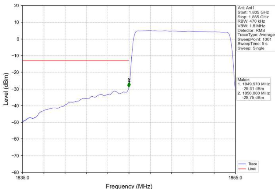
Band2_15MHz_QPSK_LCH_1857.5MHz_RB_75_0_NTNV
