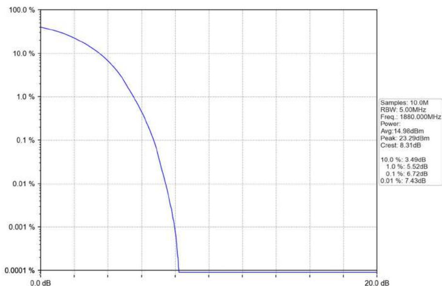
Band2_15MHz_QPSK_MCH_1880MHz_RB_75_0_NTNV
