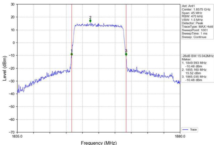
Band2_15MHz_QPSK_LCH_1857.5MHz_RB_75_0_NTNV
