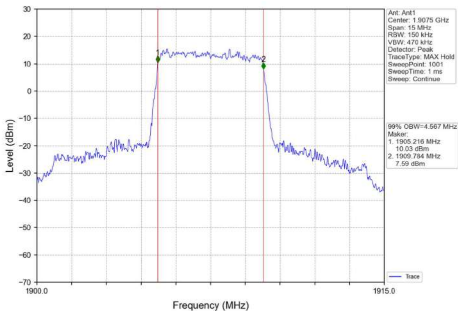
Band2_5MHz_QPSK_HCH_1907.5MHz_RB_25_0_NTNV
