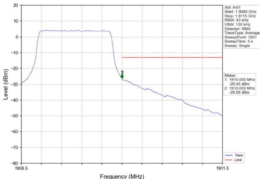
Band2_1.4MHz_16QAM_HCH_1909.3MHz_RB_6_0_NTNV
