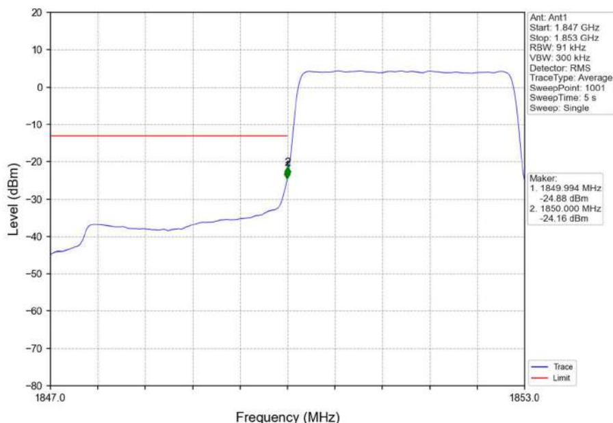
Band2_3MHz_QPSK_LCH_1851.5MHz_RB_15_0_NTNV
