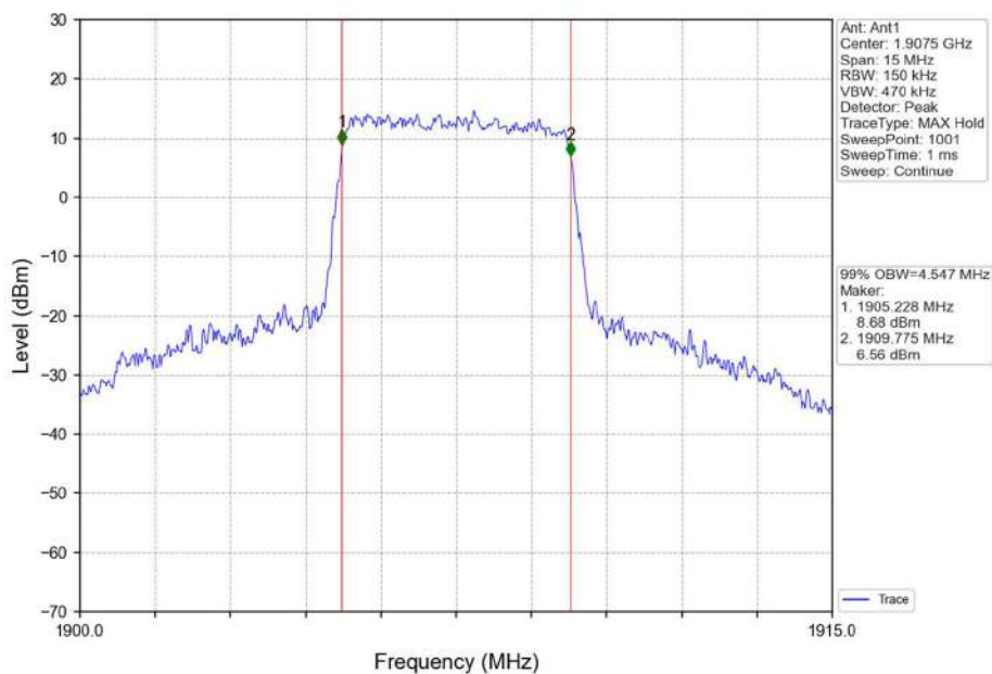
Band2_5MHz_16QAM_HCH_1907.5MHz_RB_25_0_NTNV
