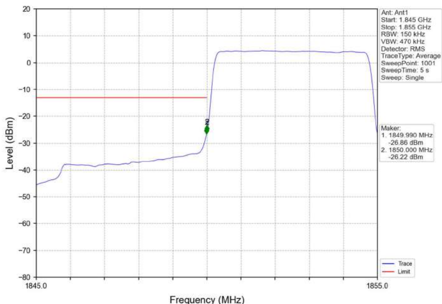
Band2_5MHz_QPSK_LCH_1852.5MHz_RB_25_0_NTNV
