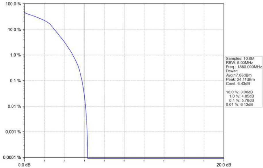
Band2_1.4MHz_16QAM_MCH_1880MHz_RB_6_0_NTNV
