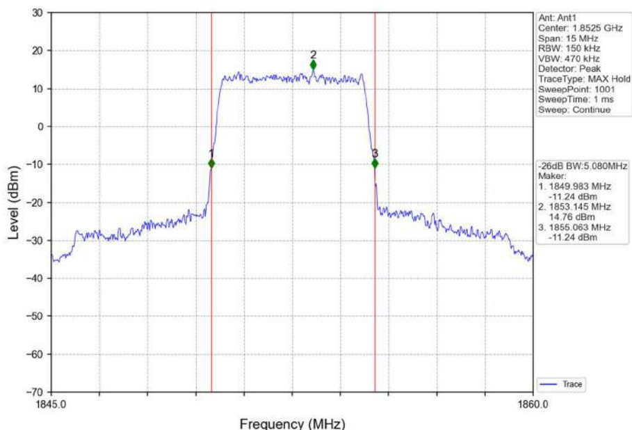
Band2_5MHz_QPSK_LCH_1852.5MHz_RB_25_0_NTNV
