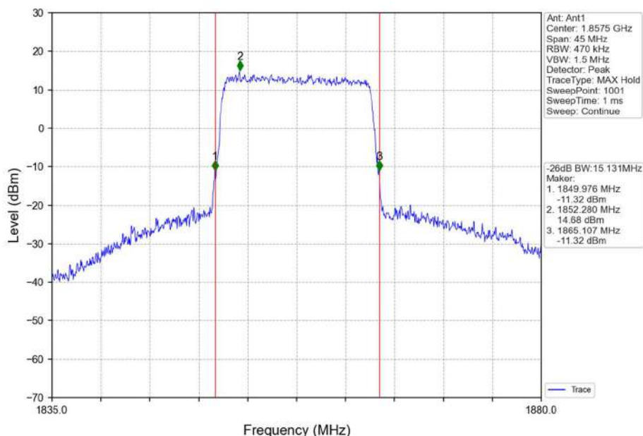
Band2_15MHz_16QAM_LCH_1857.5MHz_RB_75_0_NTNV
