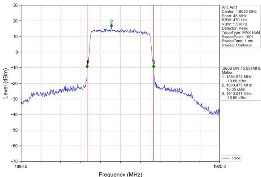
Band2_15MHz_QPSK_HCH_1902.5MHz_RB_75_0_NTNV
