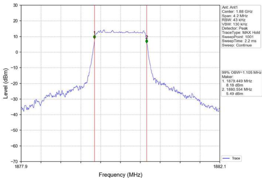
Band2_1.4MHz_16QAM_MCH_1880MHz_RB_6_0_NTNV
