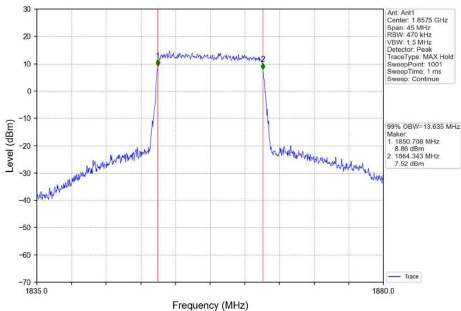
Band2_15MHz_16QAM_LCH_1857.5MHz_RB_75_0_NTNV
