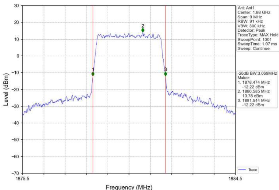
Band2_3MHz_16QAM_MCH_1880MHz_RB_15_0_NTNV
