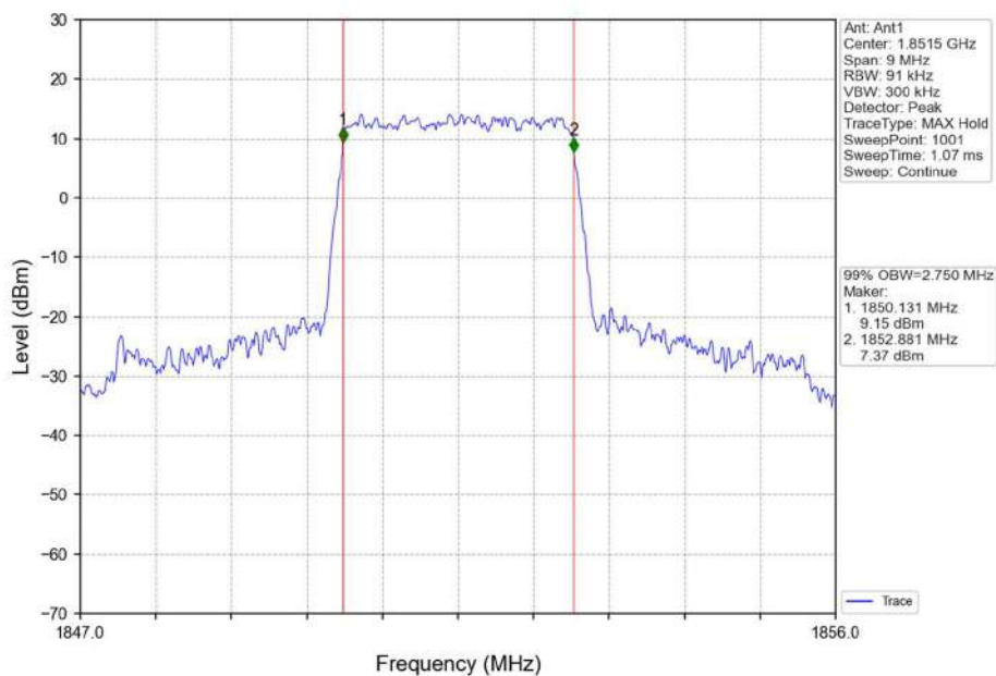
Band2_3MHz_QPSK_LCH_1851.5MHz_RB_15_0_NTNV
