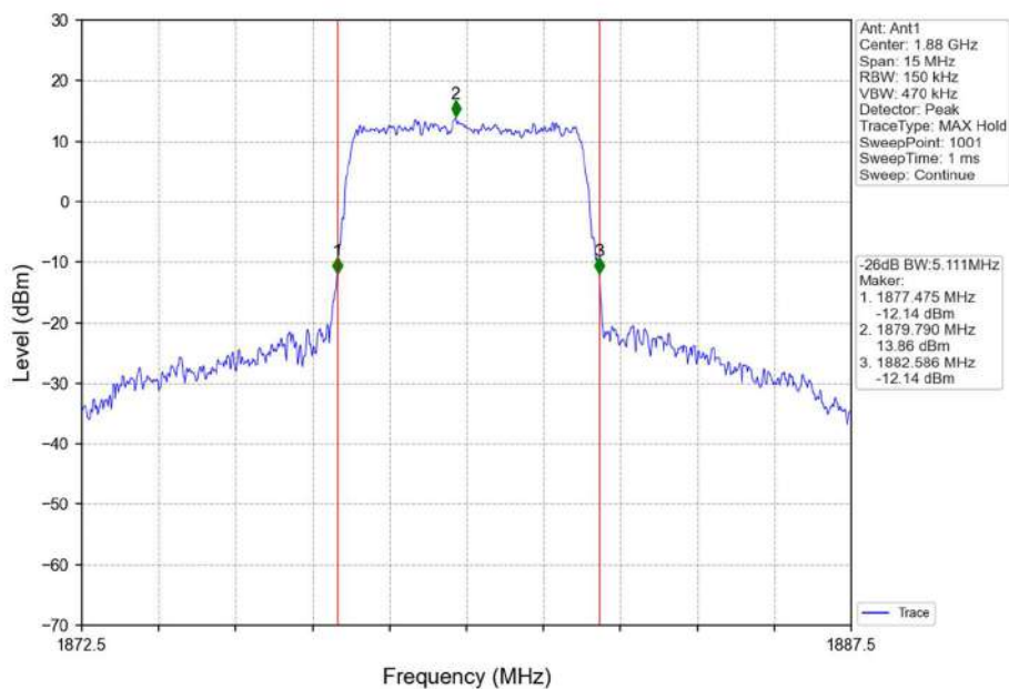
Band2_5MHz_16QAM_MCH_1880MHz_RB_25_0_NTNV
