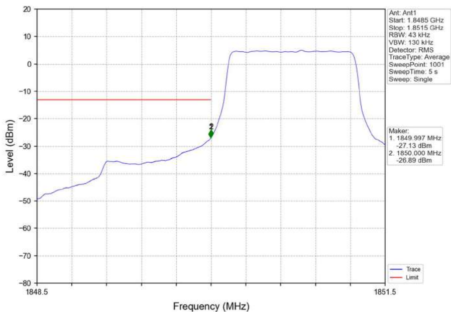
Band2_1.4MHz_QPSK_LCH_1850.7MHz_RB_6_0_NTNV
