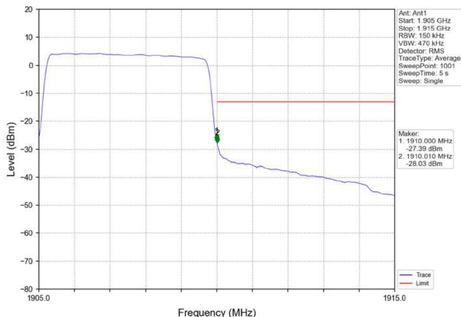
Band2_5MHz_16QAM_HCH_1907.5MHz_RB_25_0_NTNV
