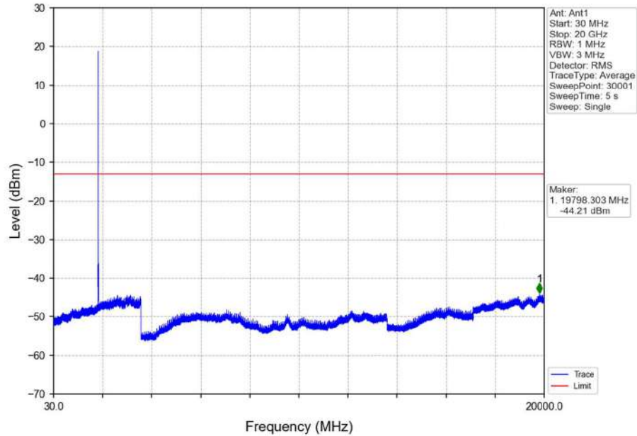
Band2_5MHz_QPSK_LCH_1852.5MHz_RB_1_0_NTNV
