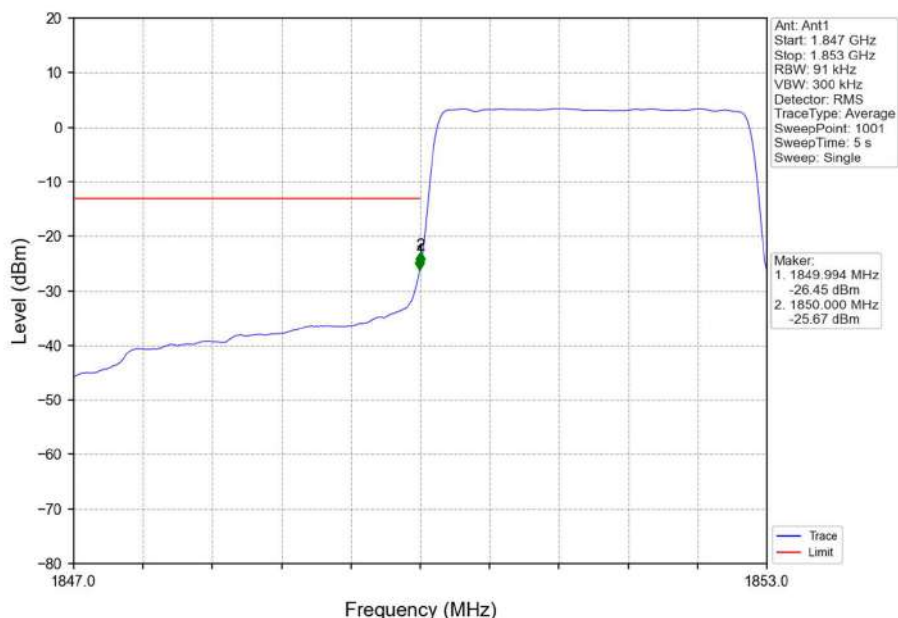
Band2_3MHz_16QAM_LCH_1851.5MHz_RB_15_0_NTNV
