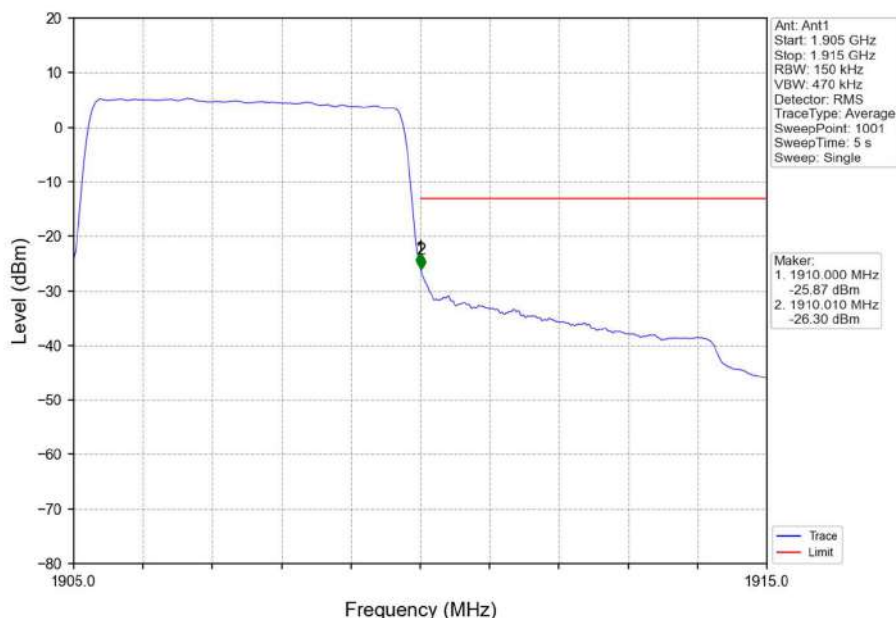
Band2_5MHz_QPSK_HCH_1907.5MHz_RB_25_0_NTNV
