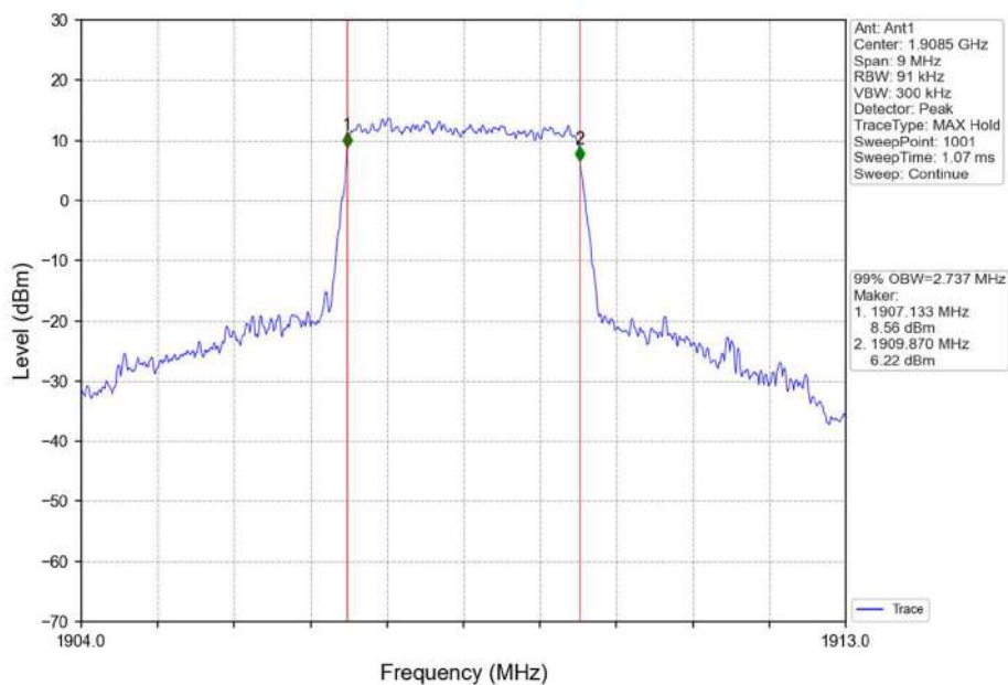
Band2_3MHz_16QAM_HCH_1908.5MHz_RB_15_0_NTNV
