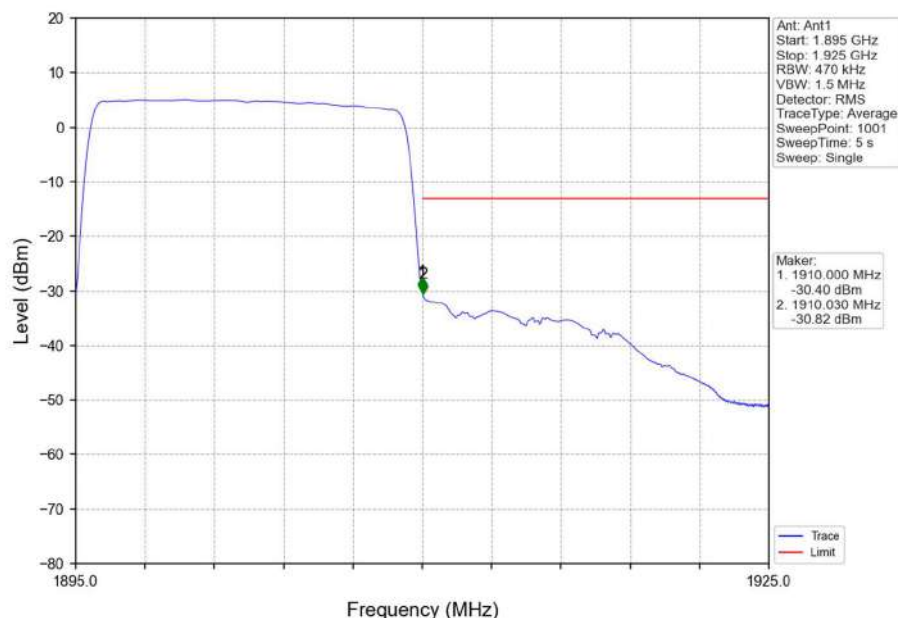
Band2_15MHz_QPSK_HCH_1902.5MHz_RB_75_0_NTNV
