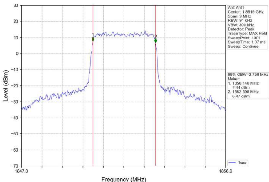
Band2_3MHz_16QAM_LCH_1851.5MHz_RB_15_0_NTNV
