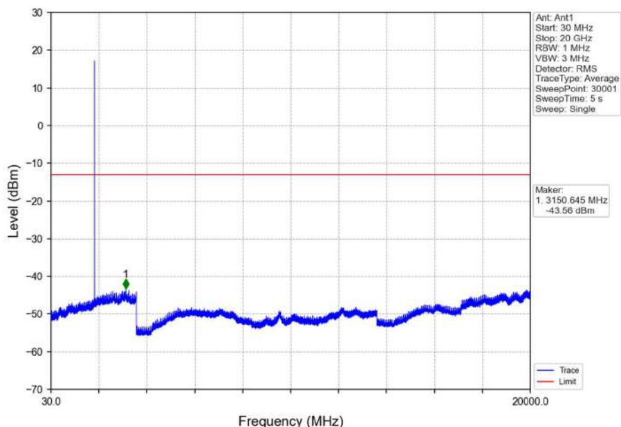
Band2_1.4MHz_16QAM_LCH_1850.7MHz_RB_1_0_NTNV
