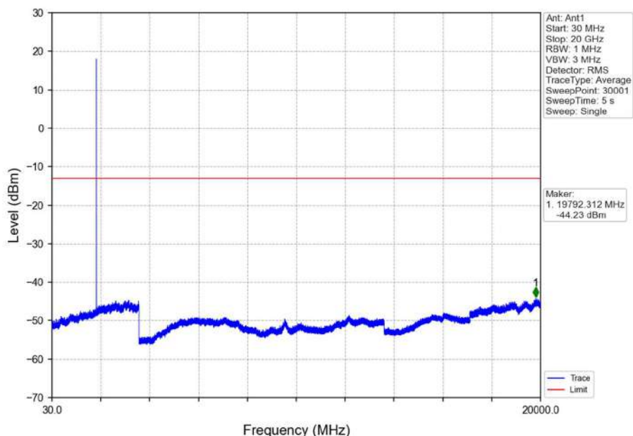
Band2_1.4MHz_QPSK_LCH_1850.7MHz_RB_1_0_NTNV
