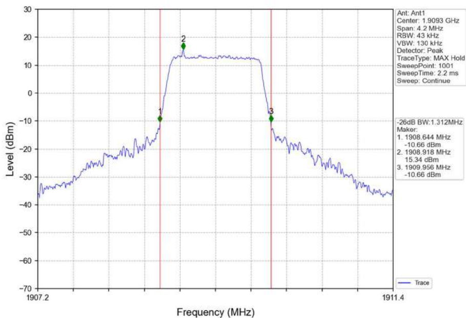
Band2_1.4MHz_16QAM_HCH_1909.3MHz_RB_6_0_NTNV
