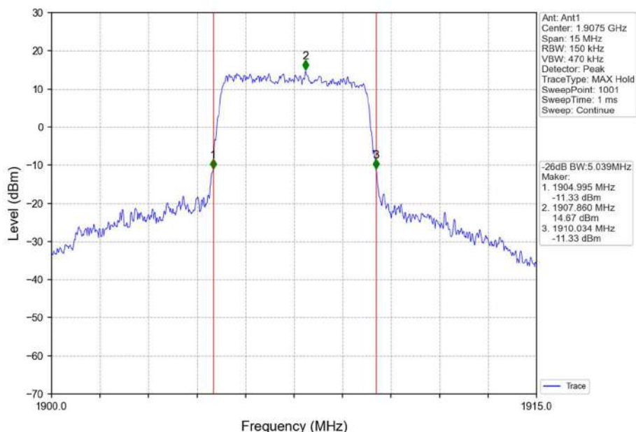
Band2_5MHz_16QAM_HCH_1907.5MHz_RB_25_0_NTNV
