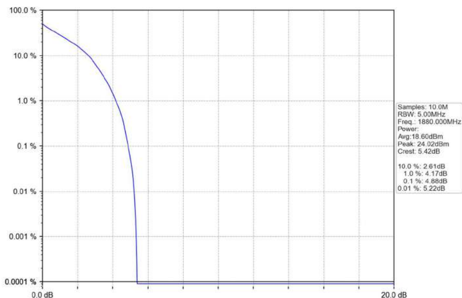
Band2_1.4MHz_QPSK_MCH_1880MHz_RB_6_0_NTNV
