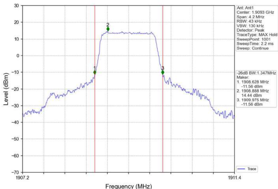
Band2_1.4MHz_QPSK_HCH_1909.3MHz_RB_6_0_NTNV
