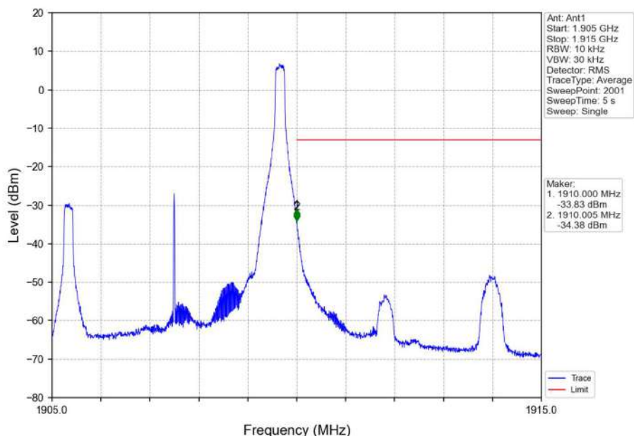
Band2_5MHz_16QAM_HCH_1907.5MHz_RB_1_24_NTNV
