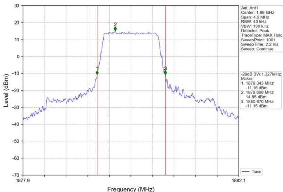
Band2_1.4MHz_QPSK_MCH_1880MHz_RB_6_0_NTNV
