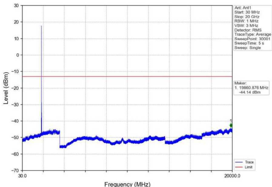
Band2_15MHz_16QAM_LCH_1857.5MHz_RB_1_0_NTNV
