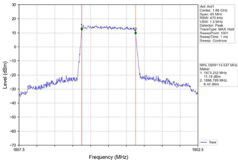
Band2_15MHz_QPSK_MCH_1880MHz_RB_75_0_NTNV
