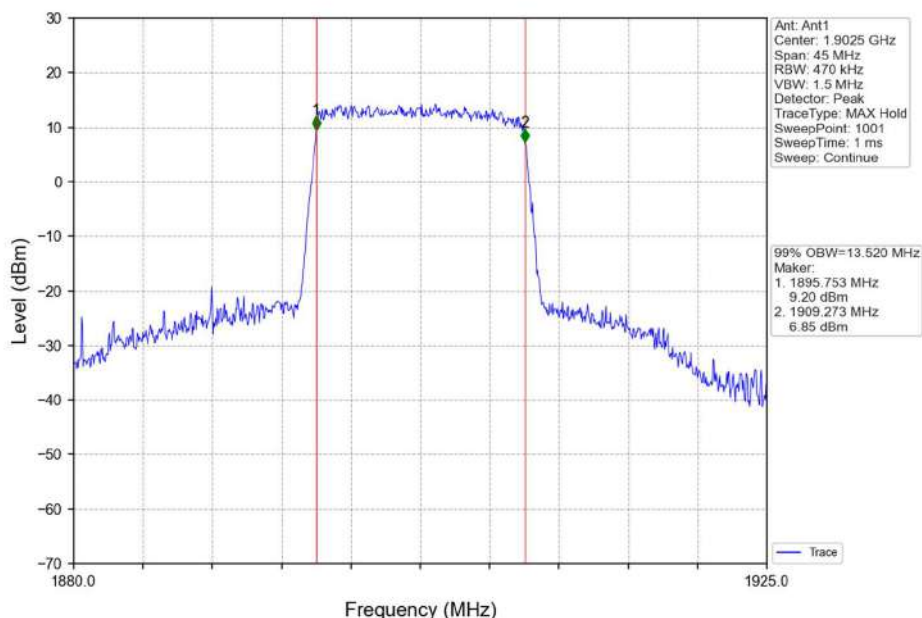
Band2_15MHz_16QAM_HCH_1902.5MHz_RB_75_0_NTNV
