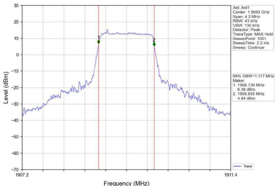
Band2_1.4MHz_16QAM_HCH_1909.3MHz_RB_6_0_NTNV
