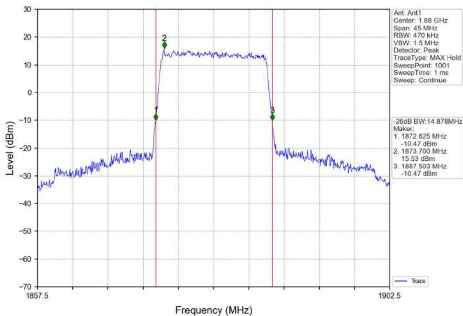
Band2_15MHz_QPSK_MCH_1880MHz_RB_75_0_NTNV
