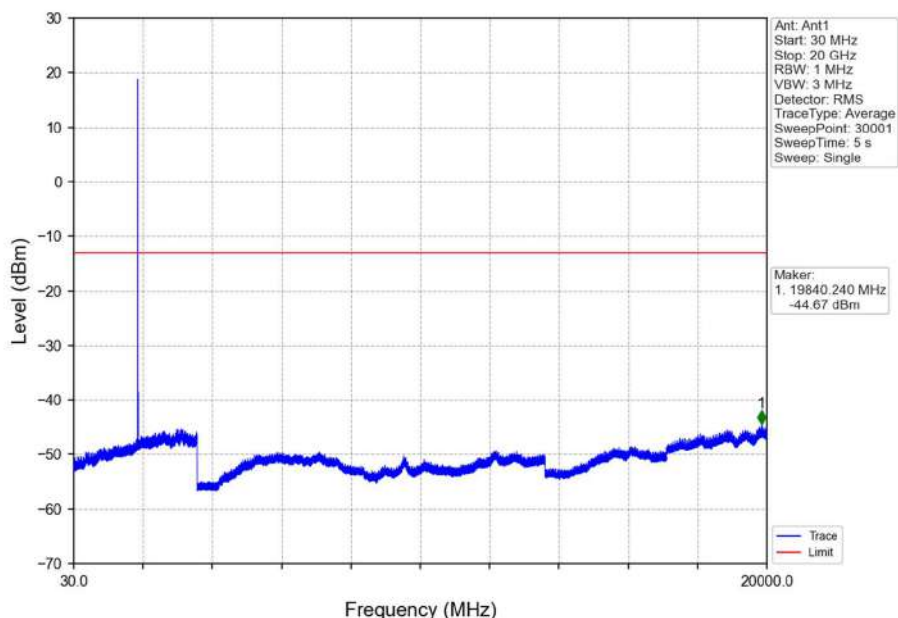
Band2_5MHz_16QAM_MCH_1880MHz_RB_1_0_NTNV
