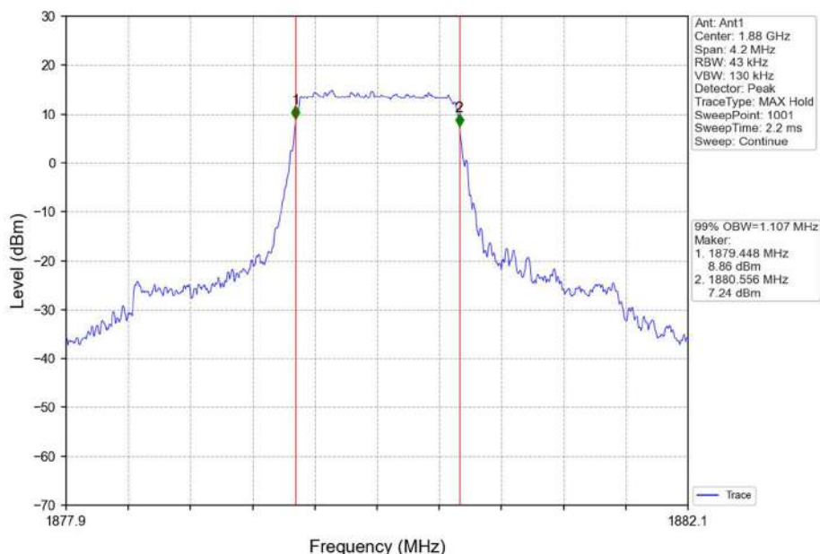
Band2_1.4MHz_QPSK_MCH_1880MHz_RB_6_0_NTNV
