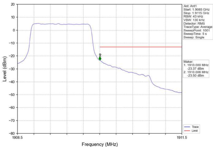
Band2_1.4MHz_QPSK_HCH_1909.3MHz_RB_6_0_NTNV
