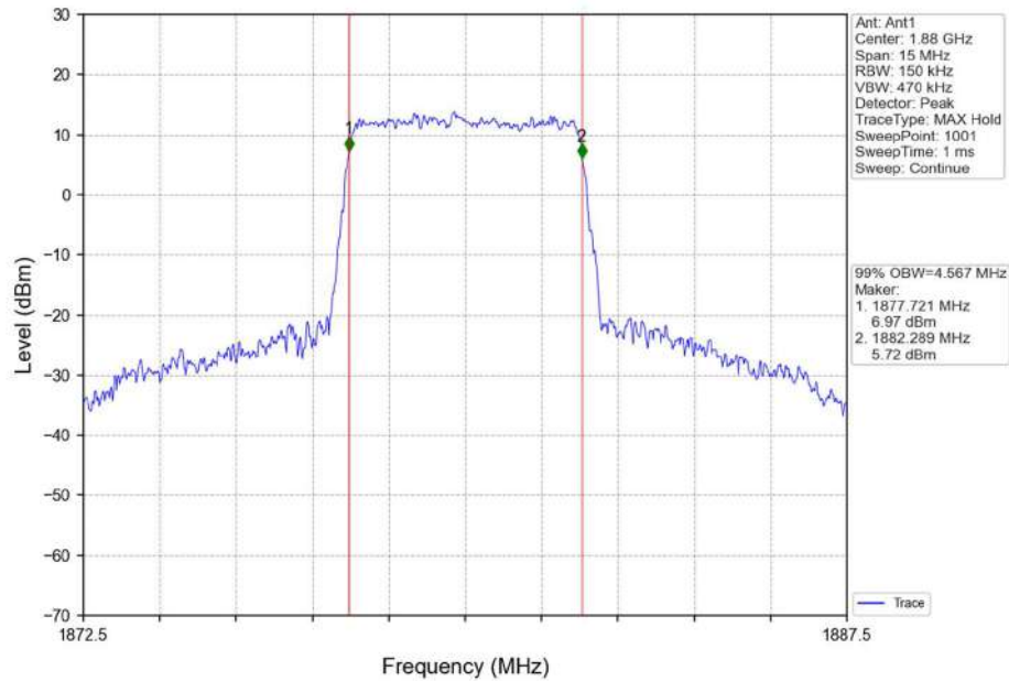
Band2_5MHz_16QAM_MCH_1880MHz_RB_25_0_NTNV
