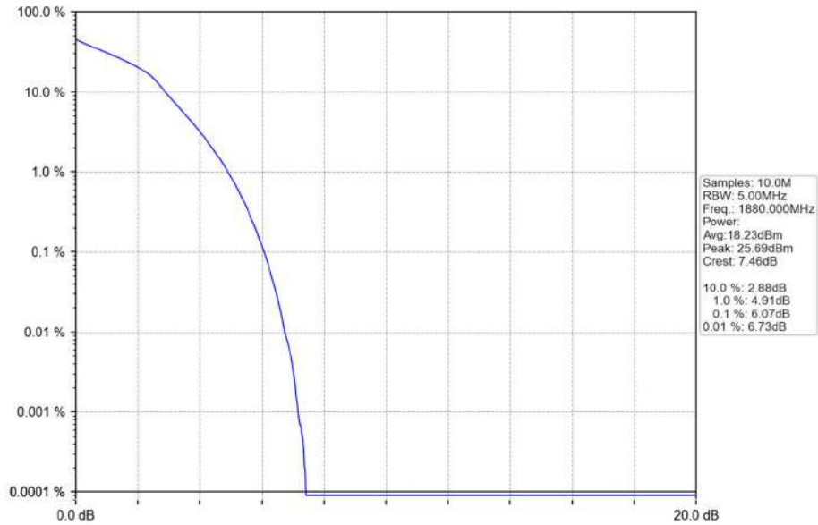
Band2_5MHz_16QAM_MCH_1880MHz_RB_25_0_NTNV
