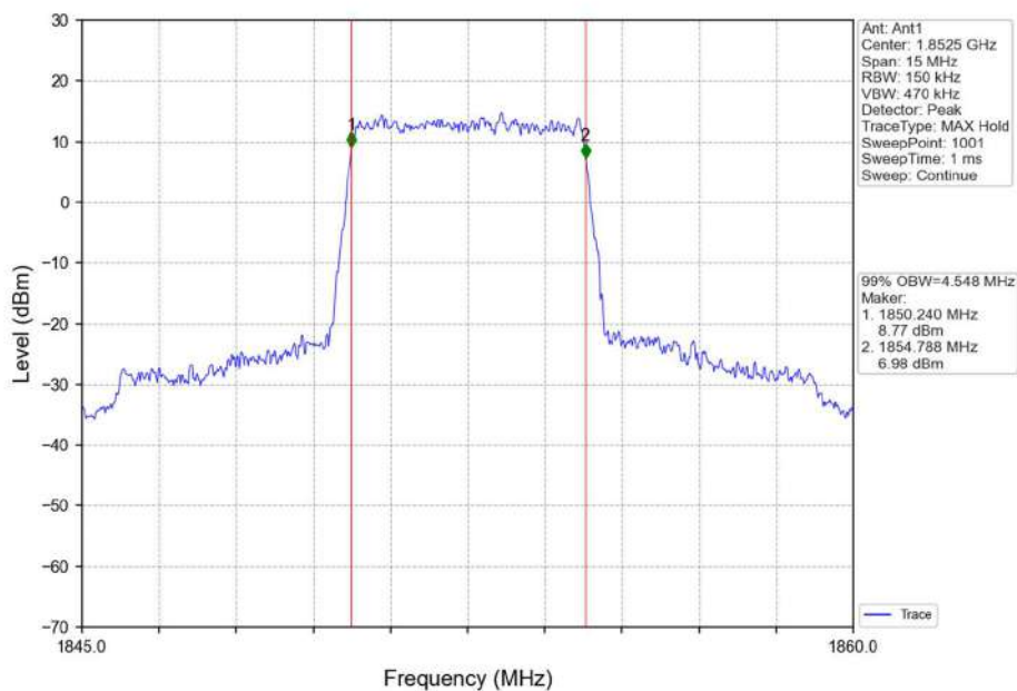
Band2_5MHz_QPSK_LCH_1852.5MHz_RB_25_0_NTNV
