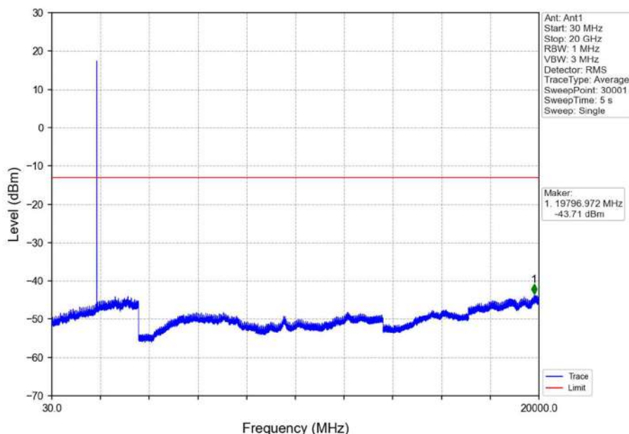
Band2_1.4MHz_16QAM_MCH_1880MHz_RB_1_0_NTNV
