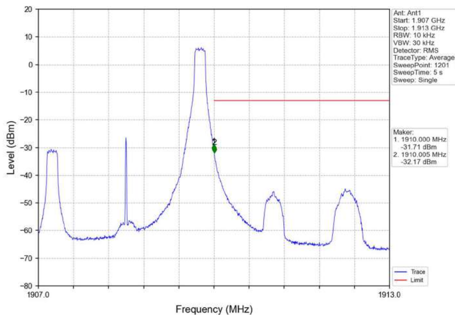
Band2_3MHz_16QAM_HCH_1908.5MHz_RB_1_14_NTNV
