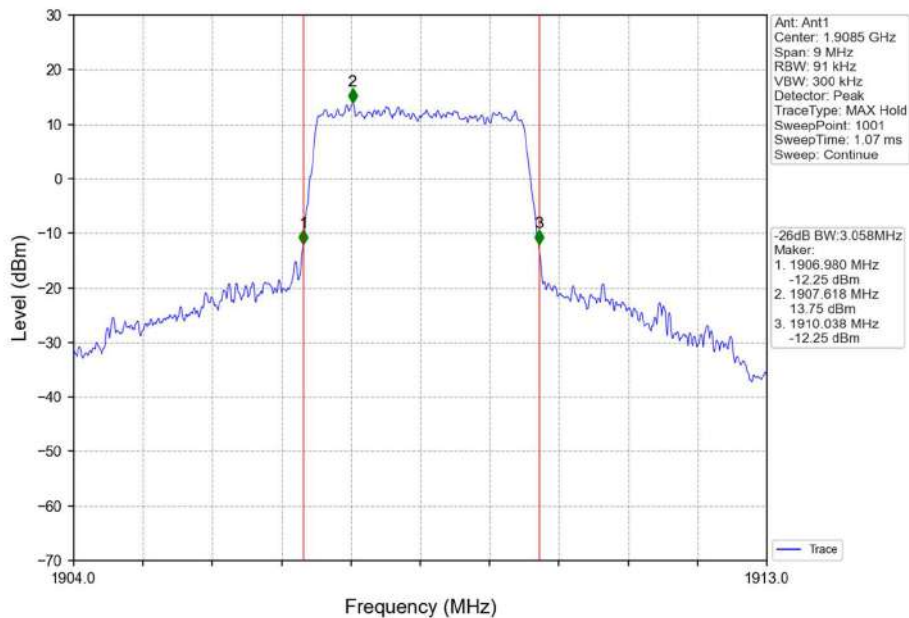
Band2_3MHz_16QAM_HCH_1908.5MHz_RB_15_0_NTNV
