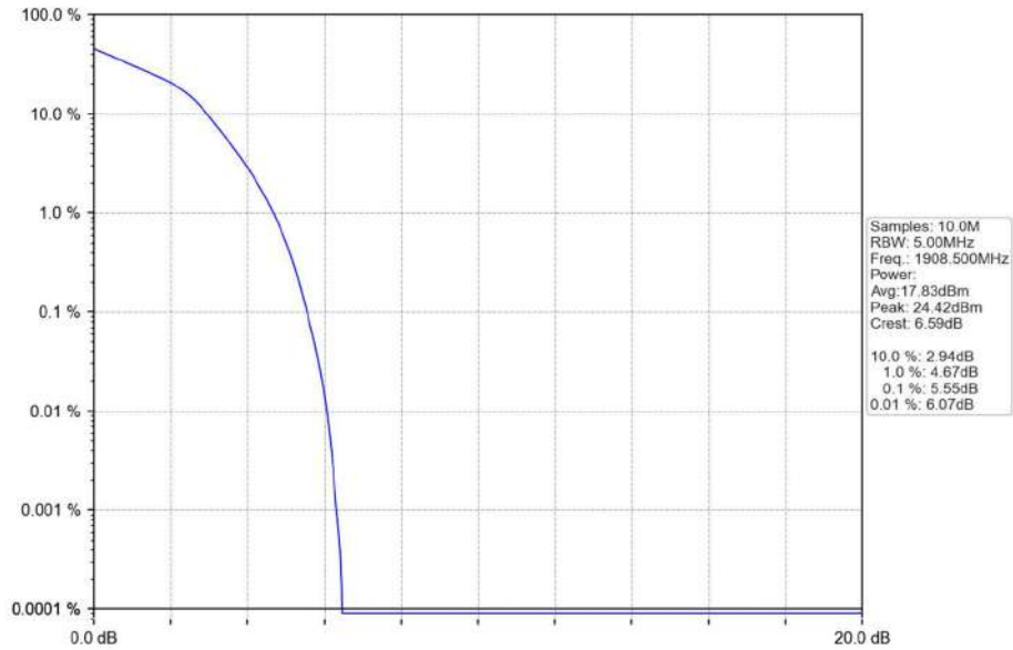
Band2_3MHz_16QAM_HCH_1908.5MHz_RB_15_0_NTNV
