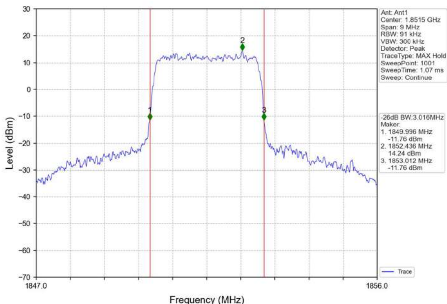
Band2_3MHz_16QAM_LCH_1851.5MHz_RB_15_0_NTNV
