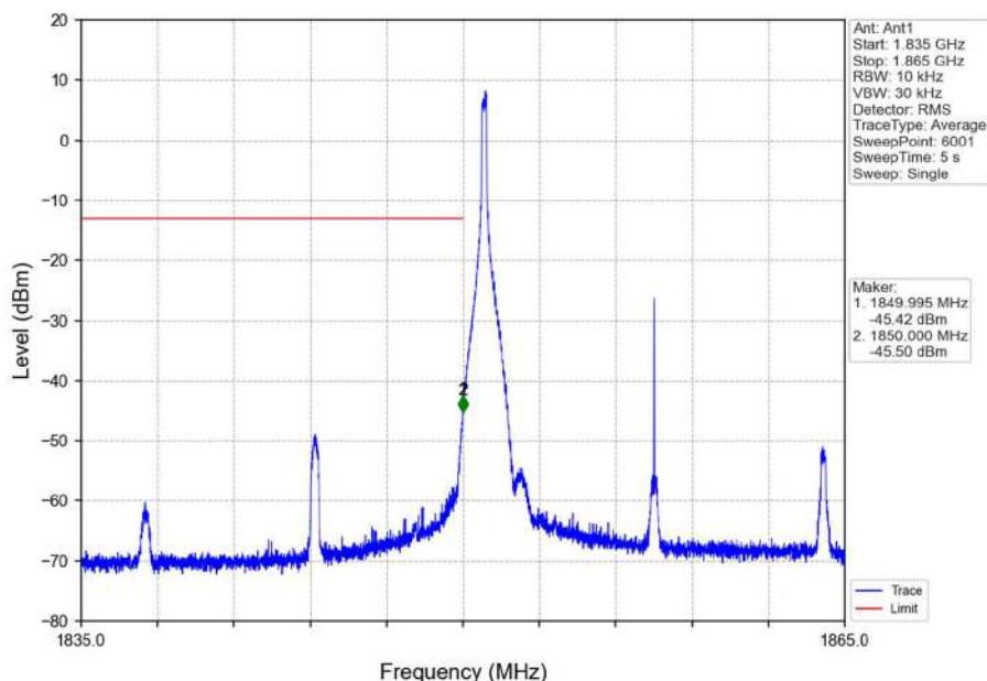
Band2_15MHz_16QAM_LCH_1857.5MHz_RB_1_0_NTNV
