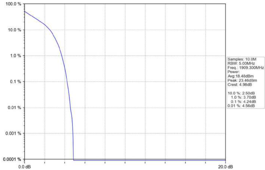
Band2_1.4MHz_QPSK_HCH_1909.3MHz_RB_6_0_NTNV
