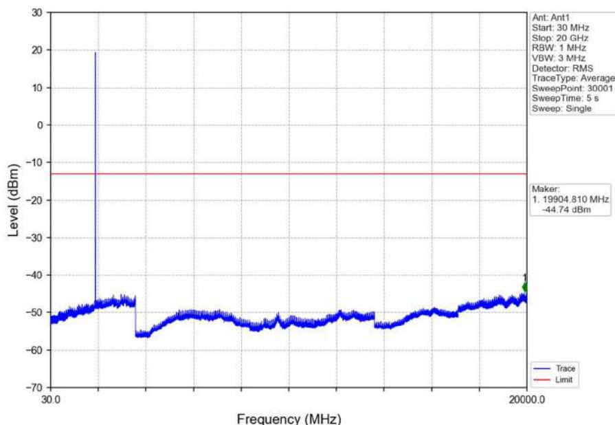
Band2_5MHz_QPSK_HCH_1907.5MHz_RB_1_0_NTNV
