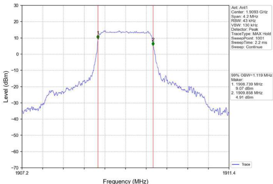
Band2_1.4MHz_QPSK_HCH_1909.3MHz_RB_6_0_NTNV
