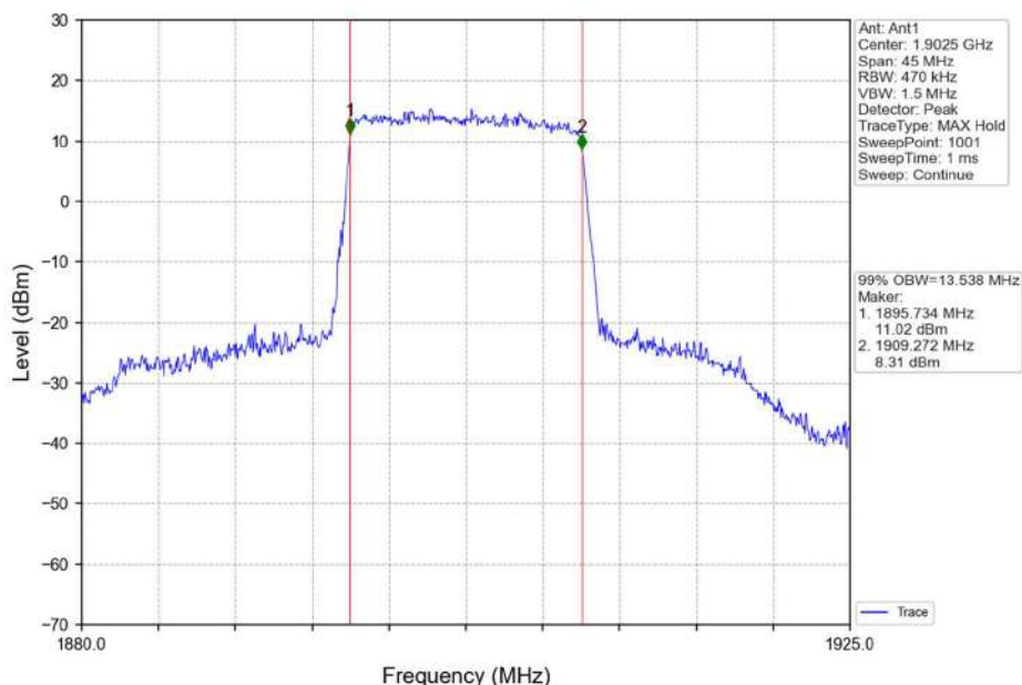
Band2_15MHz_QPSK_HCH_1902.5MHz_RB_75_0_NTNV
