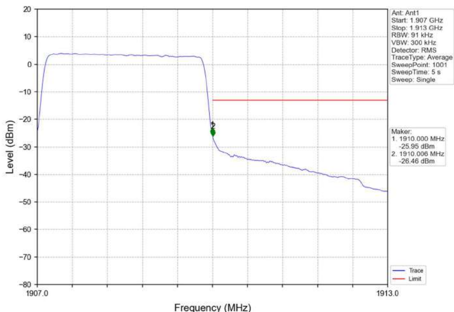
Band2_3MHz_16QAM_HCH_1908.5MHz_RB_15_0_NTNV
