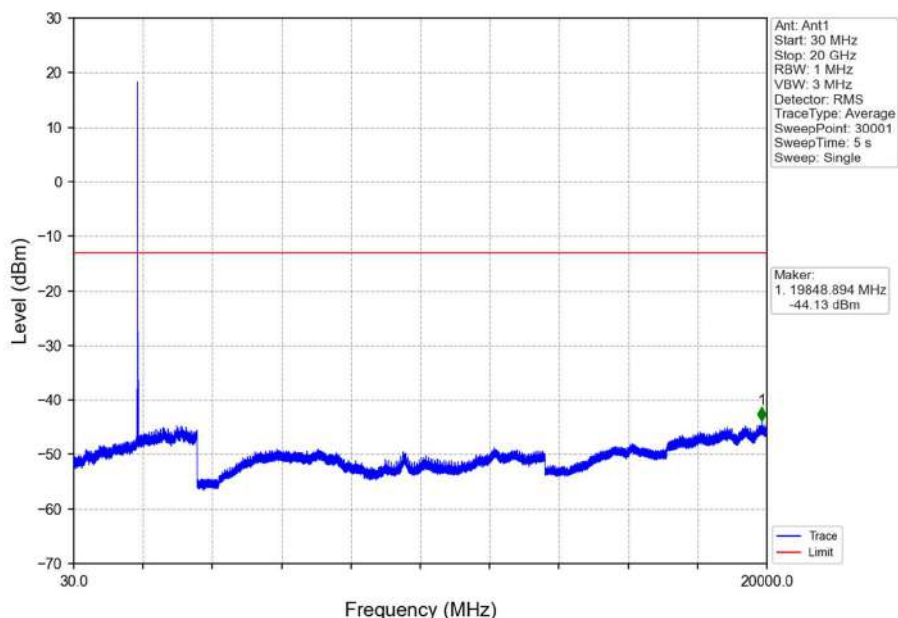
Band2_15MHz_16QAM_MCH_1880MHz_RB_1_0_NTNV
