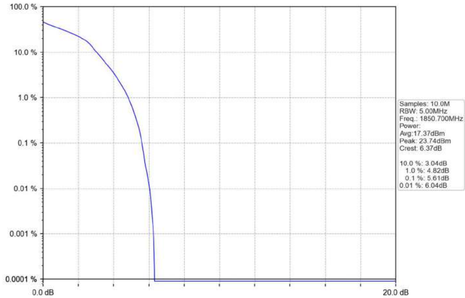
Band2_1.4MHz_16QAM_LCH_1850.7MHz_RB_6_0_NTNV
