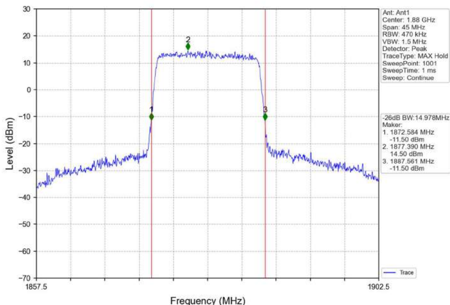
Band2_15MHz_16QAM_MCH_1880MHz_RB_75_0_NTNV
