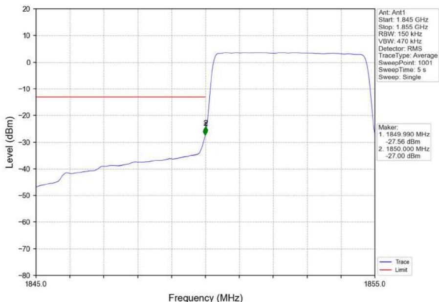
Band2_5MHz_16QAM_LCH_1852.5MHz_RB_25_0_NTNV
