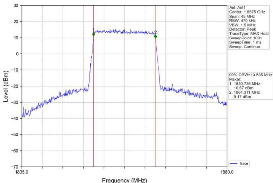
Band2_15MHz_QPSK_LCH_1857.5MHz_RB_75_0_NTNV
