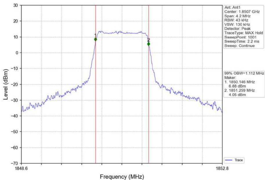
Band2_1.4MHz_16QAM_LCH_1850.7MHz_RB_6_0_NTNV
