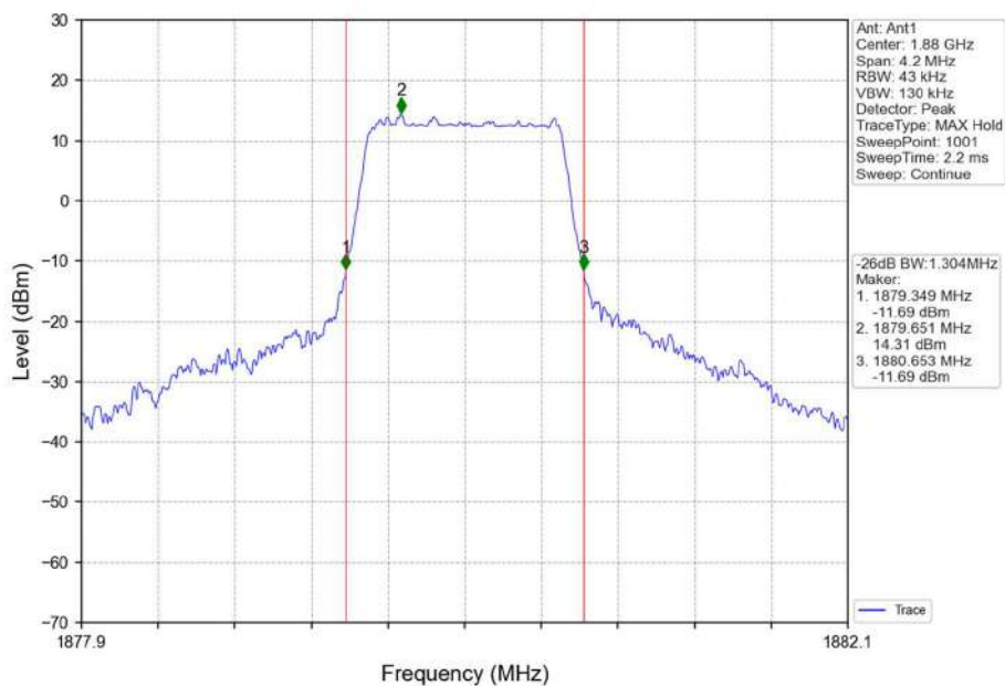
Band2_1.4MHz_16QAM_MCH_1880MHz_RB_6_0_NTNV
