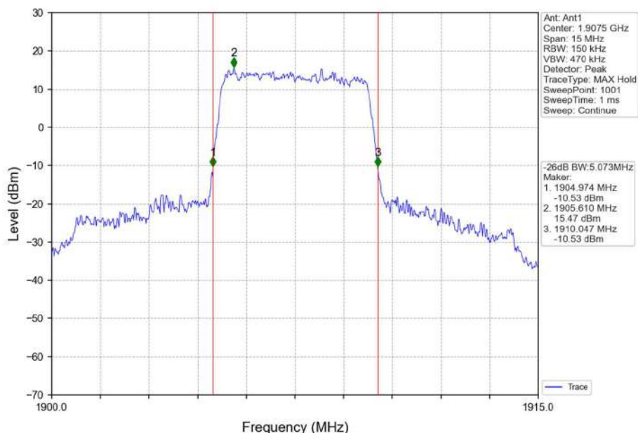
Band2_5MHz_QPSK_HCH_1907.5MHz_RB_25_0_NTNV
