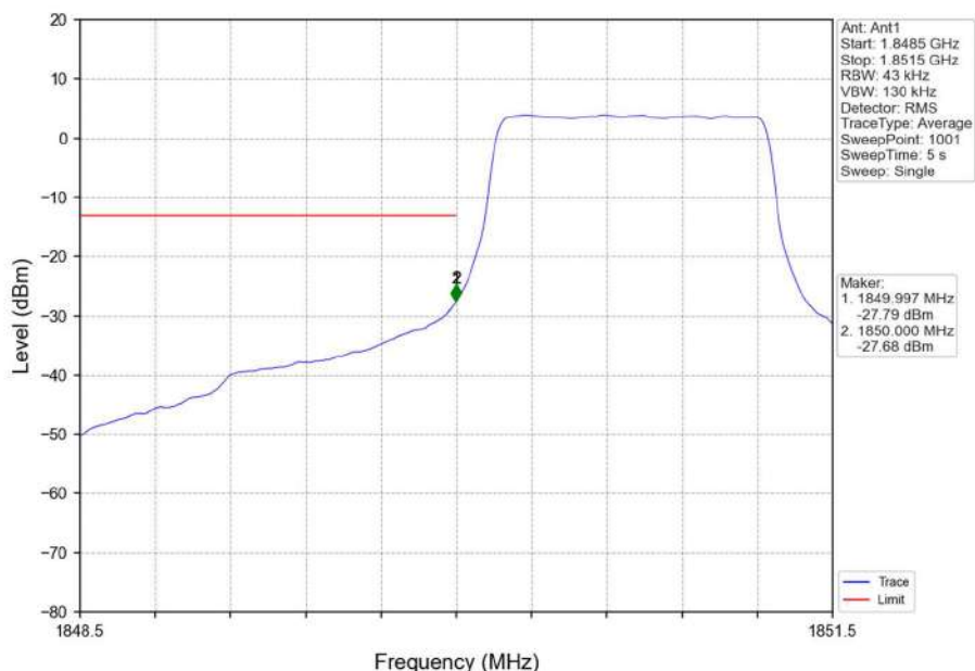
Band2_1.4MHz_16QAM_LCH_1850.7MHz_RB_6_0_NTNV
