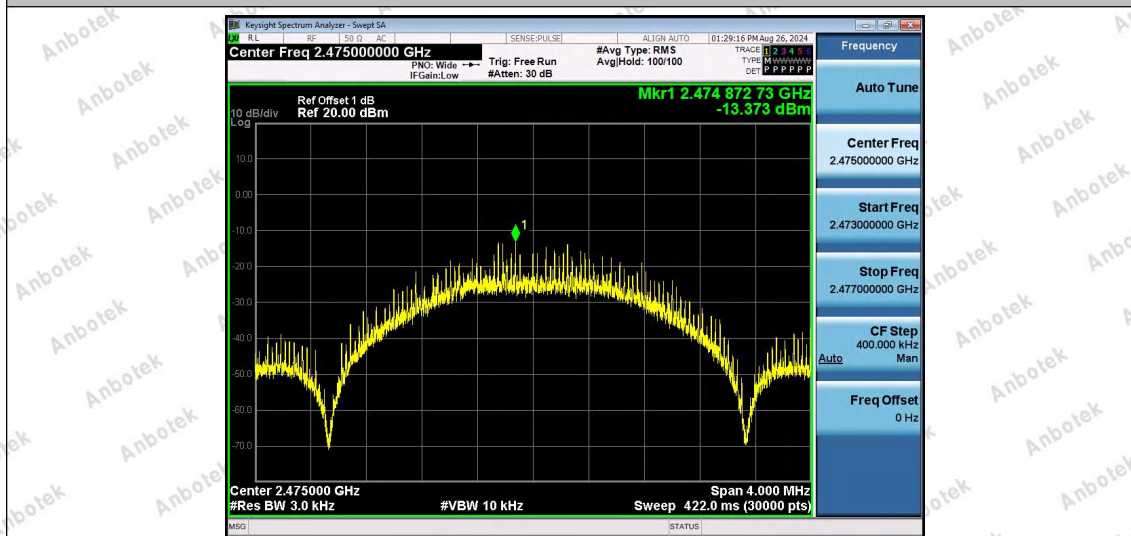
2.4G-Ant1-2475-PASS
