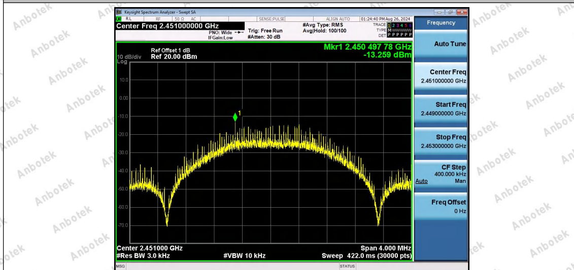
2.4G-Ant1-2451-PASS
