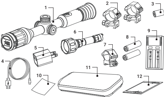
FIGURE 1-2. STANDARD COMPONENTS
