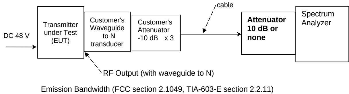
Measurement Block Diagram
