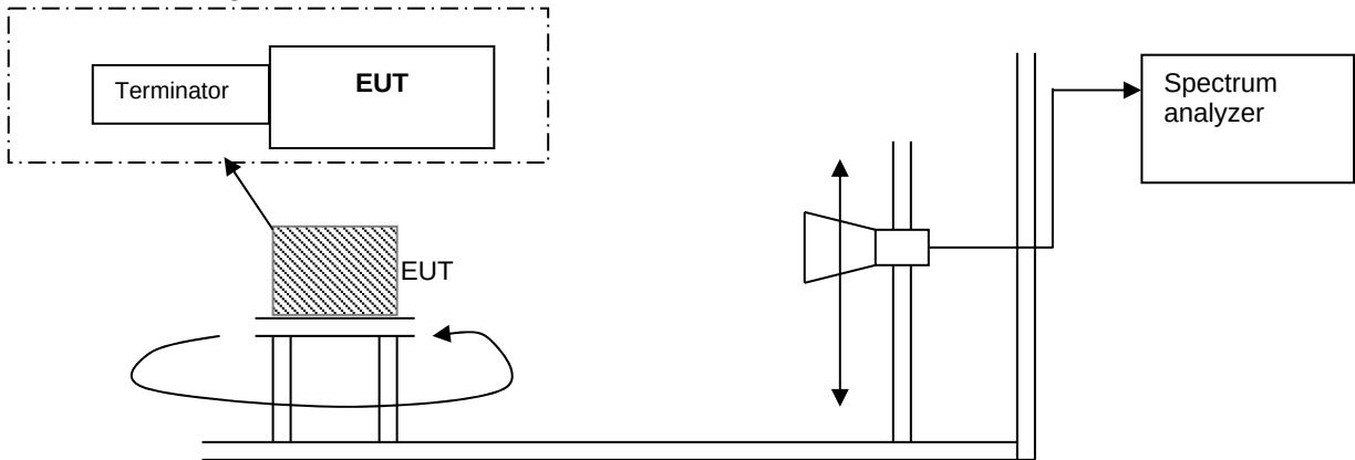
Field Strength of Spurious Emission (FCC section 2.1053, TIA-603-E section 2.2.12)
