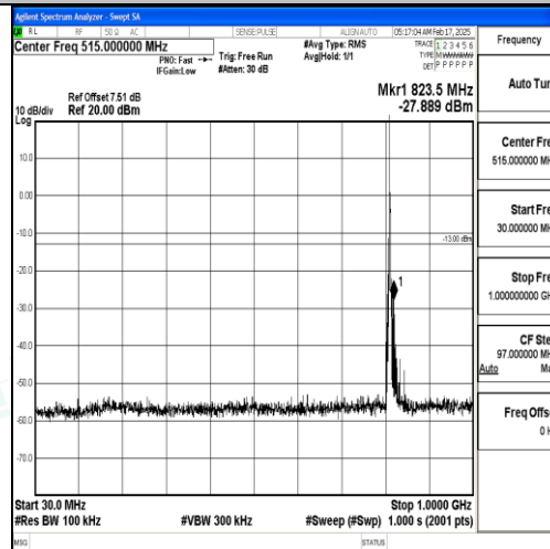
Band26_3MHz_16QAM_26705_1RB#0_30~1000_30~1000
