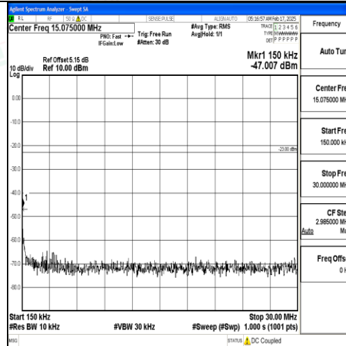
Band26_3MHz_16QAM_26705_1RB#0_0.15~30_0.15~30
