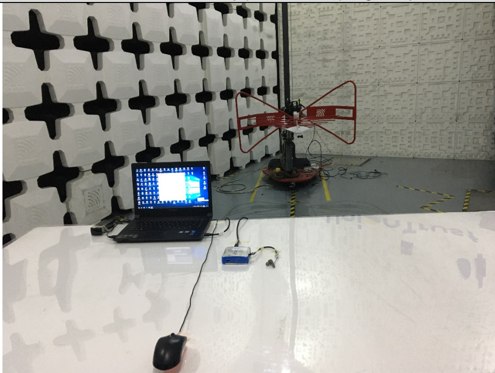
Radiated emission Test Setup (30 MHz~1 GHz)- Left earphone
