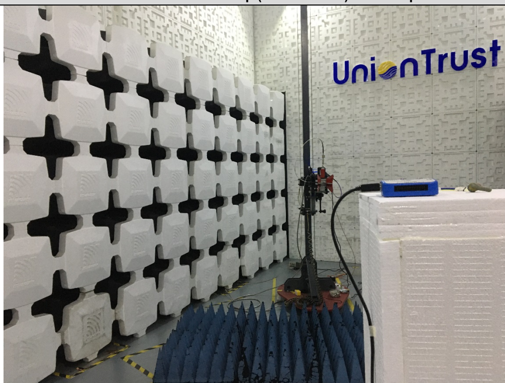
Radiated emission Test Setup (Above 1 GHz) - Left earphone
