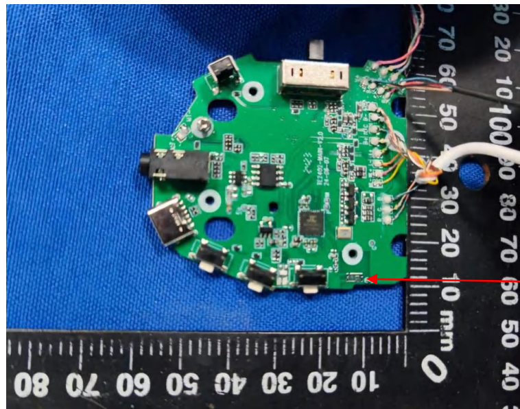
BT Antenna
